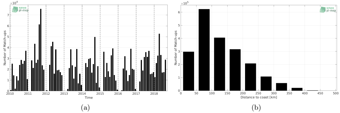
Figure 1: Number of match-ups between TSG-SAMOS and SMOS-L3-CATDS-CPDC-V3-MONTHLY-25KM SSS as a function of time (a) and as function of the distance to coast (b) over the Mississippi river plume Pi-MEP region and for the full satellite product period.
