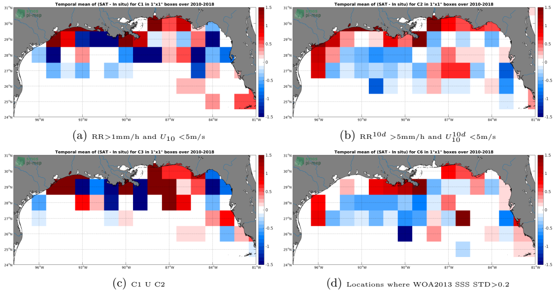
Figure 12: Temporal mean gridded over spatial boxes of size 1^\circ \times 1^\circ of \Delta SSS (SMOS-L3-CATDS-CPDC-V3-MONTHLY-25KM - TSG-SAMOS) for 4 different subdatasets corresponding to:RR >1 mm/h and U_{10} < 5 m/s (a), RR 10d > 5 mm/h and U_{10}^{10d} < 5 m/s (b), C1 U C2 (c),Locations where WOA2013 SSS STD >0.2 (d).
