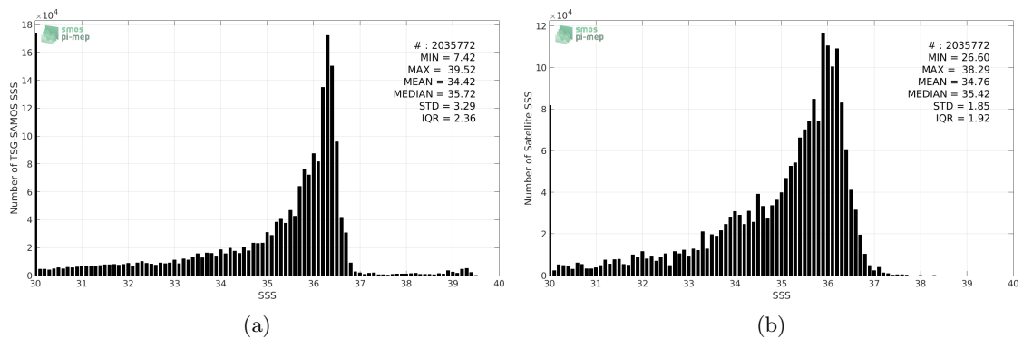
Figure 2: Histograms of SSS from TSG-SAMOS (a) and SMOS-L3-CATDS-CPDC-V3-MONTHLY-25KM (b) considering all match-up pairs per bins of 0.1 over the Mississippi river plume Pi-MEP region and for the full satellite product period.
