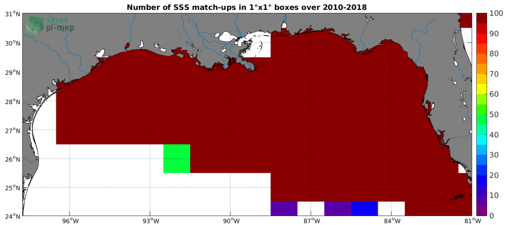
Figure 4: Number of SSS match-ups between TSG-SAMOS SSS and the SMOS-L3-CATDS-CPDC-V3-MONTHLY-25KM SSS product for the Mississippi river plume Pi-MEP region over 1^\circ \times 1^\circ boxes and for the full satellite product period.
