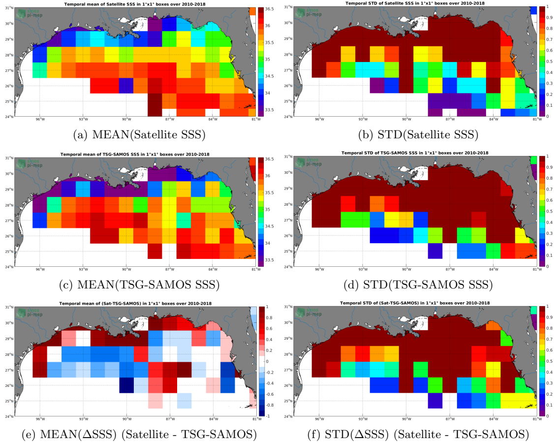
Figure 6: Temporal mean (left) and STD (right) of SSS from SMOS-L3-CATDS-CPDC-V3-MONTHLY-25KM (top), TSG-SAMOS (middle), and of \Delta SSS (Satellite - TSG-SAMOS). Only match-up pairs are used to generate these maps.
