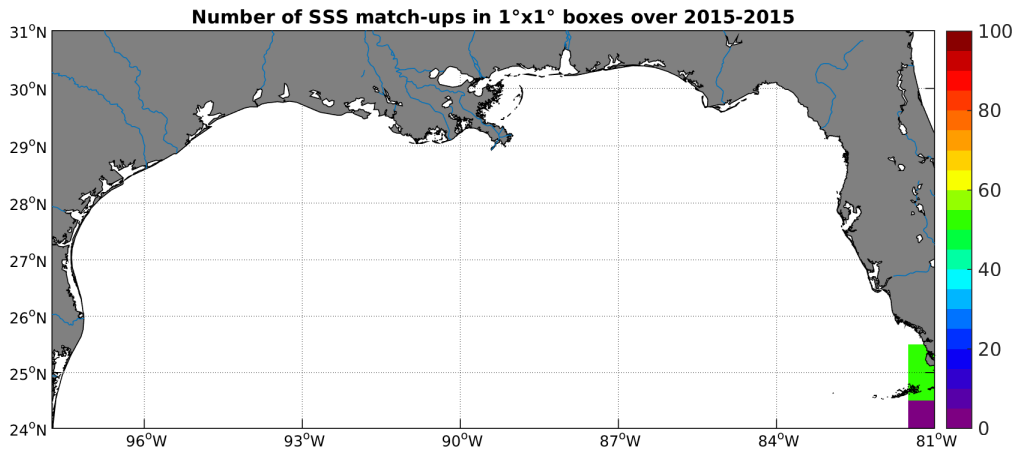
Figure 4: Number of SSS match-ups between TSG-GOSUD-Sailing-ship SSS and the SMOS-L3-CATDS-CPDC-V3-MONTHLY-25KM SSS product for the Mississippi river plume Pi-MEP region over 1^{\circ} \times 1^{\circ} boxes and for the full satellite product period.
