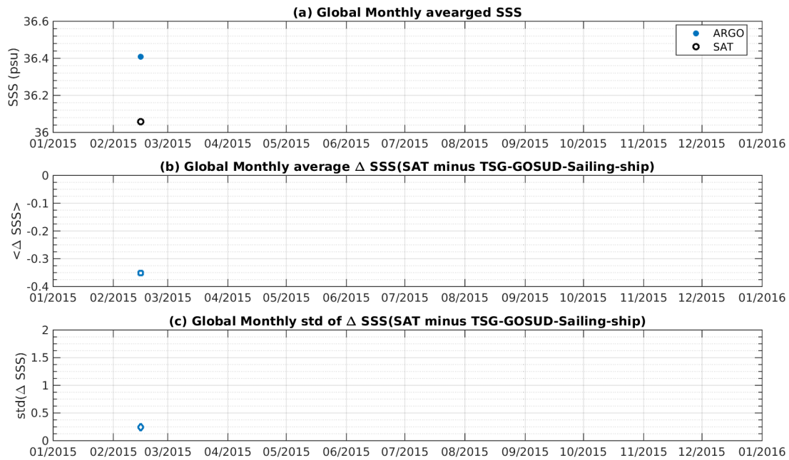
Figure 7: Time series of the monthly averaged mean SSS (top), mean \Delta SSS (Satellite - TSG-GOSUD-Sailing-ship) and STD of \Delta SSS (Satellite - TSG-GOSUD-Sailing-ship) over the Mississippi river plume Pi-MEP region considering all match-ups collected by the Pi-MEP platform.
