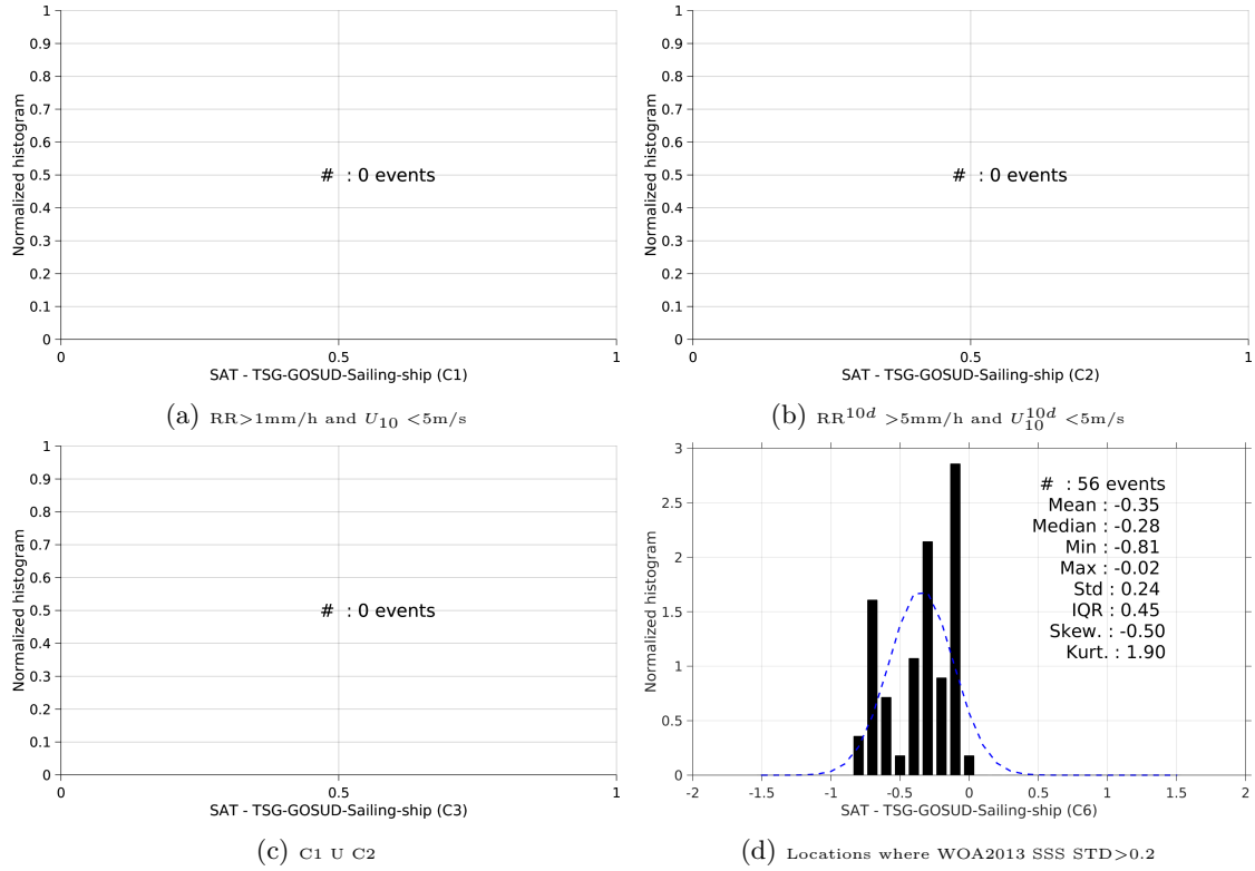
Figure 13: Normalized histogram of \Delta\text{SSS} (SMOS-L3-CATDS-CPDC-V3-MONTHLY-25KM - TSG-GOSUD-Sailing-ship) for 6 different subdatasets corresponding to: RR > 1\text{mm/h} and U_{10} < 5\text{m/s} (a), RR^{10d} > 5\text{mm/h} and U_{10}^{10d} < 5\text{m/s} (b), C1 U C2 (c), Locations where WOA2013 SSS STD > 0.2 (d).
