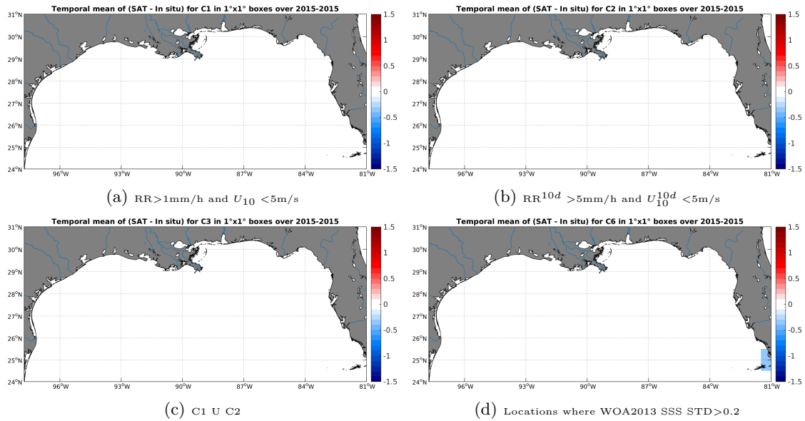
Figure 12: Temporal mean gridded over spatial boxes of size 1^\circ \times 1^\circ of \Delta SSS (SMOS-L3-CATDS-CPDC-V3-MONTHLY-25KM - TSG-GOSUD-Sailing-ship) for 4 different subdatasets corresponding to:RR >1 mm/h and U_{10} < 5 m/s (a), RR ^{10d} > 5 mm/h and U_{10}^{10d} < 5 m/s (b), C1 U C2 (c),Locations where WOA2013 SSS STD >0.2 (d).
