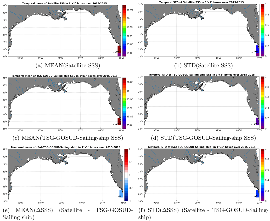
Figure 6: Temporal mean (left) and STD (right) of SSS from SMOS-L3-CATDS-CPDC-V3-MONTHLY-25KM (top), TSG-GOSUD-Sailing-ship (middle), and of \Delta SSS (Satellite - TSG-GOSUD-Sailing-ship). Only match-up pairs are used to generate these maps.
