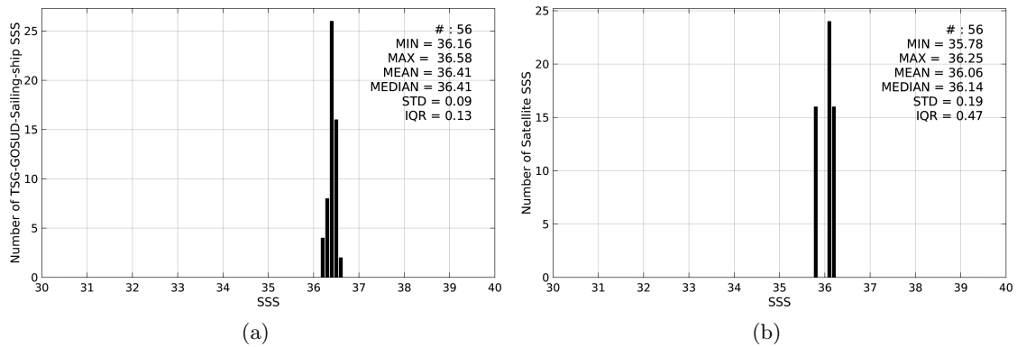
Figure 2: Histograms of SSS from TSG-GOSUD-Sailing-ship (a) and SMOS-L3-CATDS-CPDC-V3-MONTHLY-25KM (b) considering all match-up pairs per bins of 0.1 over the Mississippi river plume Pi-MEP region and for the full satellite product period.
