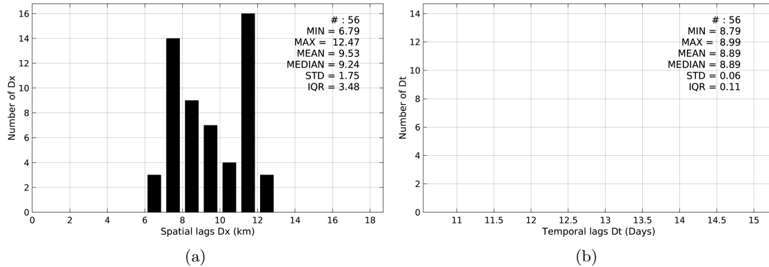
Figure 5: Histograms of the spatial (a) and temporal (b) lags between the time of the TSG-GOSUD-Sailing-ship measurements and the date of the corresponding SMOS-L3-CATDS-CPDC-V3-MONTHLY-25KM SSS product.
