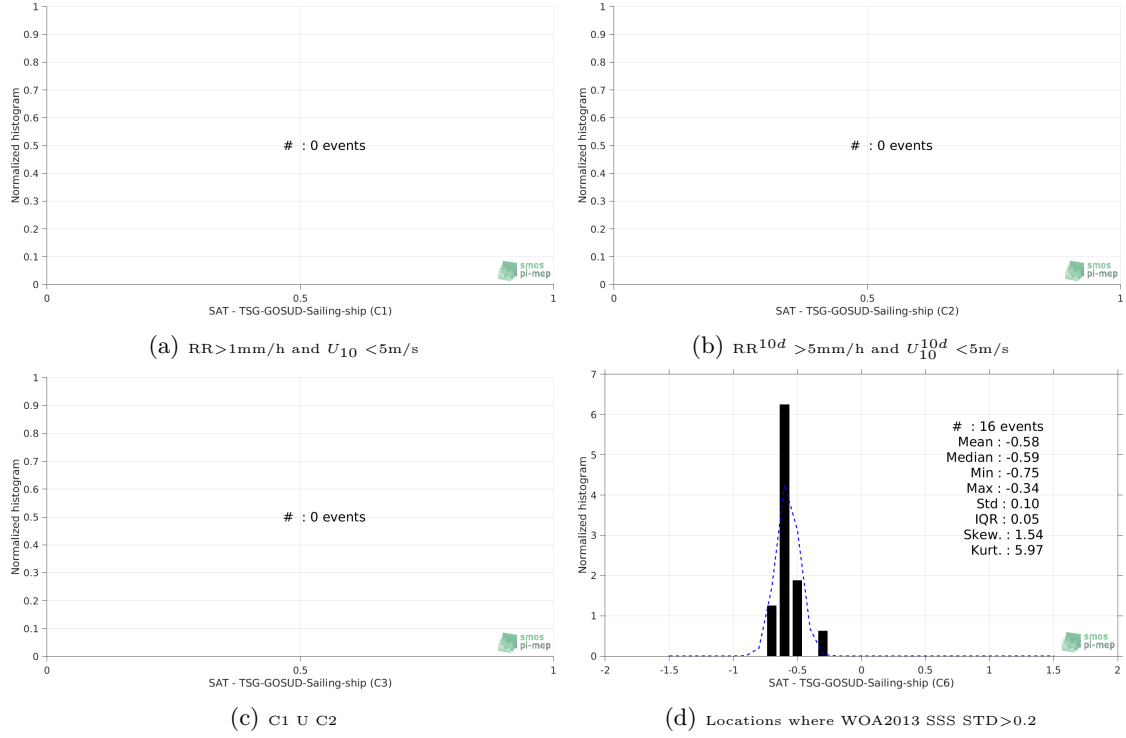
Figure 13: Normalized histogram of \Delta SSS (SMOS-L3-CATDS-CPDC-V3-10DAYS-25KM - TSG-GOSUD-Sailing-ship) for 6 different subdatasets corresponding to: RR > 1\text{mm/h} and U_{10} < 5\text{m/s} (a), RR^{10d} > 5\text{mm/h} and U_{10}^{10d} < 5\text{m/s} (b), C1 U C2 (c), Locations where WOA2013 SSS STD > 0.2 (d).
