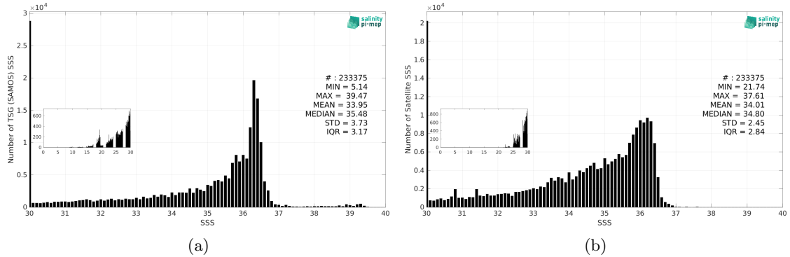
Figure 3: Histograms of SSS from TSG (SAMOS) (a) and SMOS SSS L3 v2 - 9-Days (BEC) (b) considering all match-up pairs per bins of 0.1 over the Mississippi river plume Pi-MEP region and for the full satellite product period.
