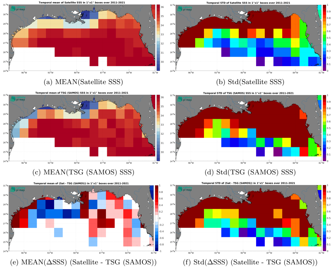
Figure 7: Temporal mean (left) and Std (right) of SSS from SMOS SSS L3 v2 - 9-Days (BEC) (top), TSG (SAMOS) (middle), and of \Delta\text{SSS} (Satellite - TSG (SAMOS)). Only match-up pairs are used to generate these maps.
