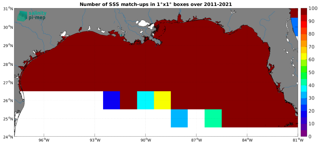
Figure 5: Number of SSS match-ups between TSG (SAMOS) SSS and the SMOS SSS L3 v2 - 9-Days (BEC) SSS product for the Mississippi river plume Pi-MEP region over 1^\circ \times 1^\circ boxes and for the full satellite product period.
