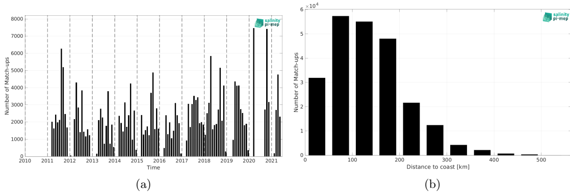
Figure 2: Number of match-ups between TSG (SAMOS) and SMOS SSS L3 v2 - 9-Days (BEC) SSS as a function of time (a) and as function of the distance to coast (b) over the Mississippi river plume Pi-MEP region and for the full satellite product period.
