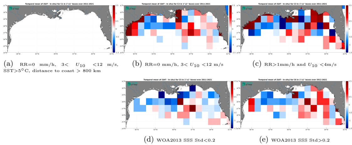
Figure 14: Temporal mean gridded over spatial boxes of size 1^\circ \times 1^\circ of \Delta SSS (SMOS SSS L3 v2 - 9-Days (BEC) - TSG (SAMOS)) for 5 different subdatasets corresponding to:RR=0 mm/h, 3 < U_{10} < 12 m/s, SST>5°C, distance to coast > 800 km (a), RR=0 mm/h, 3 < U_{10} < 12 m/s (b), RR>1mm/h and U_{10} < 4 m/s (c), WOA2013 SSS Std<0.2 (d), WOA2013 SSS Std>0.2 (e).
