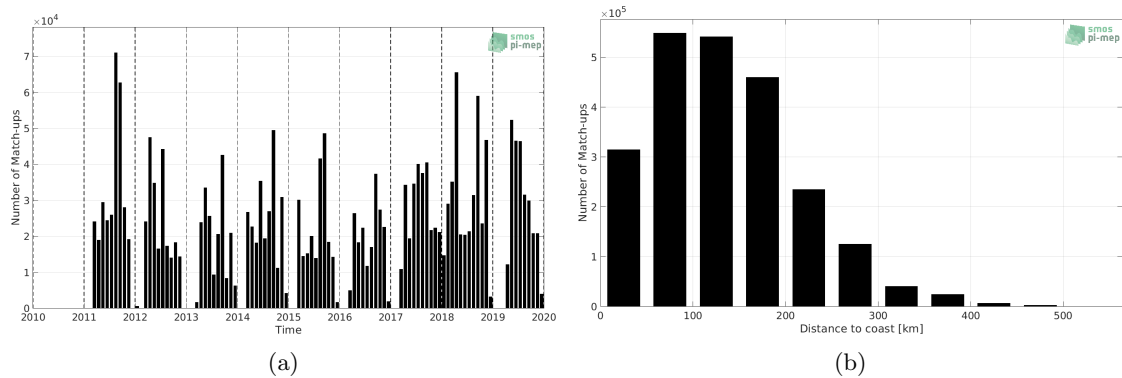
Figure 1: Number of match-ups between TSG (SAMOS) and SMOS SSS L3 v2 - 9-Days (BEC) SSS as a function of time (a) and as function of the distance to coast (b) over the Mississippi river plume Pi-MEP region and for the full satellite product period.
