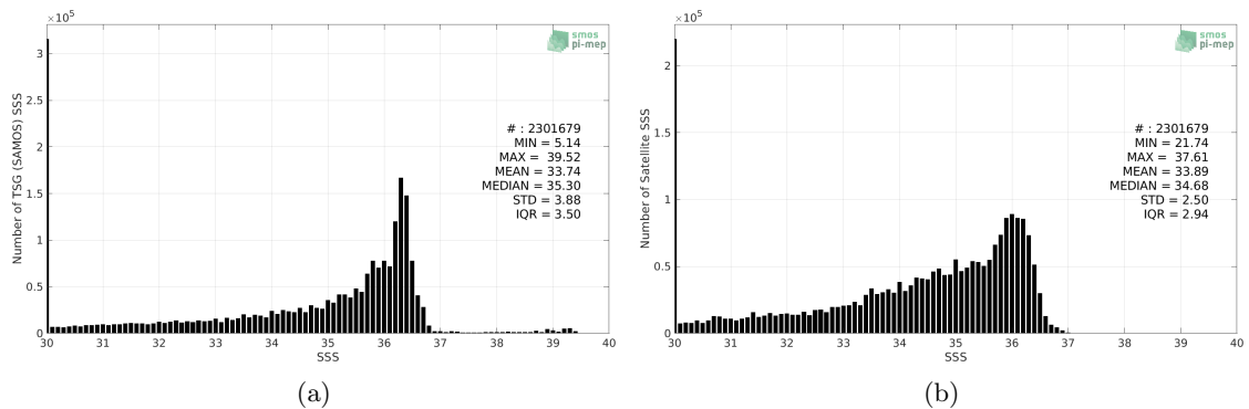
Figure 2: Histograms of SSS from TSG (SAMOS) (a) and SMOS SSS L3 v2 - 9-Days (BEC) (b) considering all match-up pairs per bins of 0.1 over the Mississippi river plume Pi-MEP region and for the full satellite product period.
