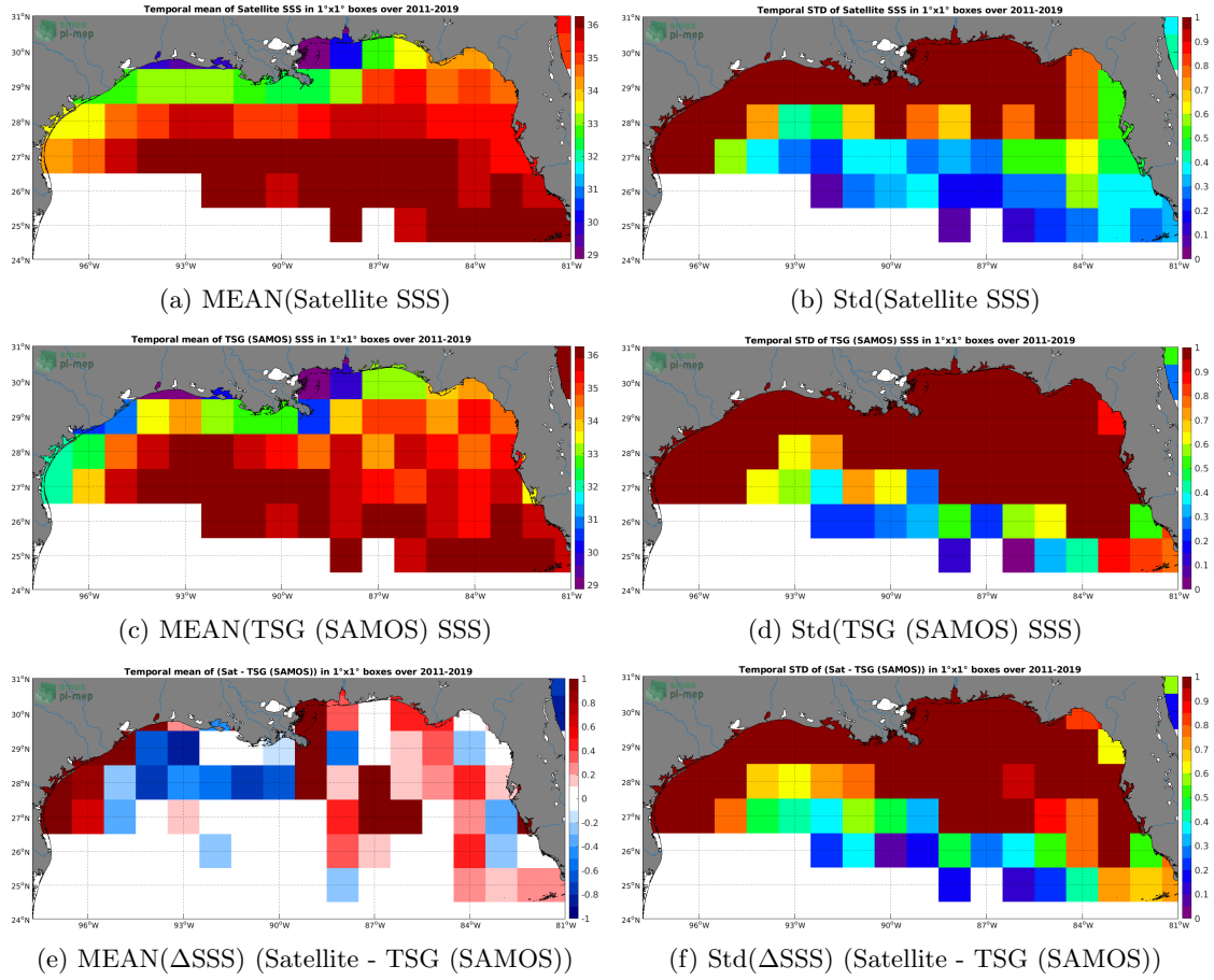
Figure 6: Temporal mean (left) and Std (right) of SSS from SMOS SSS L3 v2 - 9-Days (BEC) (top), TSG (SAMOS) (middle), and of \Delta SSS (Satellite - TSG (SAMOS)). Only match-up pairs are used to generate these maps.
