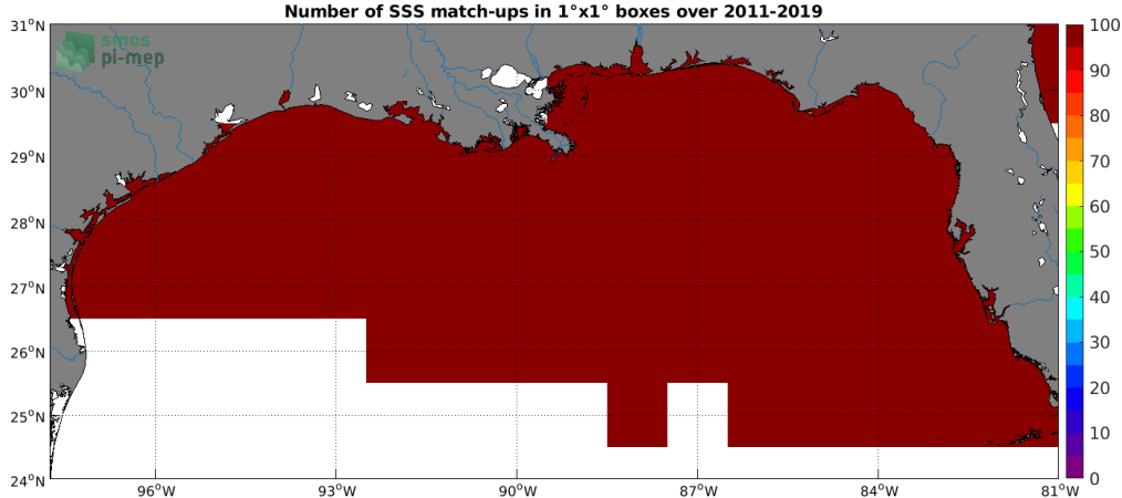
Figure 4: Number of SSS match-ups between TSG (SAMOS) SSS and the SMOS SSS L3 v2 - 9-Days (BEC) SSS product for the Mississippi river plume Pi-MEP region over 1^\circ \times 1^\circ boxes and for the full satellite product period.
