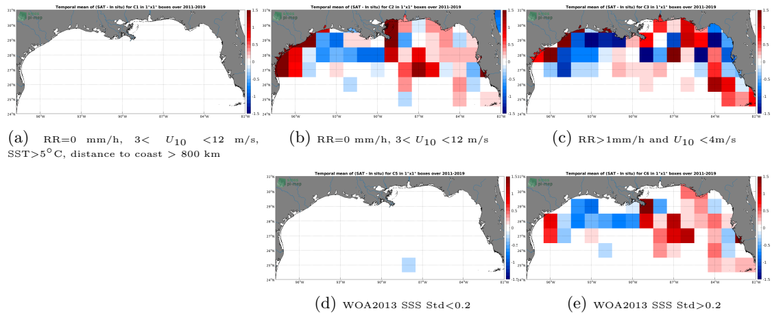
Figure 12: Temporal mean gridded over spatial boxes of size 1^{\circ}\times 1^{\circ} of \Delta\text{SSS} (SMOS SSS L3 v2 - 9-Days (BEC) - TSG (SAMOS)) for 5 different subdatasets corresponding to: \text{RR}=0 mm/h, 3 < U_{10} < 12 m/s, \text{SST} > 5^{\circ}\text{C} , distance to coast > 800 km (a), \text{RR}=0 mm/h, 3 < U_{10} < 12 m/s (b), \text{RR} > 1\text{mm/h} and U_{10} < 4\text{m/s} (c), WOA2013 SSS Std < 0.2 (d), WOA2013 SSS Std > 0.2 (e).
