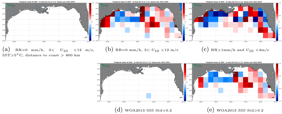
Figure 12: Temporal mean gridded over spatial boxes of size 1^{\circ}\times 1^{\circ} of \Delta\text{SSS} (SMOS SSS L3 v2 - 9-Days (BEC) - TSG (SAMOS)) for 5 different subdatasets corresponding to:RR=0 mm/h, 3 < U_{10} < 12 m/s, SST >5^{\circ}\text{C} , distance to coast > 800 km (a), RR=0 mm/h, 3 < U_{10} < 12 m/s (b), RR >1 mm/h and U_{10} < 4 m/s (c), WOA2013 SSS Std <0.2 (d), WOA2013 SSS Std >0.2 (e).
