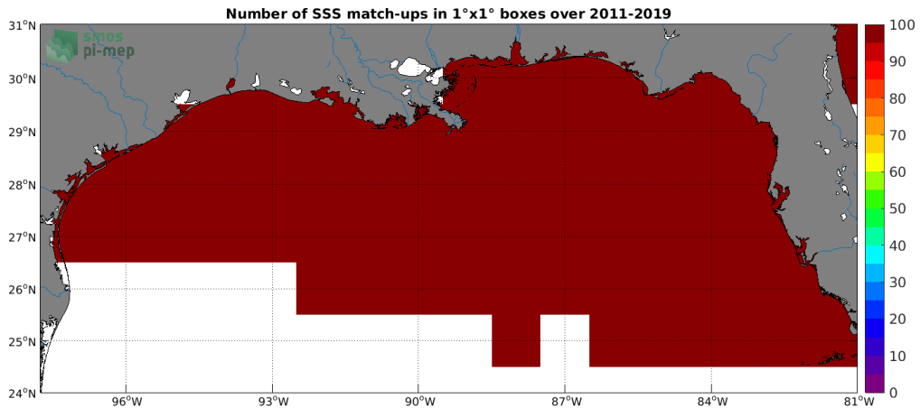
Figure 4: Number of SSS match-ups between TSG (SAMOS) SSS and the SMOS SSS L3 v2 - 9-Days (BEC) SSS product for the Mississippi river plume Pi-MEP region over 1°x1° boxes and for the full satellite product period.
