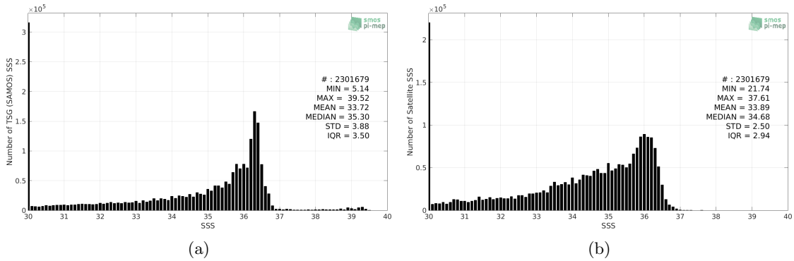
Figure 2: Histograms of SSS from TSG (SAMOS) (a) and SMOS L3 v2 - 9-Days (BEC) (b) considering all match-up pairs per bins of 0.1 over the Mississippi river plume Pi-MEP region and for the full satellite product period.
