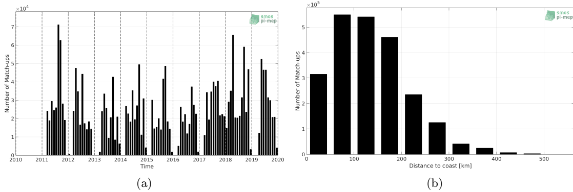
Figure 1: Number of match-ups between TSG (SAMOS) and SMOS L3 v2 - 9-Days (BEC) SSS as a function of time (a) and as function of the distance to coast (b) over the Mississippi river plume Pi-MEP region and for the full satellite product period.
