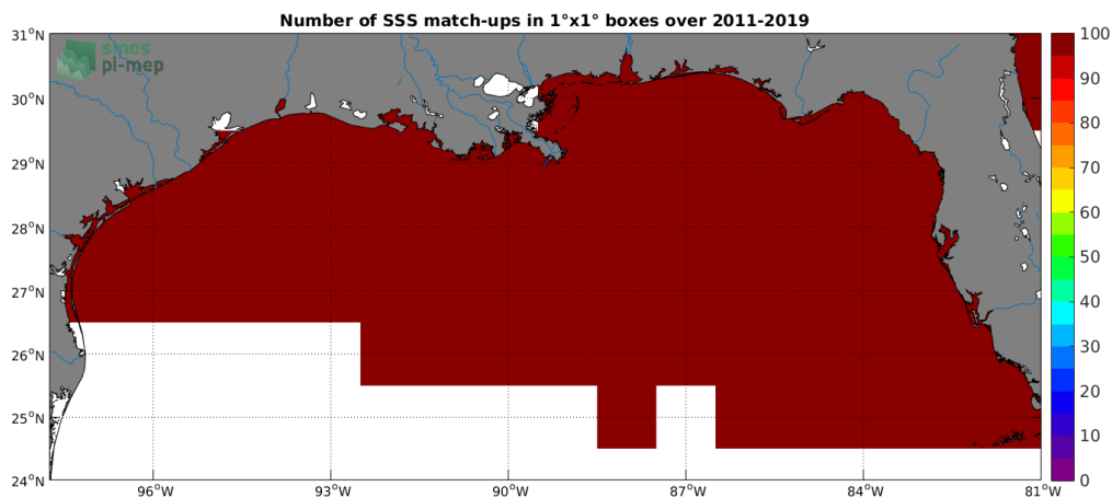
Figure 4: Number of SSS match-ups between TSG (SAMOS) SSS and the SMOS L3 v2 - 9-Days (BEC) SSS product for the Mississippi river plume Pi-MEP region over 1°x1° boxes and for the full satellite product period.
