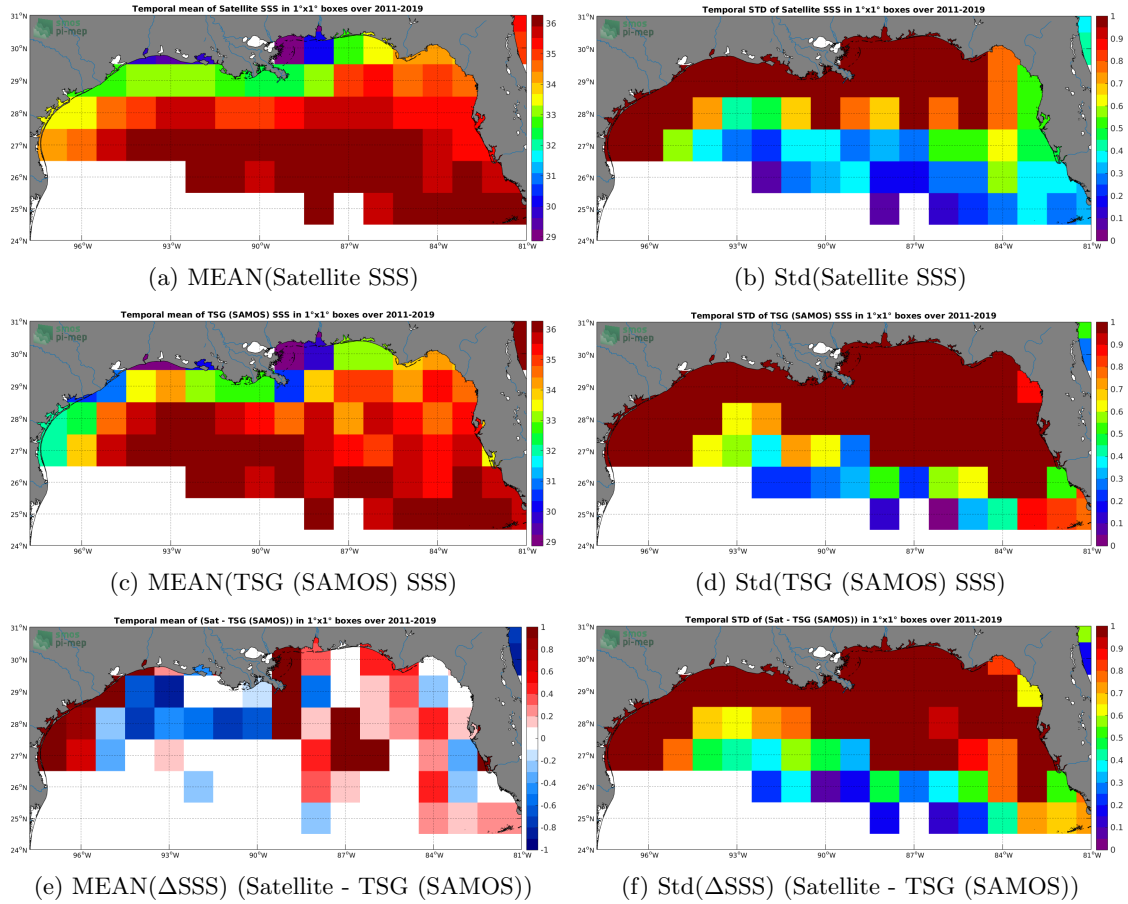
Figure 6: Temporal mean (left) and Std (right) of SSS from SMOS L3 v2 - 9-Days (BEC) (top), TSG (SAMOS) (middle), and of \Delta SSS (Satellite - TSG (SAMOS)). Only match-up pairs are used to generate these maps.
