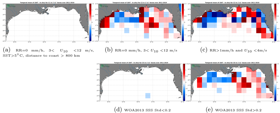
Figure 12: Temporal mean gridded over spatial boxes of size 1^{\circ}\times 1^{\circ} of \Delta\text{SSS} (SMOS L3 v2 - 9-Days (BEC) - TSG (SAMOS)) for 5 different subdatasets corresponding to:RR=0 mm/h, 3 < U_{10} < 12 m/s, SST >5^{\circ}\text{C} , distance to coast > 800 km (a), RR=0 mm/h, 3 < U_{10} < 12 m/s (b), RR >1 mm/h and U_{10} < 4 m/s (c), WOA2013 SSS Std <0.2 (d), WOA2013 SSS Std >0.2 (e).
