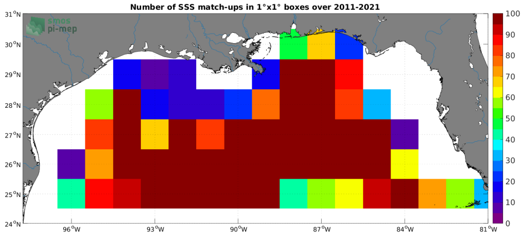
Figure 4: Number of SSS match-ups between Argo SSS and the SMOS SSS L3 v2 - 9-Days (BEC) SSS product for the Mississippi river plume Pi-MEP region over 1^\circ \times 1^\circ boxes and for the full satellite product period.
