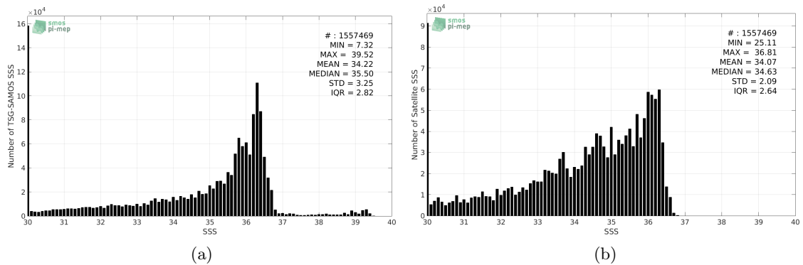
Figure 2: Histograms of SSS from TSG-SAMOS (a) and SMOS-L3-BEC-OA-V1-9DAYS-0.25DEG (b) considering all match-up pairs per bins of 0.1 over the Mississippi river plume Pi-MEP region and for the full satellite product period.
