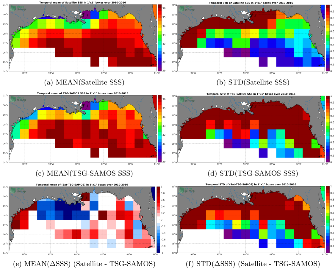
Figure 6: Temporal mean (left) and STD (right) of SSS from SMOS-L3-BEC-OA-V1-9DAYS-0.25DEG (top), TSG-SAMOS (middle), and of \Delta SSS (Satellite - TSG-SAMOS). Only match-up pairs are used to generate these maps.
