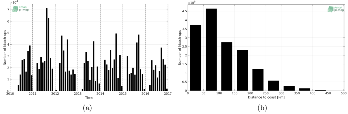
Figure 1: Number of match-ups between TSG-SAMOS and SMOS-L3-BEC-OA-V1-9DAYS-0.25DEG SSS as a function of time (a) and as function of the distance to coast (b) over the Mississippi river plume Pi-MEP region and for the full satellite product period.
