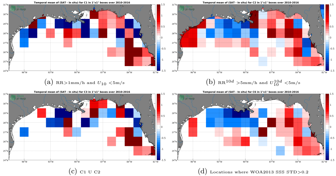
Figure 12: Temporal mean gridded over spatial boxes of size 1^\circ \times 1^\circ of \Delta SSS (SMOS-L3-BEC-OA-V1-9DAYS-0.25DEG - TSG-SAMOS) for 4 different subdatasets corresponding to: RR > 1mm/h and U_{10} < 5\text{m/s} (a), RR^{10d} > 5\text{mm/h} and U_{10}^{10d} < 5\text{m/s} (b), C1 U C2 (c), Locations where WOA2013 SSS STD > 0.2 (d).
