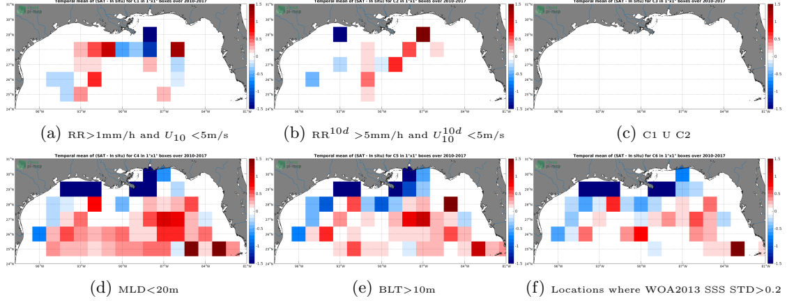
Figure 12: Temporal mean gridded over spatial boxes of size 1^\circ \times 1^\circ of \Delta SSS (SMOS-L3-BEC-OA-V1-9DAYS-0.25DEG - Argo) for 6 different subdatasets corresponding to: RR>1\text{mm/h} and U_{10}<5\text{m/s} (a), RR^{10d}>5\text{mm/h} and U_{10}^{10d}<5\text{m/s} (b), C1 U C2 (c), MLD<20\text{m} (d), BLT>10\text{m} (e), Locations where WOA2013 SSS STD>0.2 (f).
