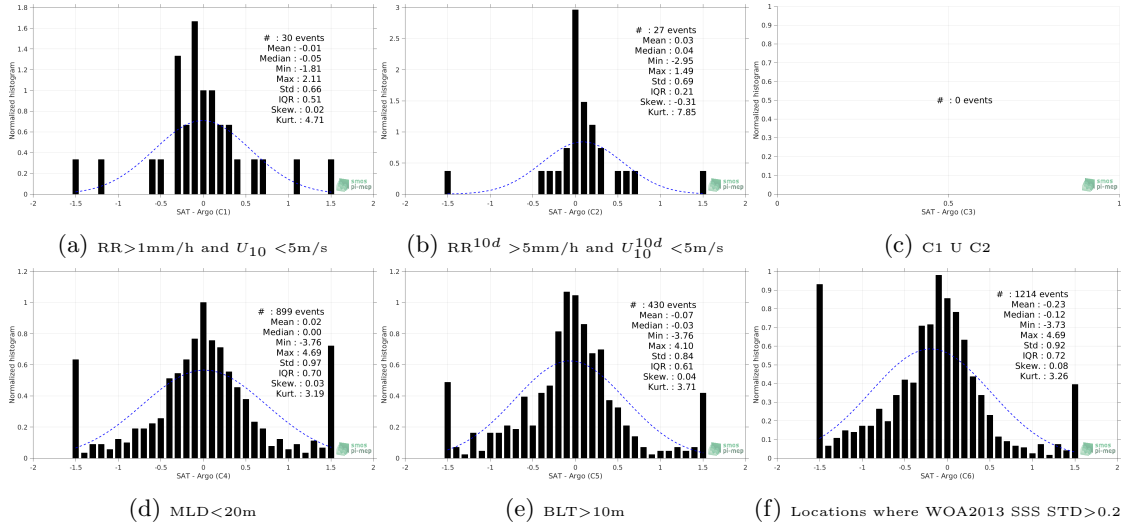
Figure 13: Normalized histogram of \Delta SSS (SMOS-L3-BEC-OA-V1-9DAYS-0.25DEG - Argo) for 6 different subdatasets corresponding to: RR>1\text{mm/h} and U_{10}<5\text{m/s} (a), RR^{10d}>5\text{mm/h} and U_{10}^{10d}<5\text{m/s} (b), C1 U C2 (c), MLD<20\text{m} (d), BLT>10\text{m} (e), Locations where WOA2013 SSS STD>0.2 (f).
