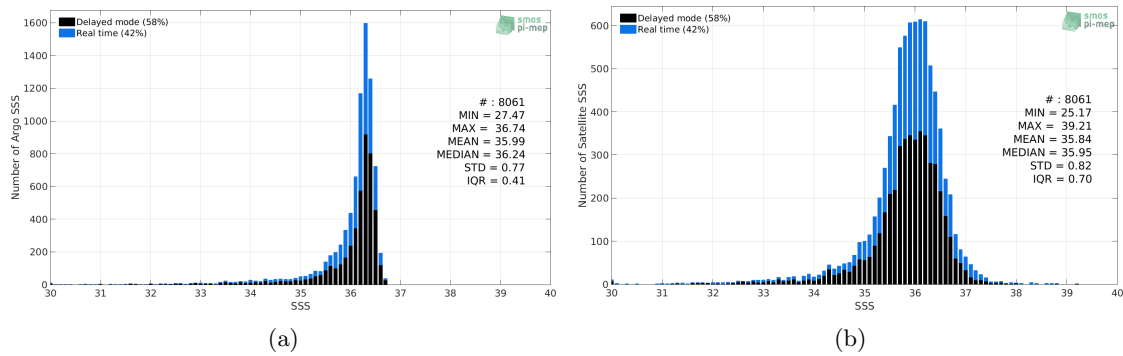
Figure 2: Histograms of SSS from Argo (a) and SMOS SSS L2-AVERAGED v700 (ESA) (b) considering all match-up pairs per bins of 0.1 over the Mississippi river plume Pi-MEP region and for the full satellite product period.
