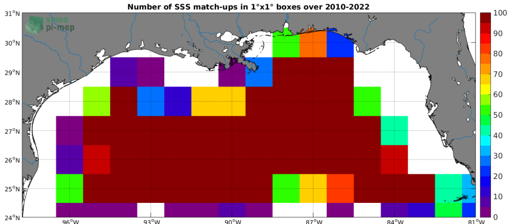
Figure 4: Number of SSS match-ups between Argo SSS and the SMOS SSS L2-AVERAGED v700 (ESA) SSS product for the Mississippi river plume Pi-MEP region over 1^\circ \times 1^\circ boxes and for the full satellite product period.
