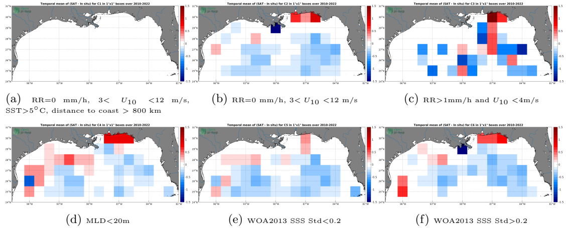
Figure 12: Temporal mean gridded over spatial boxes of size 1^{\circ}\times 1^{\circ} of \Delta\text{SSS} (SMOS SSS L2-AVERAGED v700 (ESA) - Argo) for 6 different subdatasets corresponding to:RR=0 mm/h, 3 < U_{10} < 12 m/s, SST > 5^{\circ}\text{C} , distance to coast > 800 km (a), RR=0 mm/h, 3 < U_{10} < 12 m/s (b), RR > 1\text{mm/h} and U_{10} < 4\text{m/s} (c),MLD < 20\text{m} (d),WOA2013 SSS Std < 0.2 (e),WOA2013 SSS Std > 0.2 (f).
