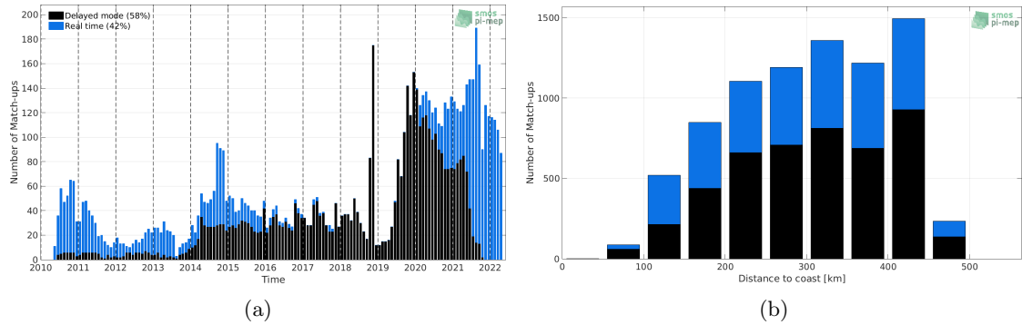
Figure 1: Number of match-ups between Argo and SMOS SSS L2-AVERAGED v700 (ESA) SSS as a function of time (a) and as function of the distance to coast (b) over the Mississippi river plume Pi-MEP region and for the full satellite product period.
