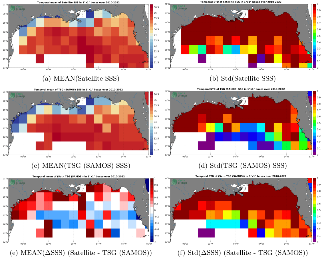
Figure 6: Temporal mean (left) and Std (right) of SSS from SMOS SSS L2 v700 (ESA) (top), TSG (SAMOS) (middle), and of \Delta\text{SSS} (Satellite - TSG (SAMOS)). Only match-up pairs are used to generate these maps.
