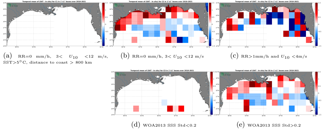
Figure 12: Temporal mean gridded over spatial boxes of size 1^{\circ} \times 1^{\circ} of \Delta\text{SSS} (SMOS SSS L2 v700 (ESA) - TSG (SAMOS)) for 5 different subdatasets corresponding to: RR=0 mm/h, 3 < U_{10} < 12 m/s, SST > 5^{\circ}\text{C} , distance to coast > 800 km (a), RR=0 mm/h, 3 < U_{10} < 12 m/s (b), RR > 1 mm/h and U_{10} < 4 m/s (c), WOA2013 SSS Std < 0.2 (d), WOA2013 SSS Std > 0.2 (e).
