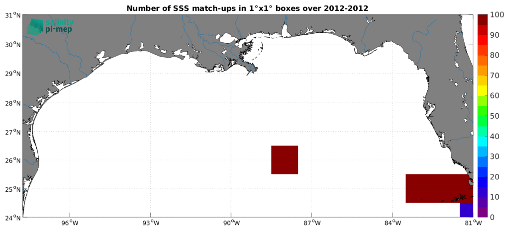
Figure 5: Number of SSS match-ups between TSG (GOSUD-Sailing-ship) SSS and the SMOS SSS L2 v700 (ESA) SSS product for the Mississippi river plume Pi-MEP region over 1^\circ \times 1^\circ boxes and for the full satellite product period.
