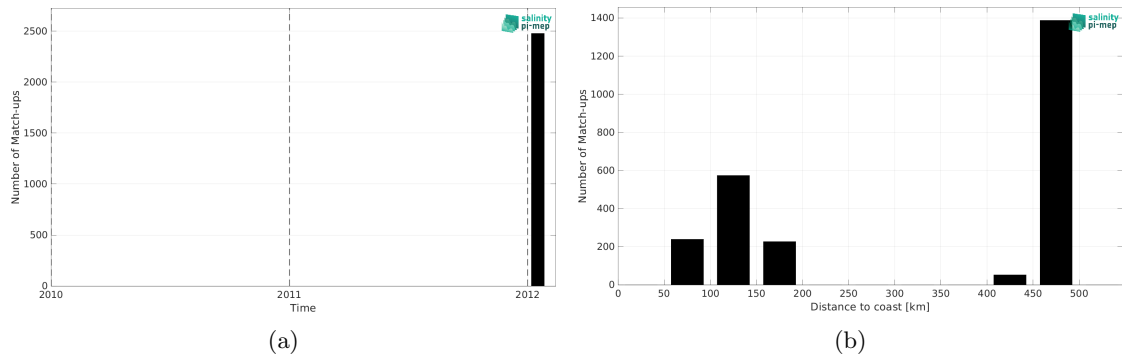
Figure 2: Number of match-ups between TSG (GOSUD-Sailing-ship) and SMOS SSS L2 v700 (ESA) SSS as a function of time (a) and as function of the distance to coast (b) over the Mississippi river plume Pi-MEP region and for the full satellite product period.
