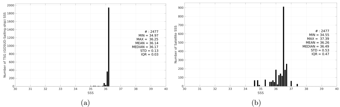
Figure 3: Histograms of SSS from TSG (GOSUD-Sailing-ship) (a) and SMOS SSS L2 v700 (ESA) (b) considering all match-up pairs per bins of 0.1 over the Mississippi river plume Pi-MEP region and for the full satellite product period.
