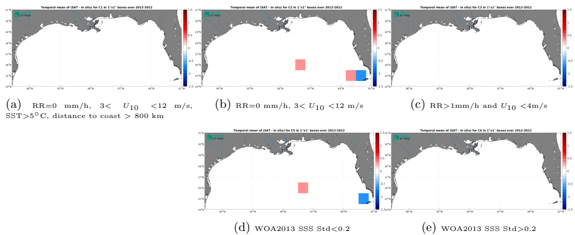
Figure 14: Temporal mean gridded over spatial boxes of size 1^\circ \times 1^\circ of \Delta SSS (SMOS SSS L2 v700 (ESA) - TSG (GOSUD-Sailing-ship)) for 5 different subdatasets corresponding to:RR=0 mm/h, 3 < U_{10} < 12 m/s, SST>5°C, distance to coast > 800 km (a), RR=0 mm/h, 3 < U_{10} < 12 m/s (b), RR>1mm/h and U_{10} < 4 m/s (c), WOA2013 SSS Std<0.2 (d), WOA2013 SSS Std>0.2 (e).
