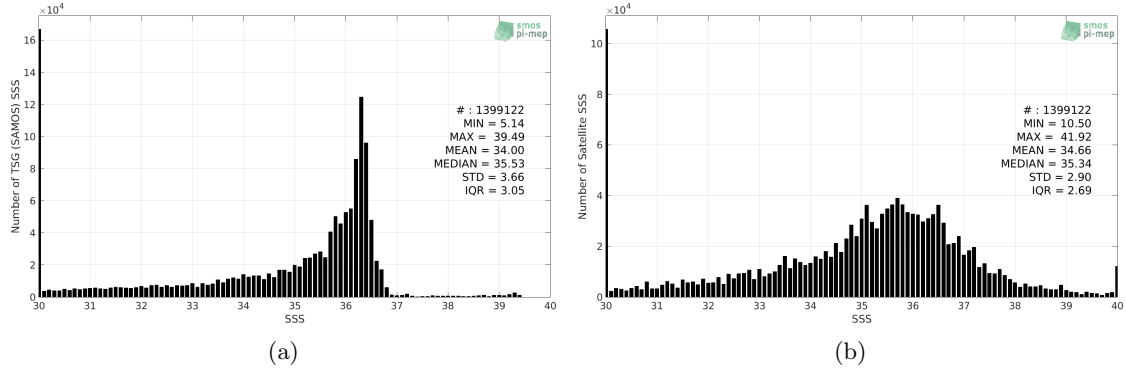
Figure 2: Histograms of SSS from TSG (SAMOS) (a) and SMOS SSS L2 v662 (ESA) (b) considering all match-up pairs per bins of 0.1 over the Mississippi river plume Pi-MEP region and for the full satellite product period.
