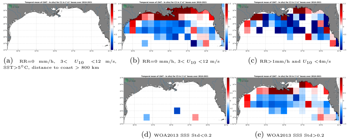
Figure 12: Temporal mean gridded over spatial boxes of size 1^{\circ}\times 1^{\circ} of \Delta\text{SSS} (SMOS SSS L2 v662 (ESA) - TSG (SAMOS)) for 5 different subdatasets corresponding to:RR=0 mm/h, 3 < U_{10} < 12 m/s, SST >5^{\circ}\text{C} , distance to coast > 800 km (a), RR=0 mm/h, 3 < U_{10} < 12 m/s (b), RR >1 mm/h and U_{10} < 4 m/s (c), WOA2013 SSS Std <0.2 (d), WOA2013 SSS Std >0.2 (e).
