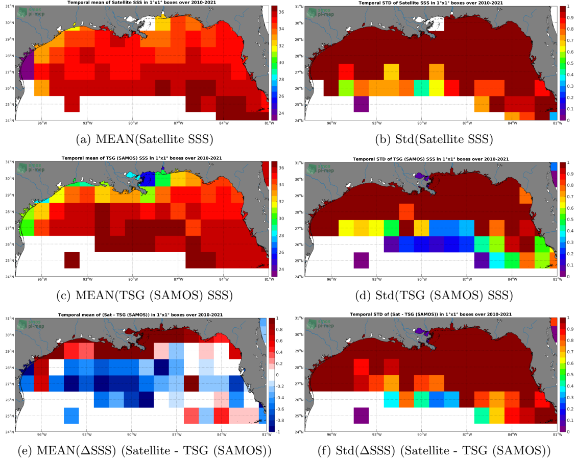
Figure 6: Temporal mean (left) and Std (right) of SSS from SMOS SSS L2 v662 (ESA) (top), TSG (SAMOS) (middle), and of \Delta SSS (Satellite - TSG (SAMOS)). Only match-up pairs are used to generate these maps.
