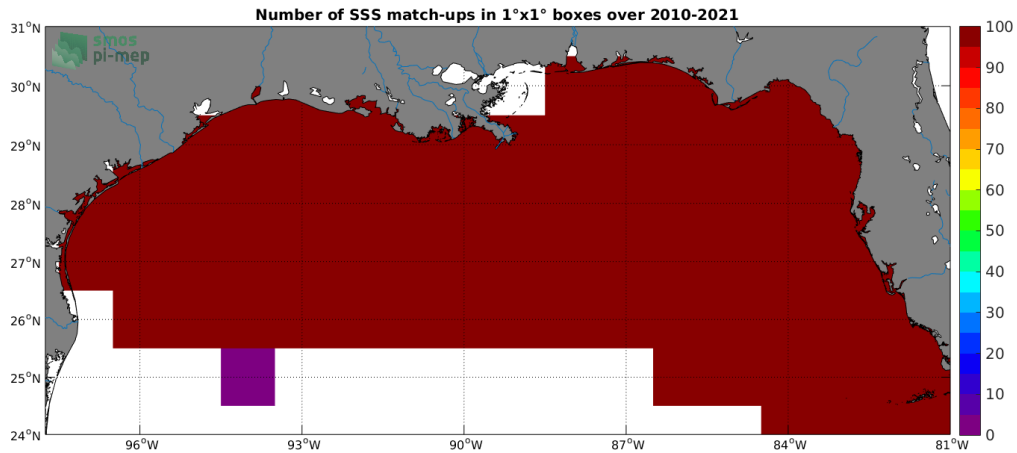
Figure 4: Number of SSS match-ups between TSG (SAMOS) SSS and the SMOS SSS L2 v662 (ESA) SSS product for the Mississippi river plume Pi-MEP region over 1^\circ \times 1^\circ boxes and for the full satellite product period.
