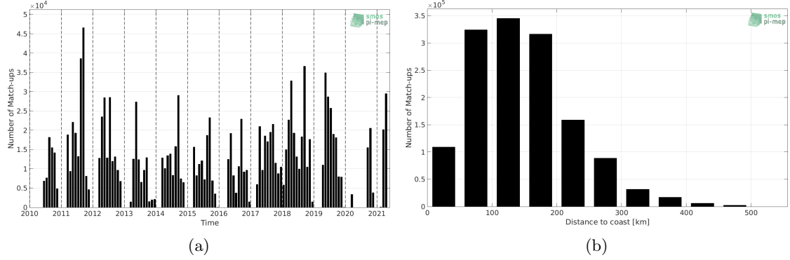
Figure 1: Number of match-ups between TSG (SAMOS) and SMOS SSS L2 v662 (ESA) SSS as a function of time (a) and as function of the distance to coast (b) over the Mississippi river plume Pi-MEP region and for the full satellite product period.
