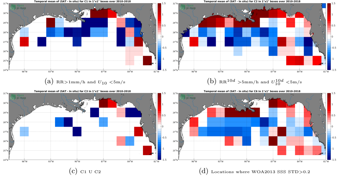
Figure 12: Temporal mean gridded over spatial boxes of size 1^\circ \times 1^\circ of \Delta SSS (SMOS-L2-DPGS-v662 - TSG-SAMOS) for 4 different subdatasets corresponding to: RR > 1\text{mm/h} and U_{10} < 5\text{m/s} (a), RR^{10d} > 5\text{mm/h} and U_{10}^{10d} < 5\text{m/s} (b), C1 \cup C2 (c), Locations where WOA2013 SSS STD > 0.2 (d).
