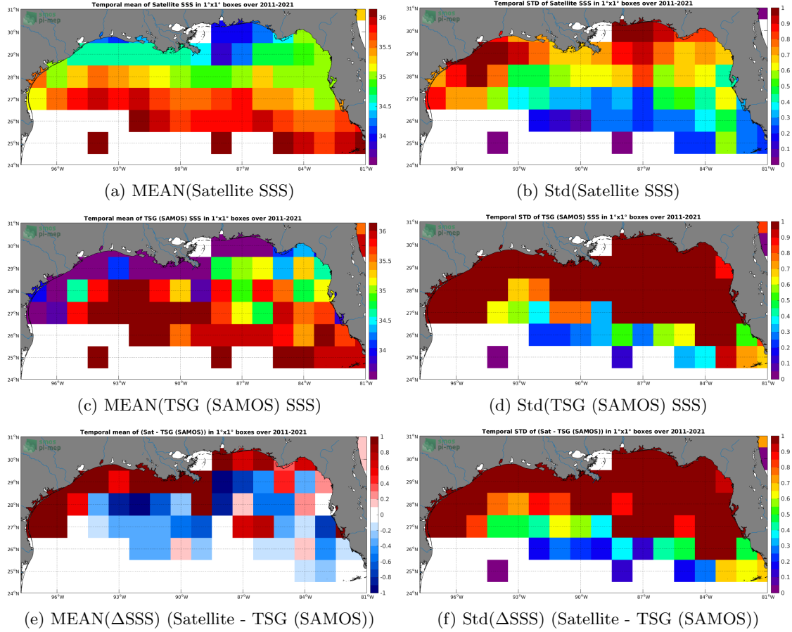
Figure 6: Temporal mean (left) and Std (right) of SSS from SMAP SSS L4 OI v1 - 7 Days (IPRC) (top), TSG (SAMOS) (middle), and of \Delta\text{SSS} (Satellite - TSG (SAMOS)). Only match-up pairs are used to generate these maps.
