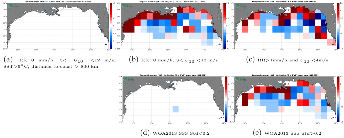
Figure 12: Temporal mean gridded over spatial boxes of size 1^{\circ}\times 1^{\circ} of \Delta\text{SSS} (SMAP SSS L4 OI v1 - 7 Days (IPRC) - TSG (SAMOS)) for 5 different subdatasets corresponding to:RR=0 mm/h, 3 < U_{10} < 12 m/s, SST >5^{\circ}\text{C} , distance to coast > 800 km (a), RR=0 mm/h, 3 < U_{10} < 12 m/s (b), RR >1\text{mm/h} and U_{10} < 4\text{m/s} (c), WOA2013 SSS Std <0.2 (d), WOA2013 SSS Std >0.2 (e).
