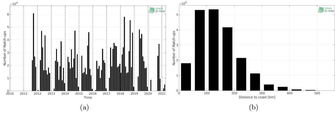
Figure 1: Number of match-ups between TSG (SAMOS) and SMAP SSS L4 OI v1 - 7 Days (IPRC) SSS as a function of time (a) and as function of the distance to coast (b) over the Mississippi river plume Pi-MEP region and for the full satellite product period.
