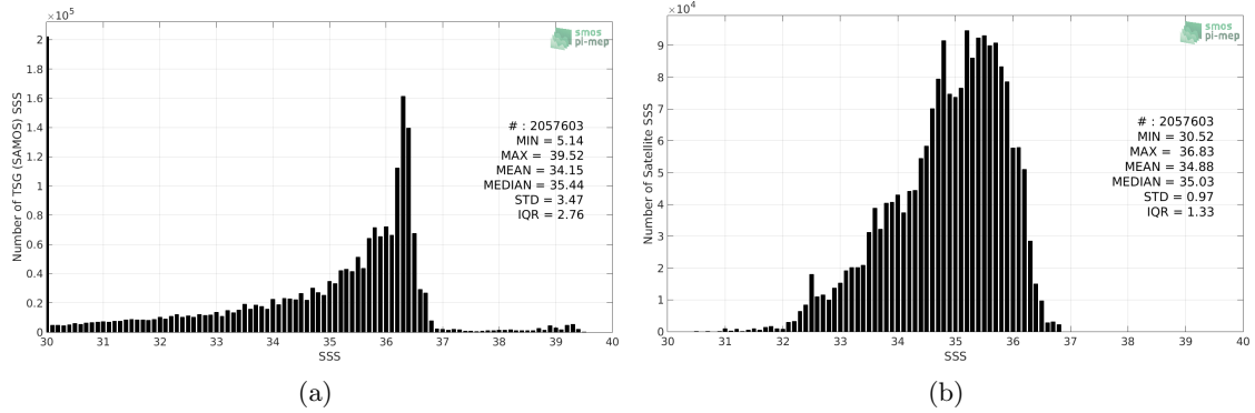
Figure 2: Histograms of SSS from TSG (SAMOS) (a) and SMAP SSS L4 OI v1 - 7 Days (IPRC) (b) considering all match-up pairs per bins of 0.1 over the Mississippi river plume Pi-MEP region and for the full satellite product period.
