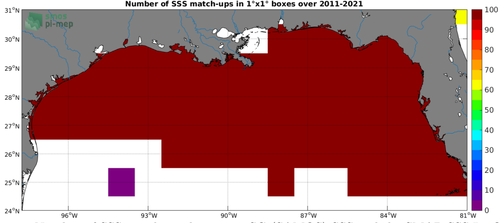
Figure 4: Number of SSS match-ups between TSG (SAMOS) SSS and the SMAP SSS L4 OI v1 - 7 Days (IPRC) SSS product for the Mississippi river plume Pi-MEP region over 1^\circ \times 1^\circ boxes and for the full satellite product period.
