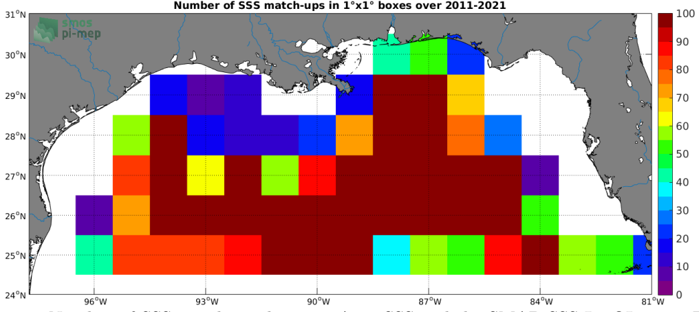
Figure 4: Number of SSS match-ups between Argo SSS and the SMAP SSS L4 OI v1 - 7 Days (IPRC) SSS product for the Mississippi river plume Pi-MEP region over 1^\circ \times 1^\circ boxes and for the full satellite product period.
