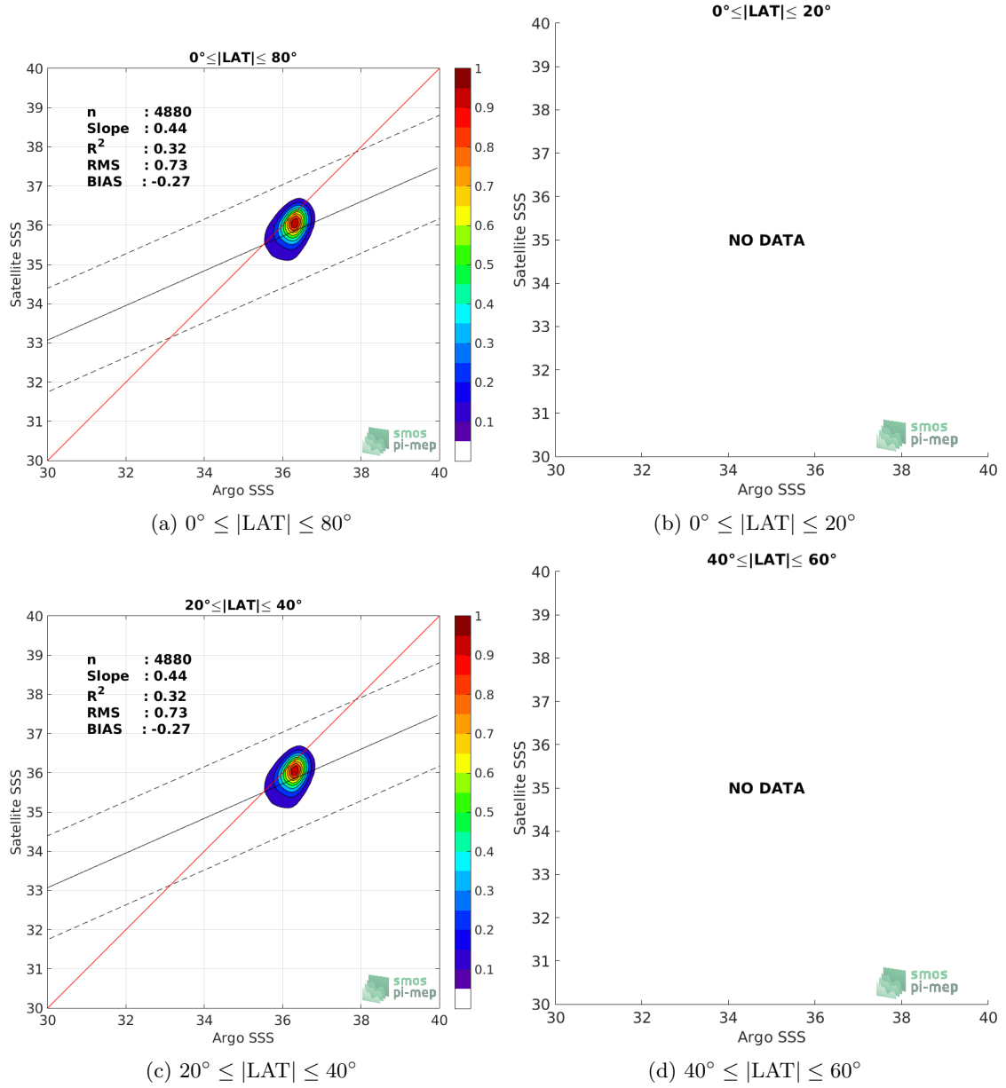
Figure 9: Contour maps of the concentration of SMAP SSS L4 OI v1 - 7 Days (IPRC) SSS (y-axis) versus Argo SSS (x-axis) at match-up pairs for different latitude bands. For each plot, the red line shows x=y . The black thin and dashed lines indicate a linear fit through the data cloud and the \pm 95\% confidence levels, respectively. The number match-up pairs n , the slope and R^2 coefficient of the linear fit, the root mean square (RMS) and the mean bias between satellite and in situ data are indicated for each latitude band in each plots.
