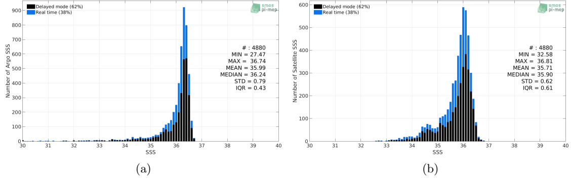
Figure 2: Histograms of SSS from Argo (a) and SMAP SSS L4 OI v1 - 7 Days (IPRC) (b) considering all match-up pairs per bins of 0.1 over the Mississippi river plume Pi-MEP region and for the full satellite product period.
