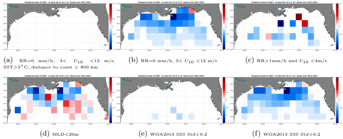
Figure 12: Temporal mean gridded over spatial boxes of size 1^{\circ} \times 1^{\circ} of \Delta\text{SSS} (SMAP SSS L4 OI v1 - 7 Days (IPRC) - Argo) for 6 different subdatasets corresponding to: \text{RR}=0 \text{ mm/h}, 3 < U_{10} < 12 \text{ m/s}, \text{SST} > 5^{\circ}\text{C} , distance to coast > 800 \text{ km} (a), \text{RR}=0 \text{ mm/h}, 3 < U_{10} < 12 \text{ m/s} (b), \text{RR} > 1\text{mm/h} and U_{10} < 4\text{m/s} (c), \text{MLD} < 20\text{m} (d), \text{WOA2013 SSS Std} < 0.2 (e), \text{WOA2013 SSS Std} > 0.2 (f).
