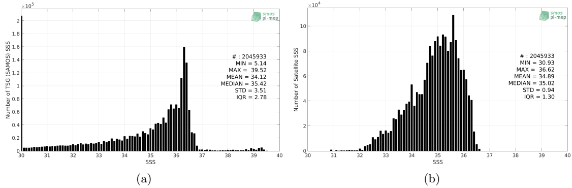
Figure 2: Histograms of SSS from TSG (SAMOS) (a) and SMAP SSS L4 OI v1 - Monthly (IPRC) (b) considering all match-up pairs per bins of 0.1 over the Mississippi river plume Pi-MEP region and for the full satellite product period.
