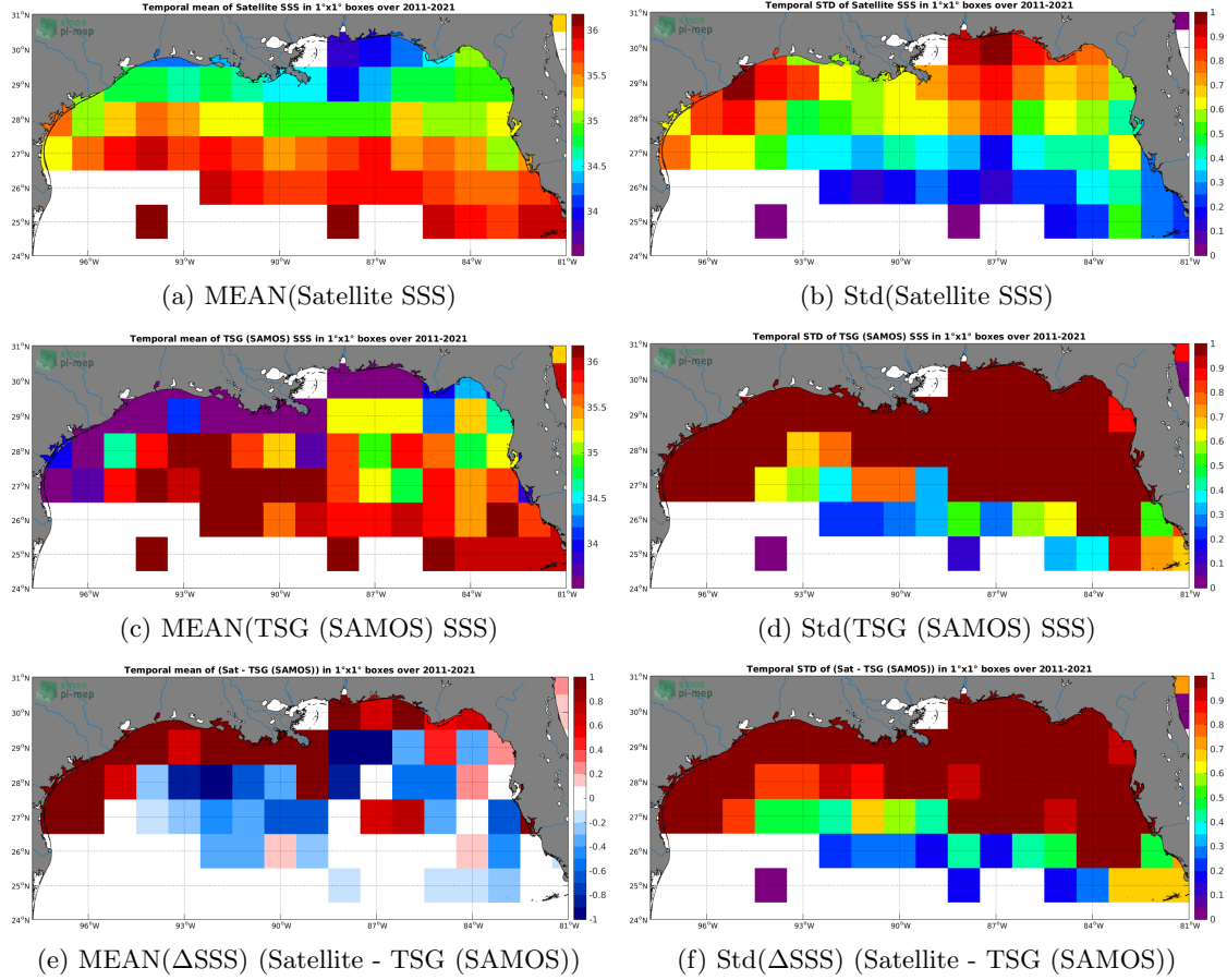
Figure 6: Temporal mean (left) and Std (right) of SSS from SMAP SSS L4 OI v1 - Monthly (IPRC) (top), TSG (SAMOS) (middle), and of \Delta\text{SSS} (Satellite - TSG (SAMOS)). Only match-up pairs are used to generate these maps.
