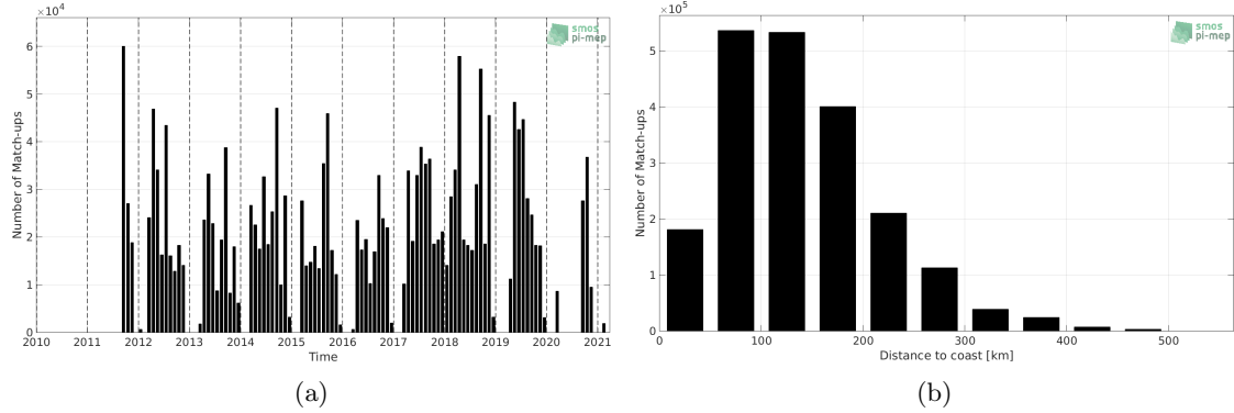
Figure 1: Number of match-ups between TSG (SAMOS) and SMAP SSS L4 OI v1 - Monthly (IPRC) SSS as a function of time (a) and as function of the distance to coast (b) over the Mississippi river plume Pi-MEP region and for the full satellite product period.
