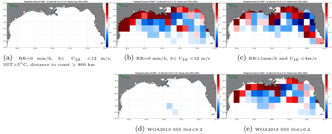
Figure 12: Temporal mean gridded over spatial boxes of size 1^{\circ}\times 1^{\circ} of \Delta\text{SSS} (SMAP SSS L4 OI v1 - Monthly (IPRC) - TSG (SAMOS)) for 5 different subdatasets corresponding to:RR=0 mm/h, 3 < U_{10} < 12 m/s, SST >5^{\circ}\text{C} , distance to coast > 800 km (a), RR=0 mm/h, 3 < U_{10} < 12 m/s (b), RR >1\text{mm/h} and U_{10} < 4\text{m/s} (c), WOA2013 SSS Std <0.2 (d), WOA2013 SSS Std >0.2 (e).
