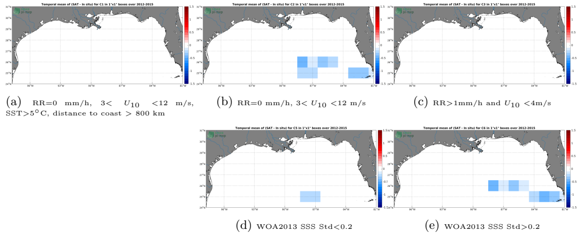
Figure 12: Temporal mean gridded over spatial boxes of size 1^\circ \times 1^\circ of \Delta SSS (SMAP SSS L4 OI v1 - Monthly (IPRC) - TSG (GOSUD-Sailing-ship)) for 5 different subdatasets corresponding to: RR=0 mm/h, 3 < U_{10} < 12 m/s, SST >5^\circ\text{C} , distance to coast > 800 km (a), RR=0 mm/h, 3 < U_{10} < 12 m/s (b), RR >1 mm/h and U_{10} < 4 m/s (c), WOA2013 SSS Std <0.2 (d), WOA2013 SSS Std >0.2 (e).
