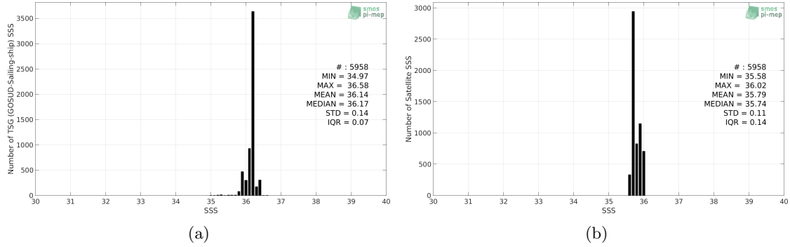
Figure 2: Histograms of SSS from TSG (GOSUD-Sailing-ship) (a) and SMAP SSS L4 OI v1 - Monthly (IPRC) (b) considering all match-up pairs per bins of 0.1 over the Mississippi river plume Pi-MEP region and for the full satellite product period.
