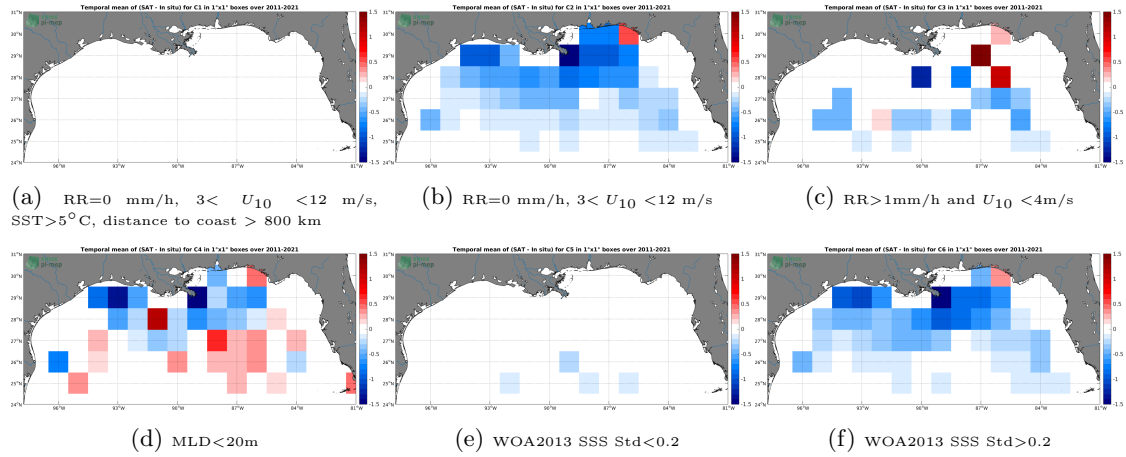
Figure 12: Temporal mean gridded over spatial boxes of size 1^{\circ} \times 1^{\circ} of \Delta\text{SSS} (SMAP SSS L4 OI v1 - Monthly (IPRC) - Argo) for 6 different subdatasets corresponding to: \text{RR}=0 mm/h, 3 < U_{10} < 12 m/s, \text{SST} > 5^{\circ}\text{C} , distance to coast > 800 km (a), \text{RR}=0 mm/h, 3 < U_{10} < 12 m/s (b), \text{RR} > 1\text{mm/h} and U_{10} < 4\text{m/s} (c), \text{MLD} < 20\text{m} (d), WOA2013 SSS Std < 0.2 (e), WOA2013 SSS Std > 0.2 (f).
