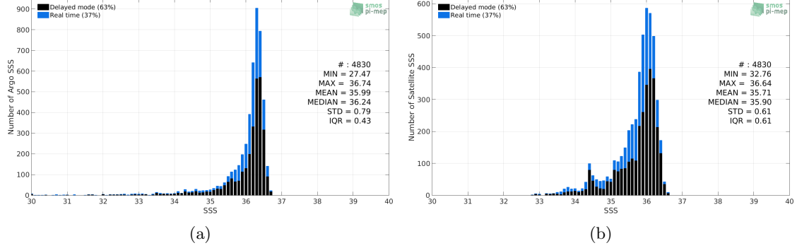
Figure 2: Histograms of SSS from Argo (a) and SMAP SSS L4 OI v1 - Monthly (IPRC) (b) considering all match-up pairs per bins of 0.1 over the Mississippi river plume Pi-MEP region and for the full satellite product period.
