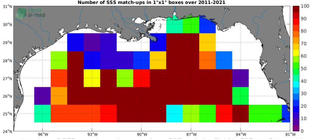
Figure 4: Number of SSS match-ups between Argo SSS and the SMAP SSS L4 OI v1 - Monthly (IPRC) SSS product for the Mississippi river plume Pi-MEP region over 1^\circ \times 1^\circ boxes and for the full satellite product period.
