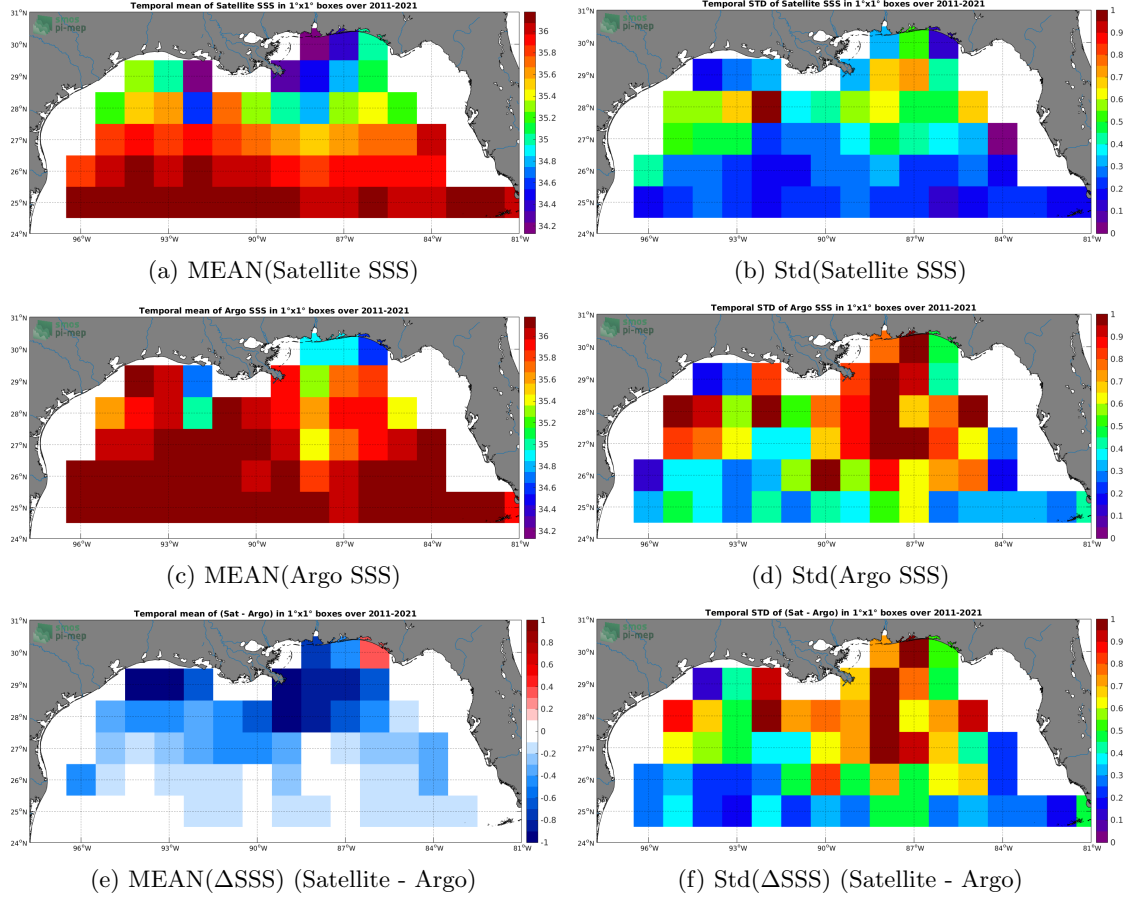
Figure 6: Temporal mean (left) and Std (right) of SSS from SMAP SSS L4 OI v1 - Monthly (IPRC) (top), Argo (middle), and of \Delta\text{SSS}(\text{Satellite} - \text{Argo}) . Only match-up pairs are used to generate these maps.
