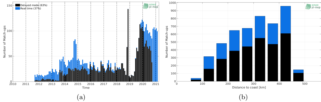
Figure 1: Number of match-ups between Argo and SMAP SSS L4 OI v1 - Monthly (IPRC) SSS as a function of time (a) and as function of the distance to coast (b) over the Mississippi river plume Pi-MEP region and for the full satellite product period.
