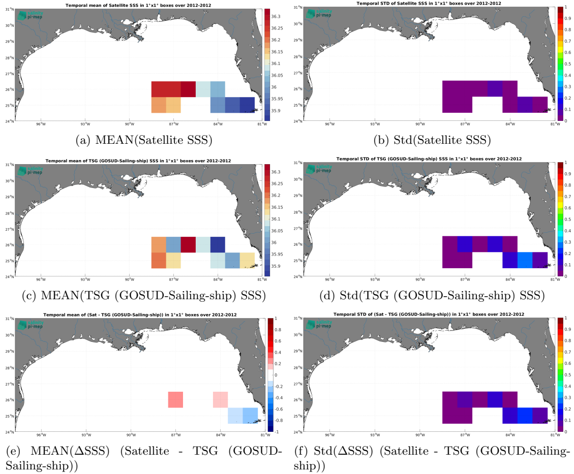
Figure 7: Temporal mean (left) and Std (right) of SSS from SMAP SSS L4 OI v3 - Monthly (ESR) (top), TSG (GOSUD-Sailing-ship) (middle), and of \Delta\text{SSS} (Satellite - TSG (GOSUD-Sailing-ship)). Only match-up pairs are used to generate these maps.
