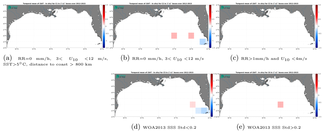
Figure 14: Temporal mean gridded over spatial boxes of size 1^\circ \times 1^\circ of \Delta SSS (SMAP SSS L4 OI v3 - Monthly (ESR) - TSG (GOSUD-Sailing-ship)) for 5 different subdatasets corresponding to: RR=0 mm/h, 3 < U_{10} < 12 m/s, SST > 5°C, distance to coast > 800 km (a), RR=0 mm/h, 3 < U_{10} < 12 m/s (b), RR > 1 mm/h and U_{10} < 4 m/s (c), WOA2013 SSS Std < 0.2 (d), WOA2013 SSS Std > 0.2 (e).
