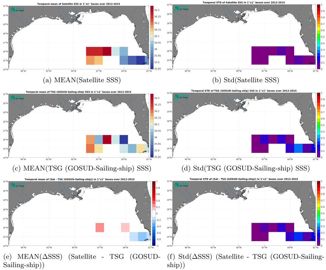
Figure 7: Temporal mean (left) and Std (right) of SSS from SMAP SSS L4 OI v3 - Monthly (ESR) (top), TSG (GOSUD-Sailing-ship) (middle), and of \Delta SSS (Satellite - TSG (GOSUD-Sailing-ship)). Only match-up pairs are used to generate these maps.
