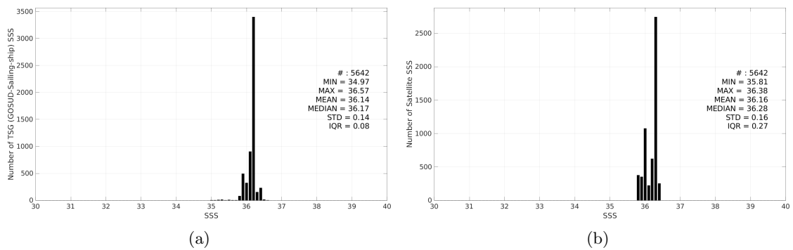
Figure 3: Histograms of SSS from TSG (GOSUD-Sailing-ship) (a) and SMAP SSS L4 OI v3 - Monthly (ESR) (b) considering all match-up pairs per bins of 0.1 over the Mississippi river plume Pi-MEP region and for the full satellite product period.
