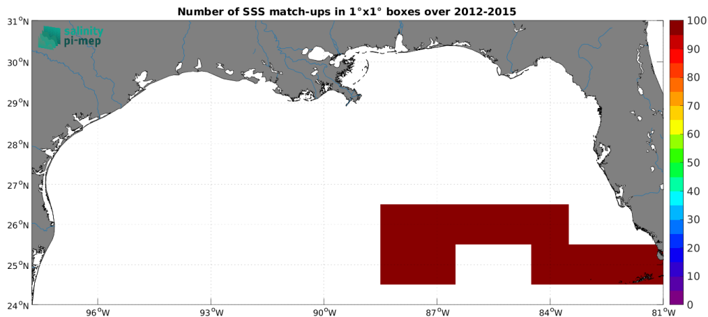
Figure 5: Number of SSS match-ups between TSG (GOSUD-Sailing-ship) SSS and the SMAP SSS L4 OI v3 - Monthly (ESR) SSS product for the Mississippi river plume Pi-MEP region over 1^\circ \times 1^\circ boxes and for the full satellite product period.
