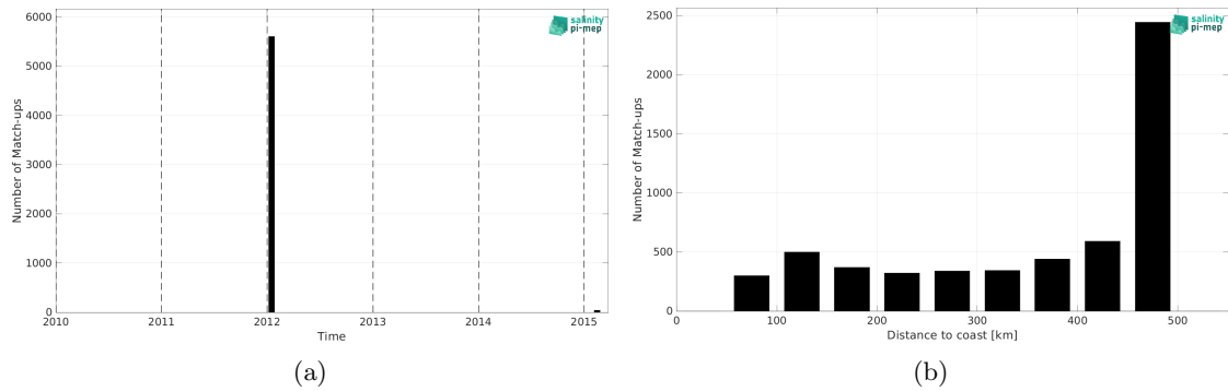
Figure 2: Number of match-ups between TSG (GOSUD-Sailing-ship) and SMAP SSS L4 OI v3 - Monthly (ESR) SSS as a function of time (a) and as function of the distance to coast (b) over the Mississippi river plume Pi-MEP region and for the full satellite product period.
