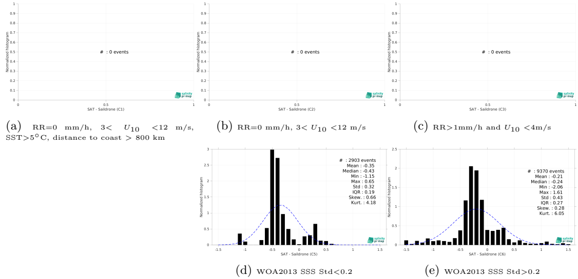
Figure 15: Normalized histogram of \Delta SSS (SMAP SSS L4 OI v3 - Monthly (ESR) - Saldrone) for 5 different subdatasets corresponding to: RR=0 mm/h, 3 < U_{10} < 12 m/s, SST > 5°C, distance to coast > 800 km (a), RR=0 mm/h, 3 < U_{10} < 12 m/s (b), RR > 1mm/h and U_{10} < 4 m/s (c), WOA2013 SSS Std < 0.2 (d), WOA2013 SSS Std > 0.2 (e).
