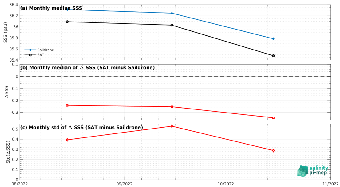
Figure 8: Time series of the monthly median SSS (top), median of \Delta SSS (Satellite - Sairdrones) and Std of \Delta SSS (Satellite - Sairdrones) over the Mississippi river plume Pi-MEP region considering all match-ups collected by the Pi-MEP.
