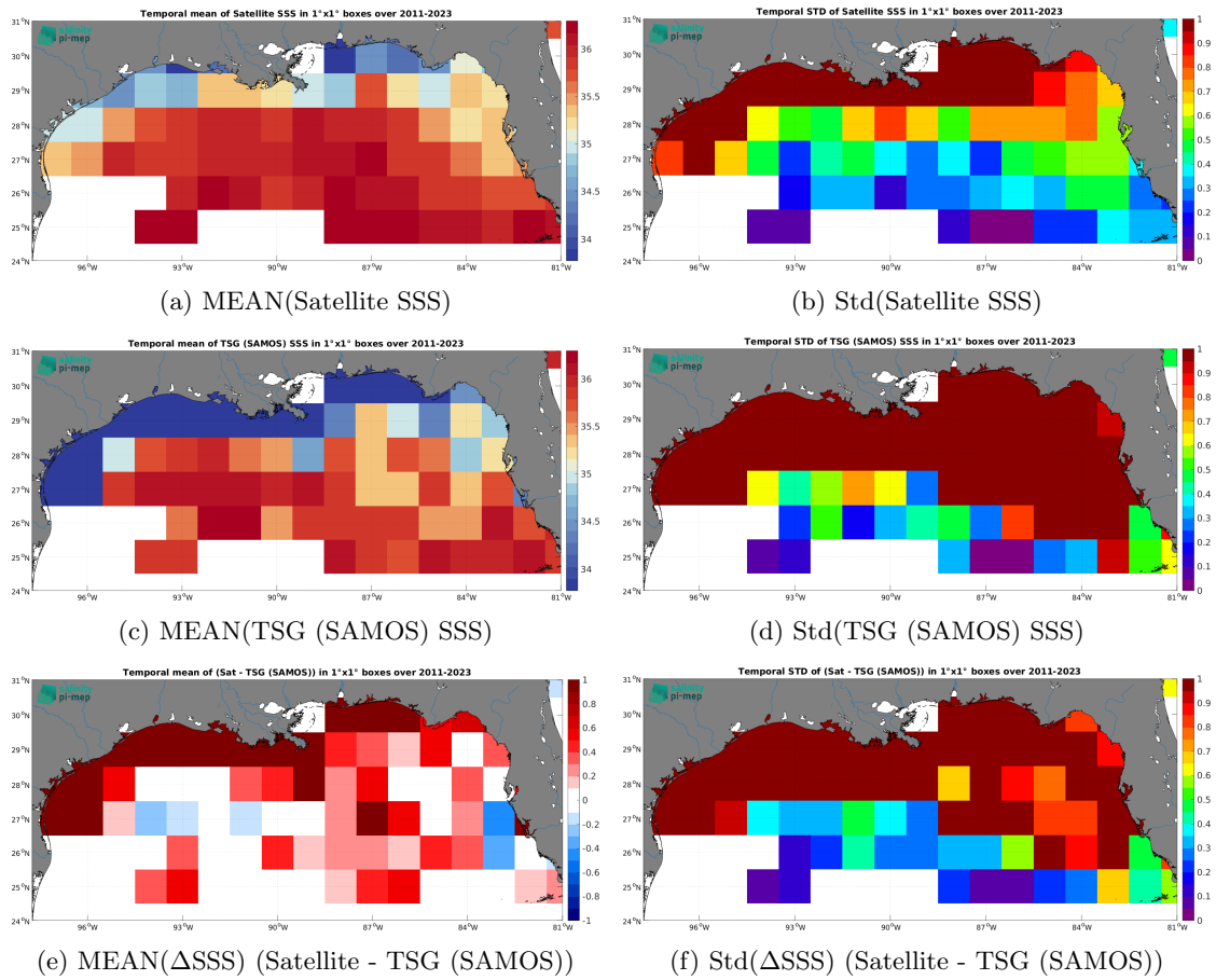
Figure 7: Temporal mean (left) and Std (right) of SSS from SMAP SSS L4 OI v3 - Daily (ESR) (top), TSG (SAMOS) (middle), and of \Delta SSS (Satellite - TSG (SAMOS)). Only match-up pairs are used to generate these maps.
