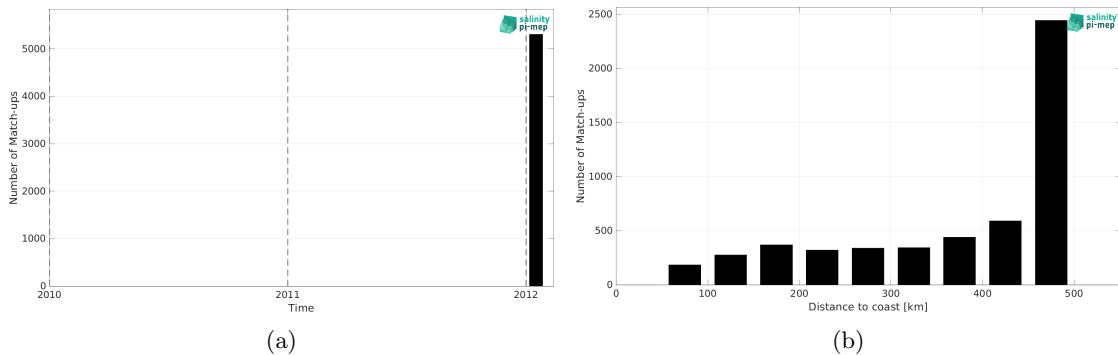
Figure 2: Number of match-ups between TSG (GOSUD-Sailing-ship) and SMAP SSS L4 OI v3 - Daily (ESR) SSS as a function of time (a) and as function of the distance to coast (b) over the Mississippi river plume Pi-MEP region and for the full satellite product period.
