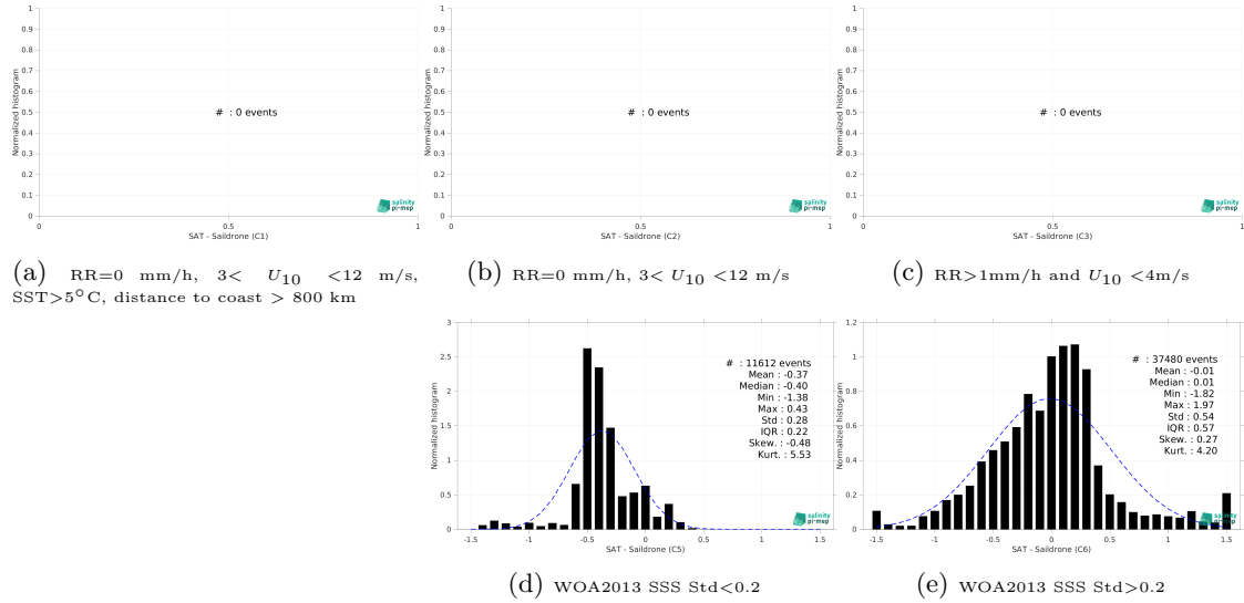
Figure 15: Normalized histogram of \Delta SSS (SMAP SSS L4 OI v3 - Daily (ESR) - Saildrone) for 5 different subdatasets corresponding to: RR=0 mm/h, 3 < U_{10} < 12 m/s, SST>5°C, distance to coast > 800 km (a), RR=0 mm/h, 3 < U_{10} < 12 m/s (b), RR>1mm/h and U_{10} < 4 m/s (c), WOA2013 SSS Std<0.2 (d), WOA2013 SSS Std>0.2 (e).
