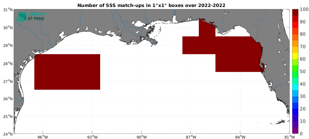
Figure 5: Number of SSS match-ups between Saildrone SSS and the SMAP SSS L4 OI v3 - Daily (ESR) SSS product for the Mississippi river plume Pi-MEP region over 1^\circ \times 1^\circ boxes and for the full satellite product period.
