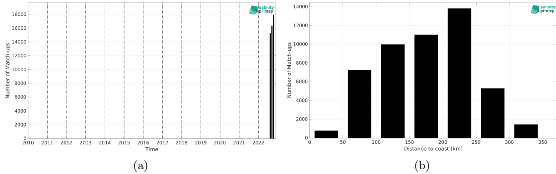
Figure 2: Number of match-ups between Saildrone and SMAP SSS L4 OI v3 - Daily (ESR) SSS as a function of time (a) and as function of the distance to coast (b) over the Mississippi river plume Pi-MEP region and for the full satellite product period.
