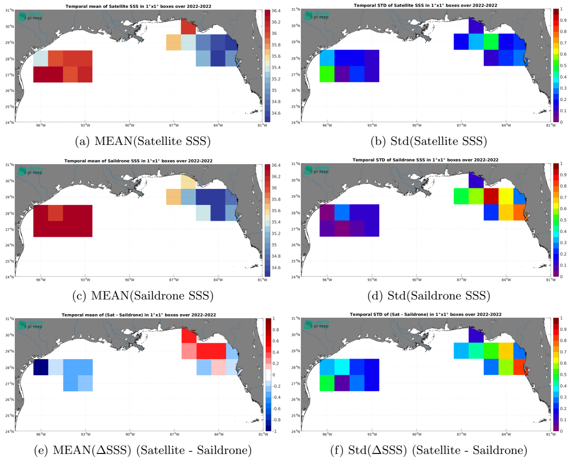
Figure 7: Temporal mean (left) and Std (right) of SSS from SMAP SSS L4 OI v3 - Daily (ESR) (top), Saildrone (middle), and of \Delta SSS (Satellite - Saildrone). Only match-up pairs are used to generate these maps.
