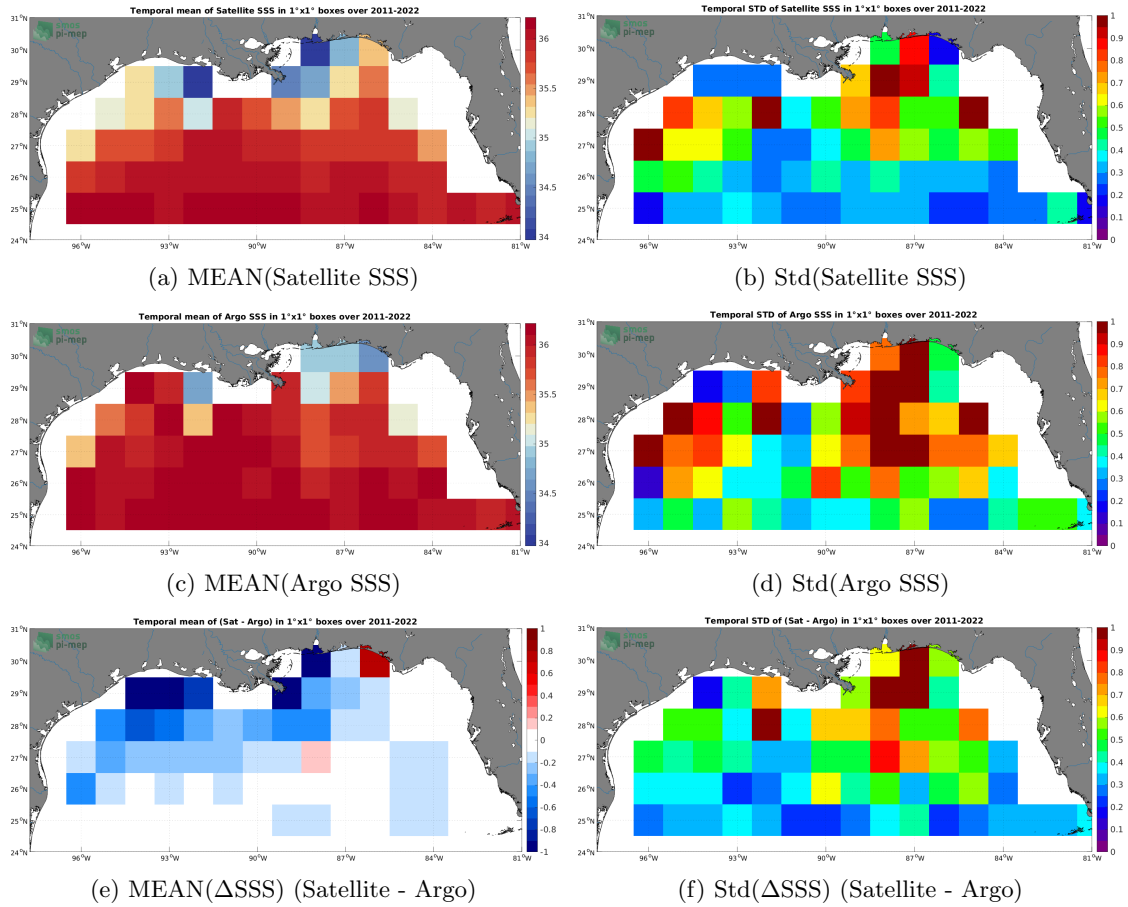
Figure 6: Temporal mean (left) and Std (right) of SSS from SMAP SSS L4 OI v2 - 7 Days (ESR) (top), Argo (middle), and of \Delta SSS (Satellite - Argo). Only match-up pairs are used to generate these maps.
