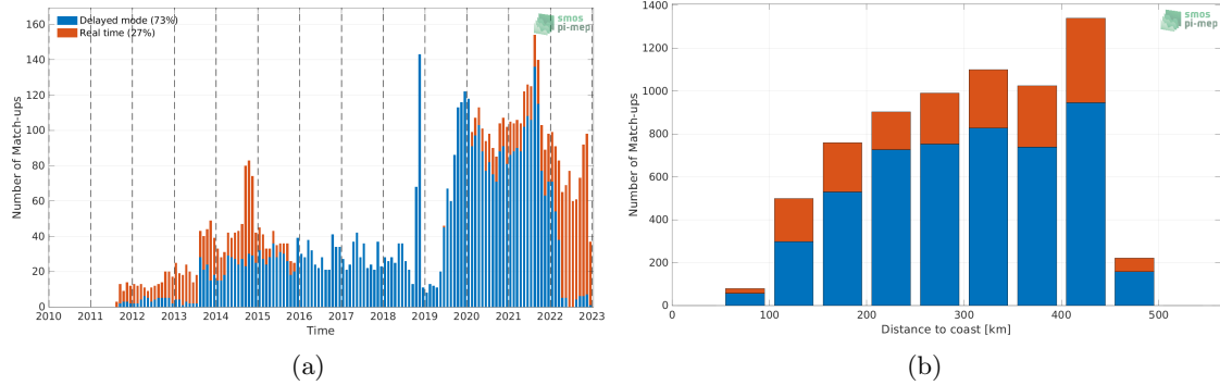
Figure 1: Number of match-ups between Argo and SMAP SSS L4 OI v2 - 7 Days (ESR) SSS as a function of time (a) and as function of the distance to coast (b) over the Mississippi river plume Pi-MEP region and for the full satellite product period.
