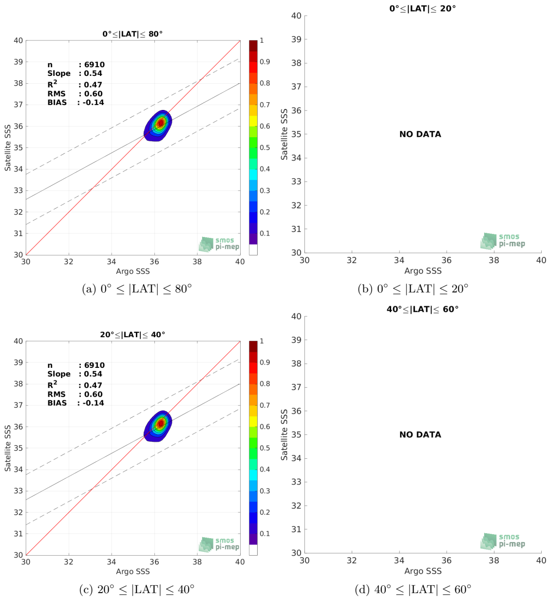
Figure 9: Contour maps of the concentration of SMAP SSS L4 OI v2 - 7 Days (ESR) SSS (y-axis) versus Argo SSS (x-axis) at match-up pairs for different latitude bands. For each plot, the red line shows x=y . The black thin and dashed lines indicate a linear fit through the data cloud and the \pm 95\% confidence levels, respectively. The number match-up pairs n , the slope and R^2 coefficient of the linear fit, the root mean square (RMS) and the mean bias between satellite and in situ data are indicated for each latitude band in each plots.
