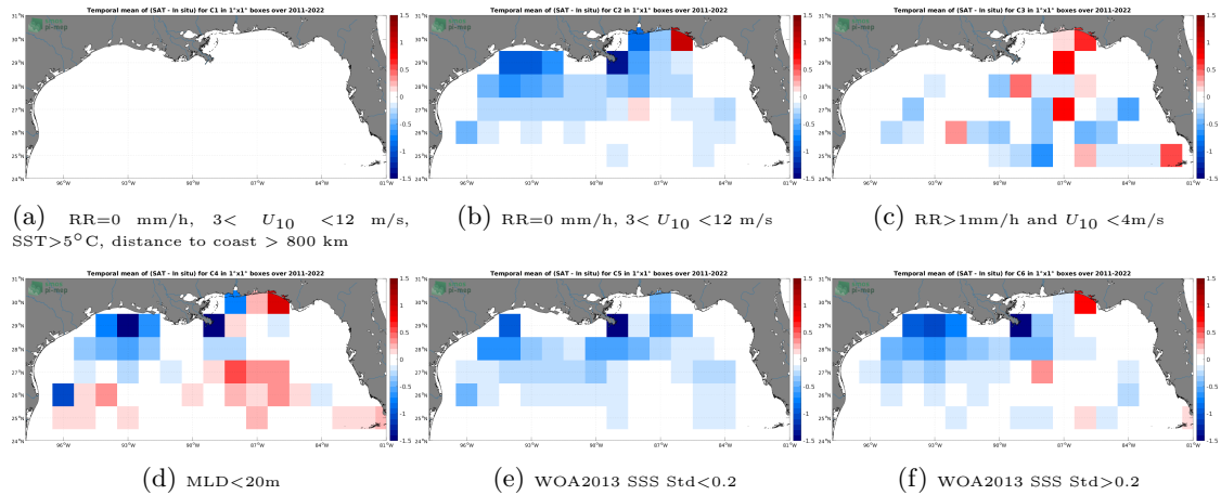
Figure 12: Temporal mean gridded over spatial boxes of size 1^{\circ}\times 1^{\circ} of \Delta\text{SSS} (SMAP SSS L4 OI v2 - 7 Days (ESR) - Argo) for 6 different subdatasets corresponding to:RR=0 mm/h, 3 < U_{10} < 12 m/s, SST > 5^{\circ}\text{C} , distance to coast > 800 km (a), RR=0 mm/h, 3 < U_{10} < 12 m/s (b), RR > 1\text{mm/h} and U_{10} < 4\text{m/s} (c),MLD < 20\text{m} (d),WOA2013 SSS Std < 0.2 (e),WOA2013 SSS Std > 0.2 (f).
