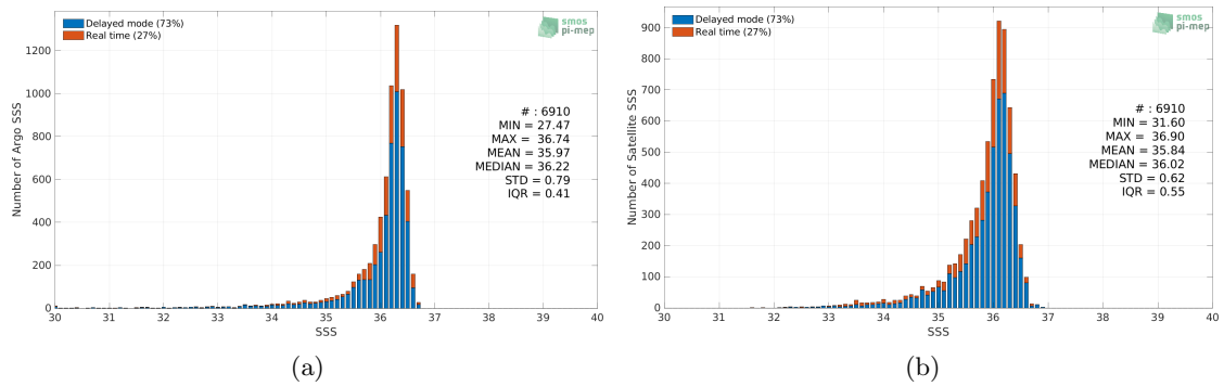
Figure 2: Histograms of SSS from Argo (a) and SMAP SSS L4 OI v2 - 7 Days (ESR) (b) considering all match-up pairs per bins of 0.1 over the Mississippi river plume Pi-MEP region and for the full satellite product period.
