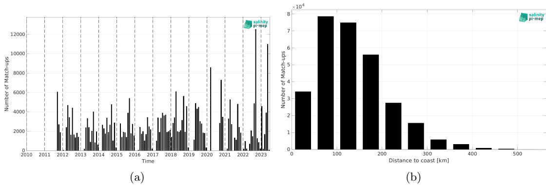
Figure 1: Number of match-ups between TSG (SAMOS) and SMAP SSS L4 OI v2 - Monthly (IPRC) SSS as a function of time (a) and as function of the distance to coast (b) over the Mississippi river plume Pi-MEP region and for the full satellite product period.
