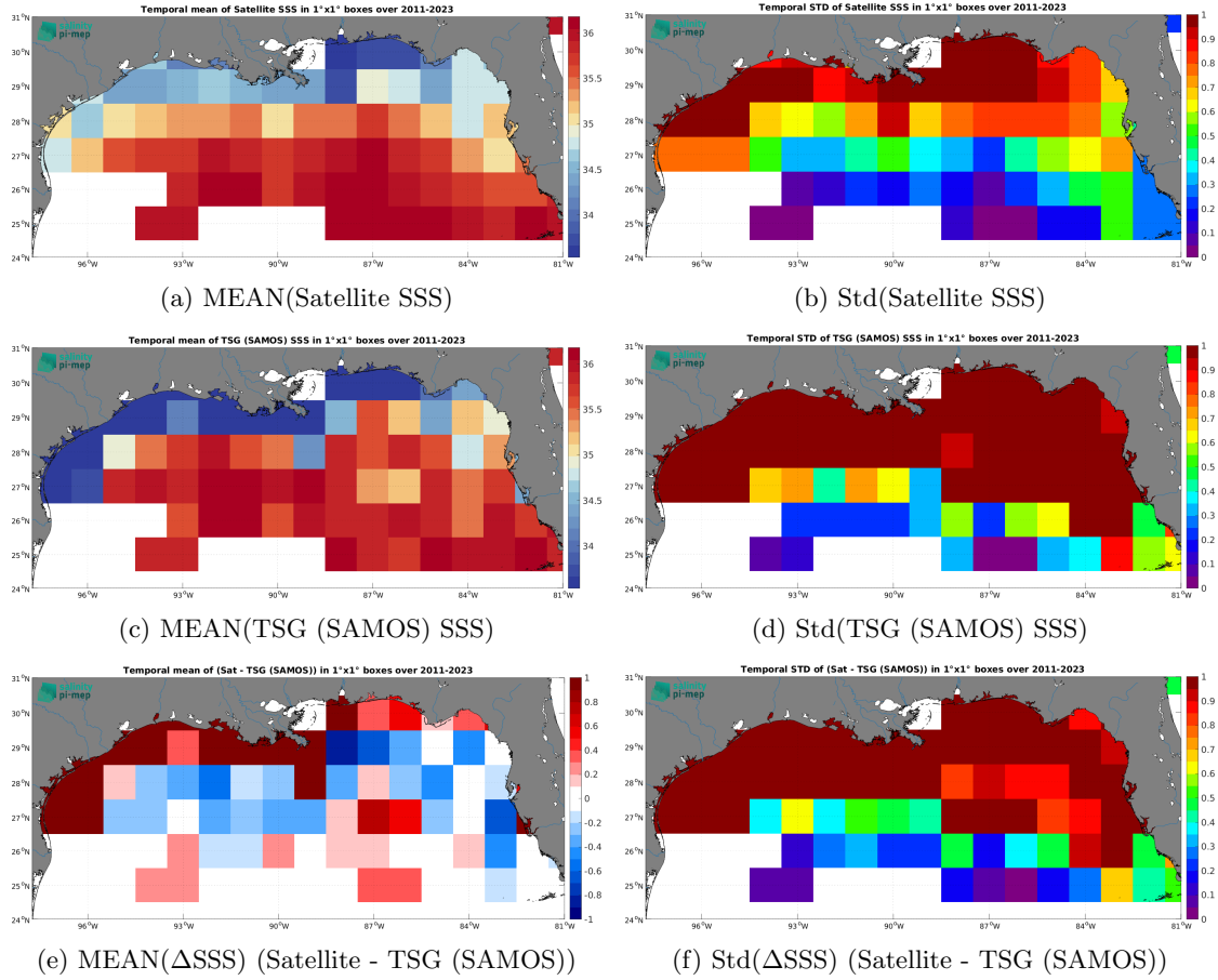
Figure 6: Temporal mean (left) and Std (right) of SSS from SMAP SSS L4 OI v2 - Monthly (IPRC) (top), TSG (SAMOS) (middle), and of \Delta\text{SSS} (Satellite - TSG (SAMOS)). Only match-up pairs are used to generate these maps.
