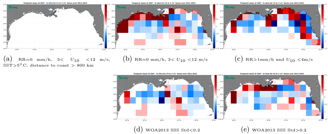
Figure 12: Temporal mean gridded over spatial boxes of size 1^{\circ}\times 1^{\circ} of \Delta\text{SSS} (SMAP SSS L4 OI v2 - Monthly (IPRC) - TSG (SAMOS)) for 5 different subdatasets corresponding to:RR=0 mm/h, 3 < U_{10} < 12 m/s, SST >5^{\circ}\text{C} , distance to coast > 800 km (a), RR=0 mm/h, 3 < U_{10} < 12 m/s (b), RR >1 mm/h and U_{10} < 4 m/s (c), WOA2013 SSS Std <0.2 (d), WOA2013 SSS Std >0.2 (e).
