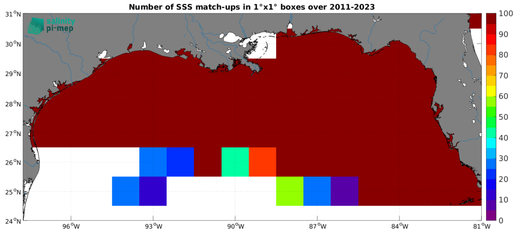
Figure 4: Number of SSS match-ups between TSG (SAMOS) SSS and the SMAP SSS L4 OI v2 - Monthly (IPRC) SSS product for the Mississippi river plume Pi-MEP region over 1^\circ \times 1^\circ boxes and for the full satellite product period.
