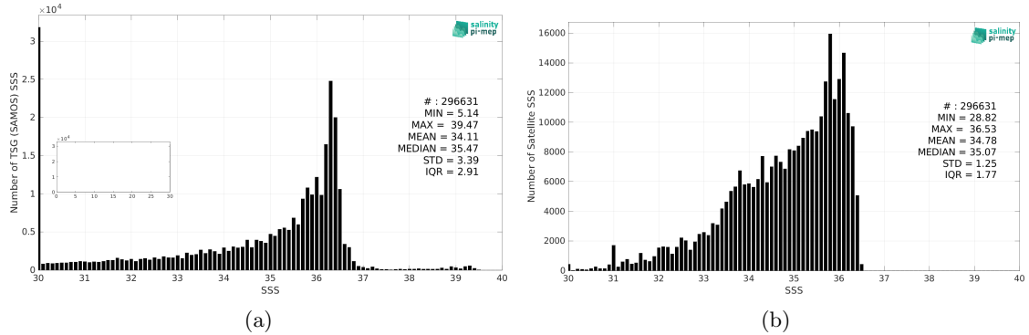
Figure 2: Histograms of SSS from TSG (SAMOS) (a) and SMAP SSS L4 OI v2 - Monthly (IPRC) (b) considering all match-up pairs per bins of 0.1 over the Mississippi river plume Pi-MEP region and for the full satellite product period.
