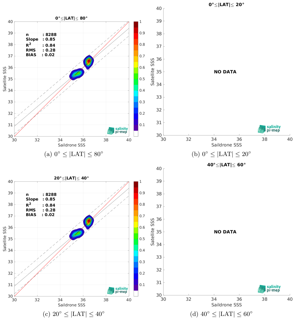
Figure 10: Contour maps of the concentration of SMAP SSS L3 v6 - 8-Day running (RSS) SSS (y-axis) versus Saïldrone SSS (x-axis) at match-up pairs for different latitude bands. For each plot, the red line shows x=y . The black thin and dashed lines indicate a linear fit through the data cloud and the \pm 95\% confidence levels, respectively. The number match-up pairs n , the slope and R^2 coefficient of the linear fit, the root mean square (RMS) and the mean bias between satellite and in situ data are indicated for each latitude band in each plots.
