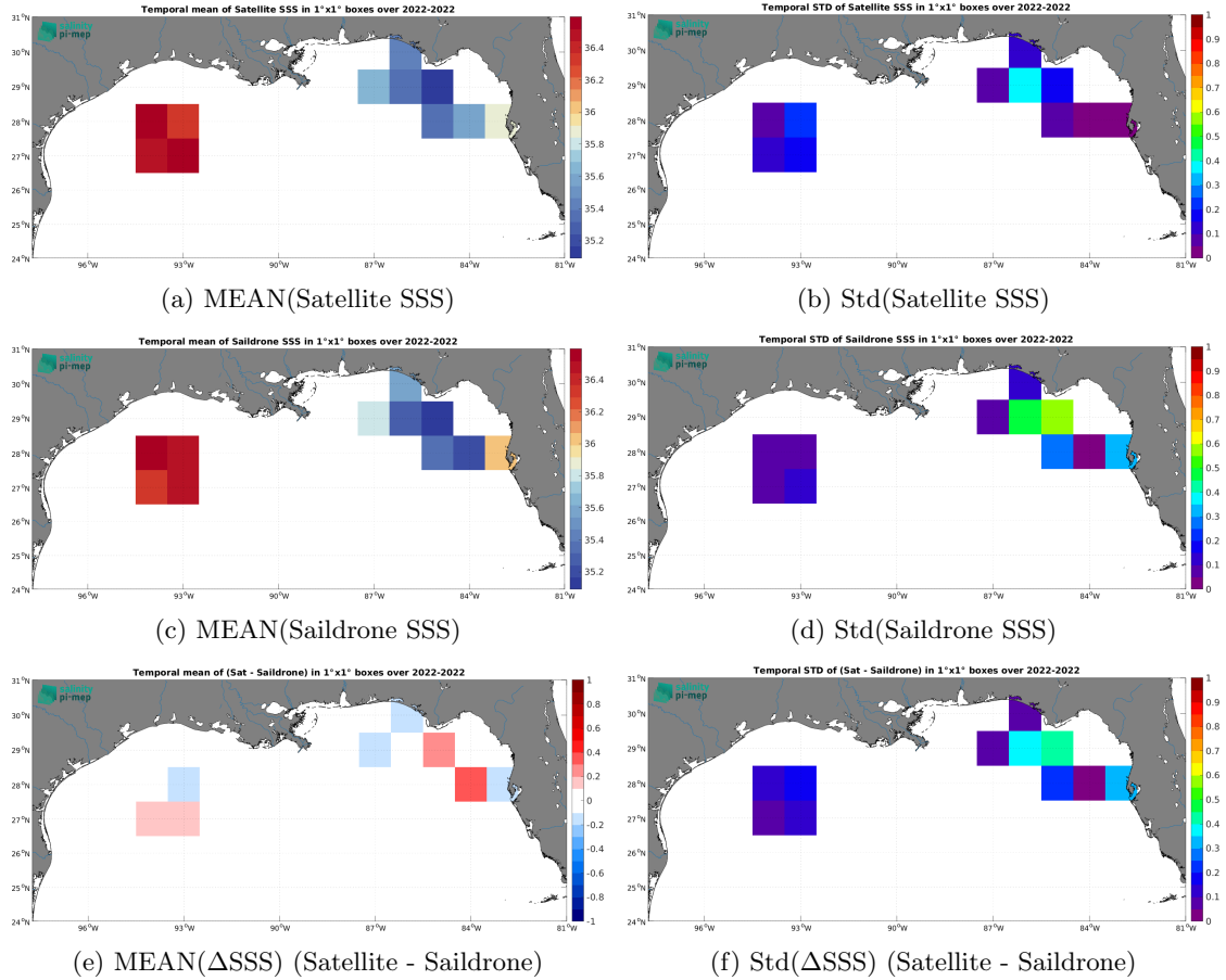
Figure 7: Temporal mean (left) and Std (right) of SSS from SMAP SSS L3 v6 - 8-Day running (RSS) (top), Saildrone (middle), and of \Delta SSS (Satellite - Saildrone). Only match-up pairs are used to generate these maps.
