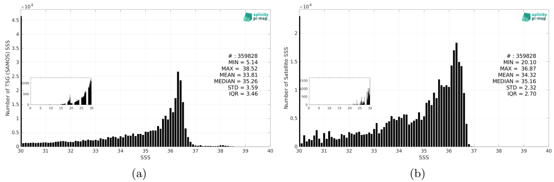
Figure 3: Histograms of SSS from TSG (SAMOS) (a) and SMAP SSS L3 v6 - Monthly (RSS) (b) considering all match-up pairs per bins of 0.1 over the Mississippi river plume Pi-MEP region and for the full satellite product period.
