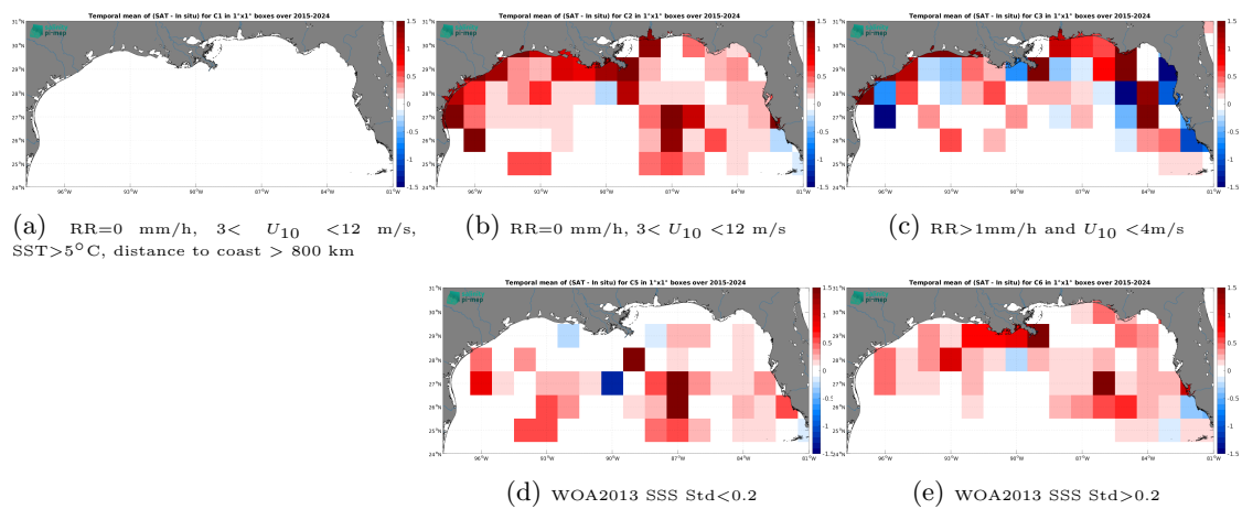
Figure 14: Temporal mean gridded over spatial boxes of size 1^\circ \times 1^\circ of \Delta SSS (SMAP SSS L3 v6 - Monthly (RSS) - TSG (SAMOS)) for 5 different subdatasets corresponding to:RR=0 mm/h, 3 < U_{10} < 12 m/s, SST >5^\circ\text{C} , distance to coast > 800 km (a), RR=0 mm/h, 3 < U_{10} < 12 m/s (b), RR >1 mm/h and U_{10} < 4 m/s (c), WOA2013 SSS Std <0.2 (d), WOA2013 SSS Std >0.2 (e).
