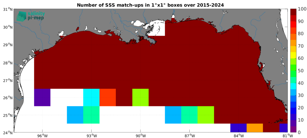
Figure 5: Number of SSS match-ups between TSG (SAMOS) SSS and the SMAP SSS L3 v6 - Monthly (RSS) SSS product for the Mississippi river plume Pi-MEP region over 1^\circ \times 1^\circ boxes and for the full satellite product period.
