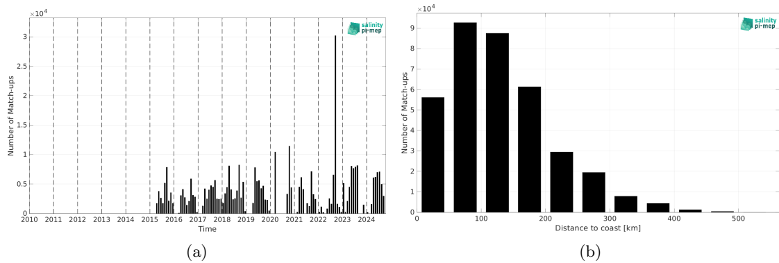
Figure 2: Number of match-ups between TSG (SAMOS) and SMAP SSS L3 v6 - Monthly (RSS) SSS as a function of time (a) and as function of the distance to coast (b) over the Mississippi river plume Pi-MEP region and for the full satellite product period.
