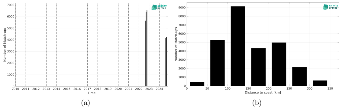
Figure 2: Number of match-ups between Sairdrone and SMAP SSS L3 v6 - Monthly (RSS) SSS as a function of time (a) and as function of the distance to coast (b) over the Mississippi river plume Pi-MEP region and for the full satellite product period.
