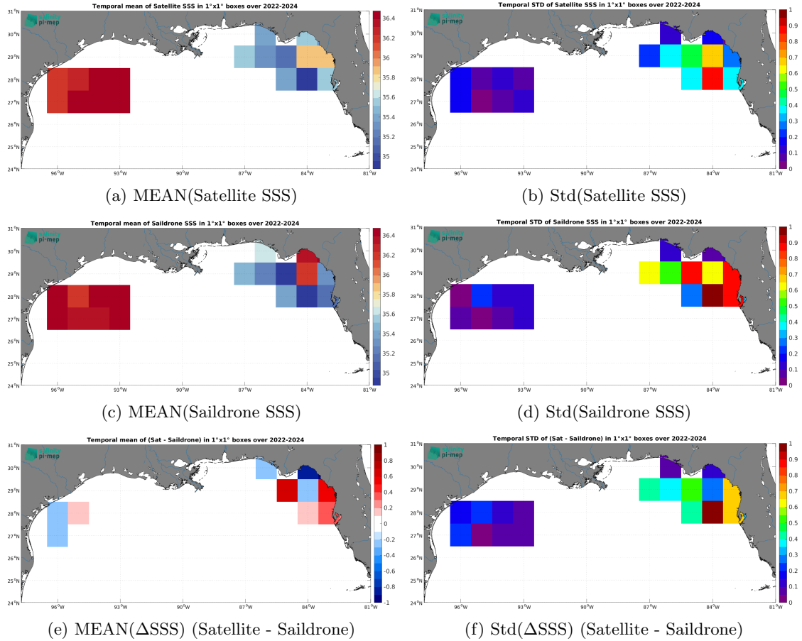
Figure 7: Temporal mean (left) and Std (right) of SSS from SMAP SSS L3 v6 - Monthly (RSS) (top), Sairdron (middle), and of \Delta SSS (Satellite - Sairdron). Only match-up pairs are used to generate these maps.
