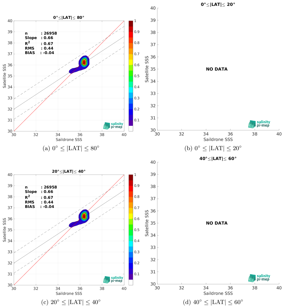
Figure 10: Contour maps of the concentration of SMAP SSS L3 v6 - Monthly (RSS) SSS (y-axis) versus Saildrone SSS (x-axis) at match-up pairs for different latitude bands. For each plot, the red line shows x=y . The black thin and dashed lines indicate a linear fit through the data cloud and the \pm 95\% confidence levels, respectively. The number match-up pairs n , the slope and R^2 coefficient of the linear fit, the root mean square (RMS) and the mean bias between satellite and in situ data are indicated for each latitude band in each plots.
