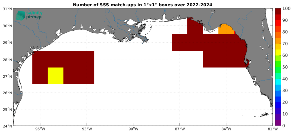
Figure 5: Number of SSS match-ups between Saildrone SSS and the SMAP SSS L3 v6 - Monthly (RSS) SSS product for the Mississippi river plume Pi-MEP region over 1^\circ \times 1^\circ boxes and for the full satellite product period.
