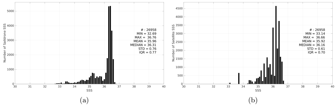
Figure 3: Histograms of SSS from Saildrone (a) and SMAP SSS L3 v6 - Monthly (RSS) (b) considering all match-up pairs per bins of 0.1 over the Mississippi river plume Pi-MEP region and for the full satellite product period.
