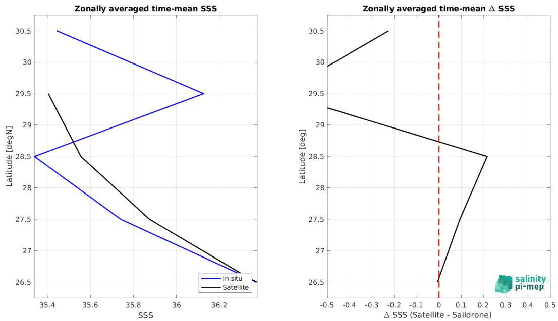
Figure 9: Left panel: Zonal mean SSS from SMAP SSS L3 v6 - Monthly (RSS) satellite product (black) and from Sairdron (blue). Right panel: Zonal mean of \Delta SSS (Satellite - Sairdron) for all the collected Pi-MEP match-up pairs estimated over the full satellite product period.
