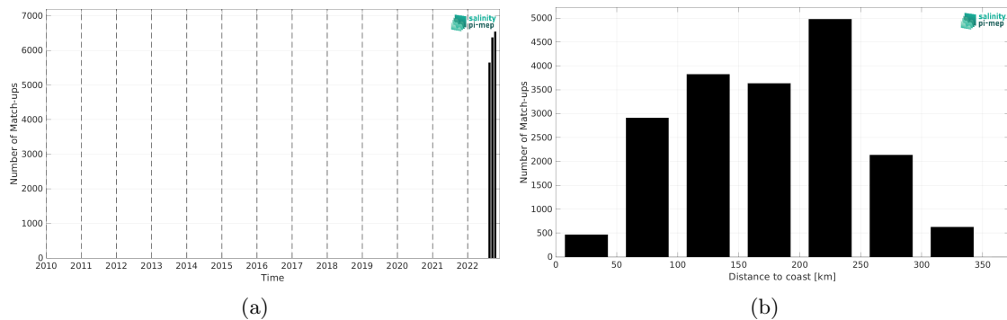
Figure 2: Number of match-ups between Saildrone and SMAP SSS L3 v6 - Monthly (RSS) SSS as a function of time (a) and as function of the distance to coast (b) over the Mississippi river plume Pi-MEP region and for the full satellite product period.
