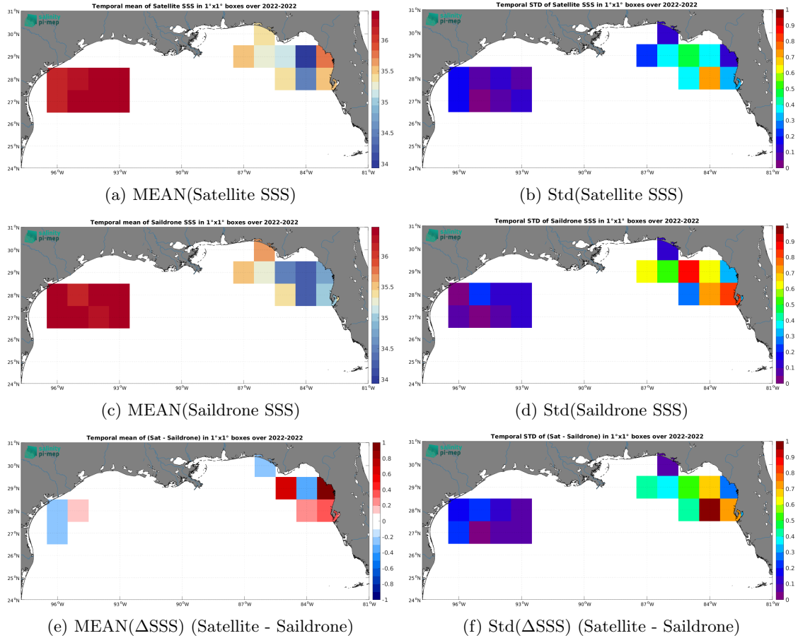
Figure 7: Temporal mean (left) and Std (right) of SSS from SMAP SSS L3 v6 - Monthly (RSS) (top), Sairdrone (middle), and of \Delta SSS (Satellite - Sairdrone). Only match-up pairs are used to generate these maps.
