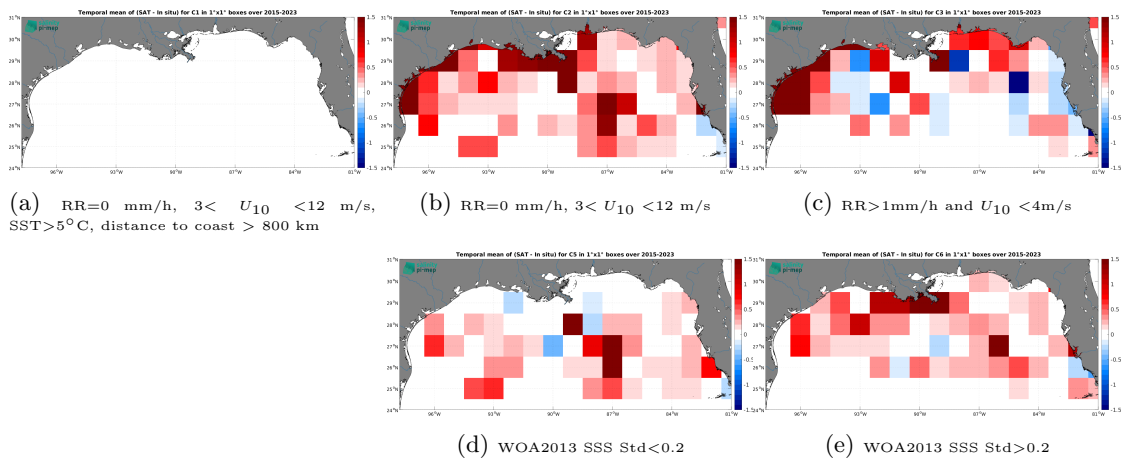
Figure 14: Temporal mean gridded over spatial boxes of size 1^\circ \times 1^\circ of \Delta SSS (SMAP SSS L3 v5.3 - 8-Day running (RSS) - TSG (SAMOS)) for 5 different subdatasets corresponding to:RR=0 mm/h, 3 < U_{10} < 12 m/s, SST > 5°C, distance to coast > 800 km (a), RR=0 mm/h, 3 < U_{10} < 12 m/s (b), RR > 1mm/h and U_{10} < 4 m/s (c), WOA2013 SSS Std < 0.2 (d), WOA2013 SSS Std > 0.2 (e).
