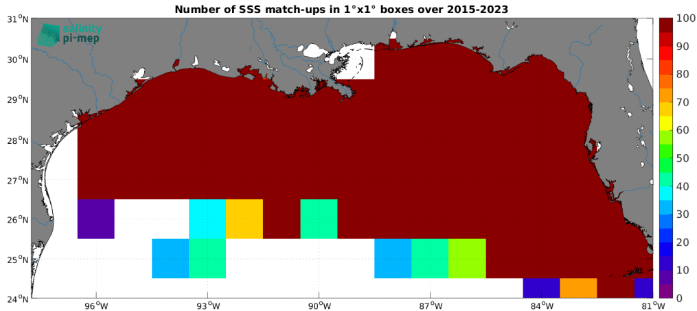
Figure 5: Number of SSS match-ups between TSG (SAMOS) SSS and the SMAP SSS L3 v5.3 - 8-Day running (RSS) SSS product for the Mississippi river plume Pi-MEP region over 1^\circ \times 1^\circ boxes and for the full satellite product period.
