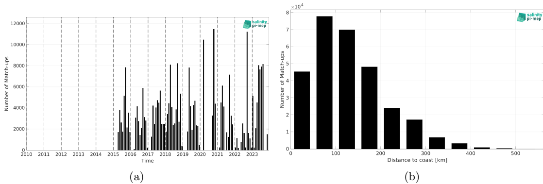
Figure 2: Number of match-ups between TSG (SAMOS) and SMAP SSS L3 v5.3 - 8-Day running (RSS) SSS as a function of time (a) and as function of the distance to coast (b) over the Mississippi river plume Pi-MEP region and for the full satellite product period.
