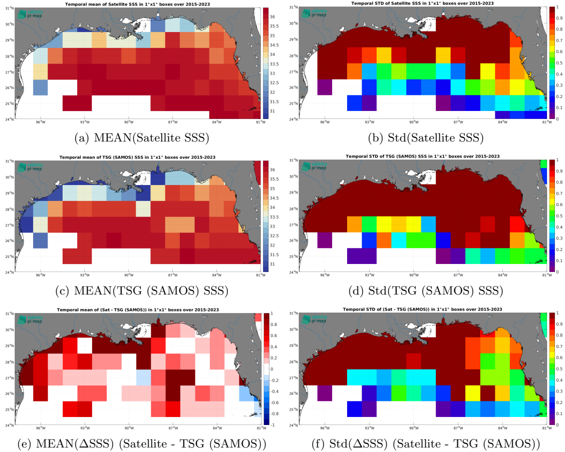
Figure 7: Temporal mean (left) and Std (right) of SSS from SMAP SSS L3 v5.3 - 8-Day running (RSS) (top), TSG (SAMOS) (middle), and of \Delta\text{SSS} (Satellite - TSG (SAMOS)). Only match-up pairs are used to generate these maps.
