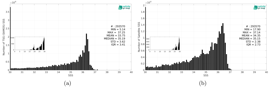
Figure 3: Histograms of SSS from TSG (SAMOS) (a) and SMAP SSS L3 v5.3 - 8-Day running (RSS) (b) considering all match-up pairs per bins of 0.1 over the Mississippi river plume Pi-MEP region and for the full satellite product period.
