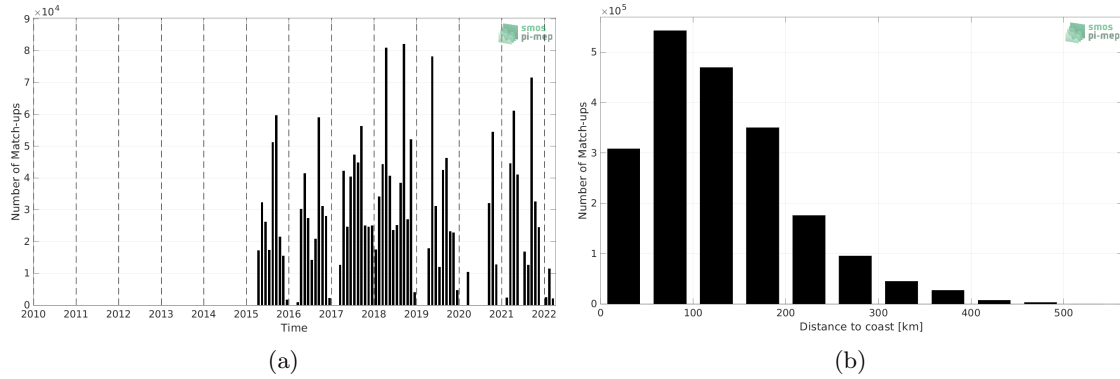
Figure 1: Number of match-ups between TSG (SAMOS) and SMAP SSS L3 v5 - 8-Day running (RSS) SSS as a function of time (a) and as function of the distance to coast (b) over the Mississippi river plume Pi-MEP region and for the full satellite product period.
