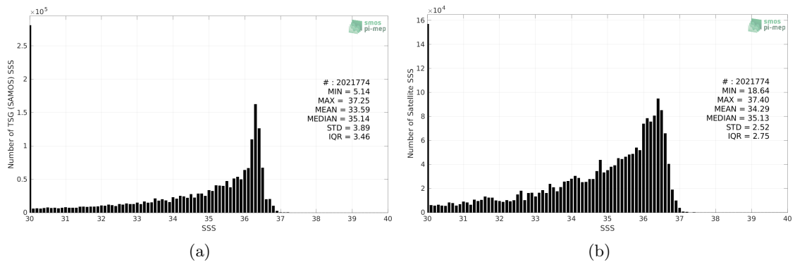
Figure 2: Histograms of SSS from TSG (SAMOS) (a) and SMAP SSS L3 v5 - 8-Day running (RSS) (b) considering all match-up pairs per bins of 0.1 over the Mississippi river plume Pi-MEP region and for the full satellite product period.
