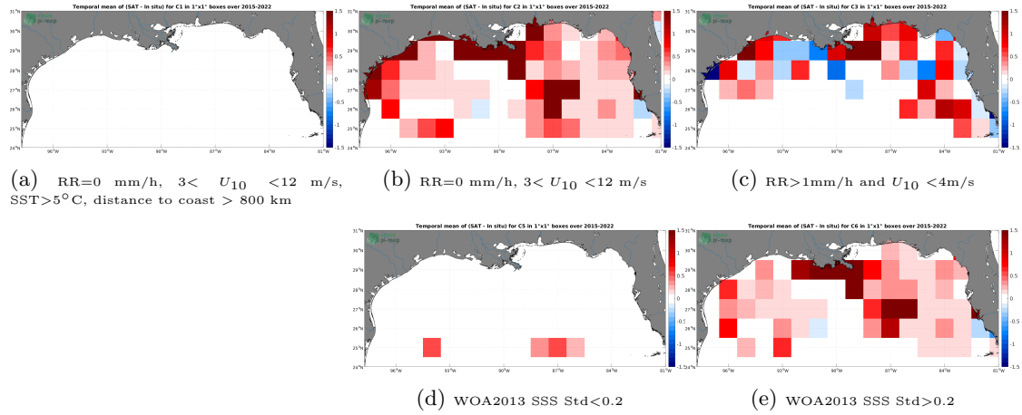
Figure 12: Temporal mean gridded over spatial boxes of size 1^{\circ}\times 1^{\circ} of \Delta\text{SSS} (SMAP SSS L3 v5 - 8-Day running (RSS) - TSG (SAMOS)) for 5 different subdatasets corresponding to:RR=0 mm/h, 3 < U_{10} < 12 m/s, SST >5^{\circ}\text{C} , distance to coast > 800 km (a), RR=0 mm/h, 3 < U_{10} < 12 m/s (b), RR >1 mm/h and U_{10} < 4 m/s (c), WOA2013 SSS Std <0.2 (d), WOA2013 SSS Std >0.2 (e).
