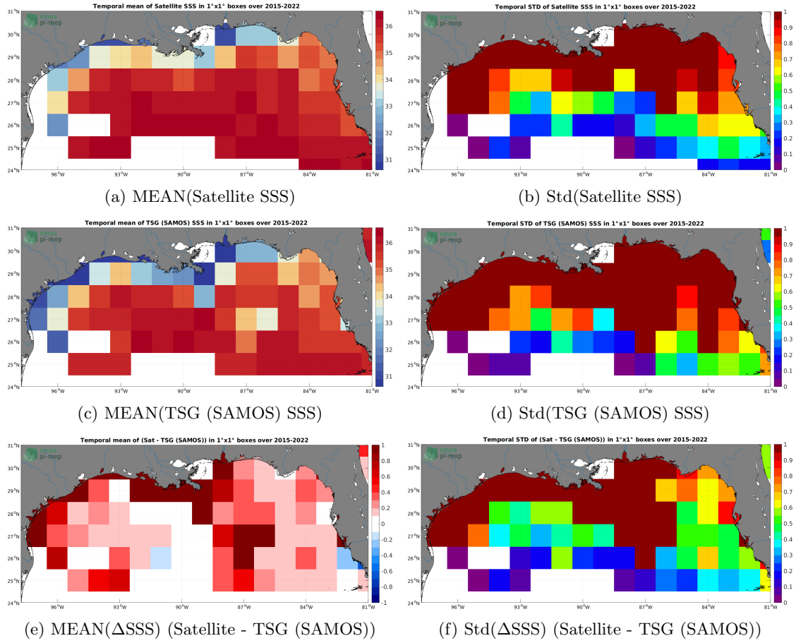
Figure 6: Temporal mean (left) and Std (right) of SSS from SMAP SSS L3 v5 - 8-Day running (RSS) (top), TSG (SAMOS) (middle), and of \Delta SSS (Satellite - TSG (SAMOS)). Only match-up pairs are used to generate these maps.
