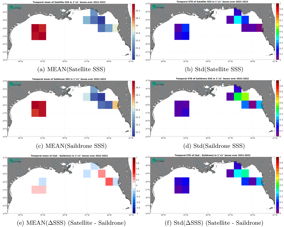
Figure 6: Temporal mean (left) and Std (right) of SSS from SMAP SSS L3 v5 - 8-Day running (RSS) (top), Saildrone (middle), and of \Delta\text{SSS} (Satellite - Saildrone). Only match-up pairs are used to generate these maps.
