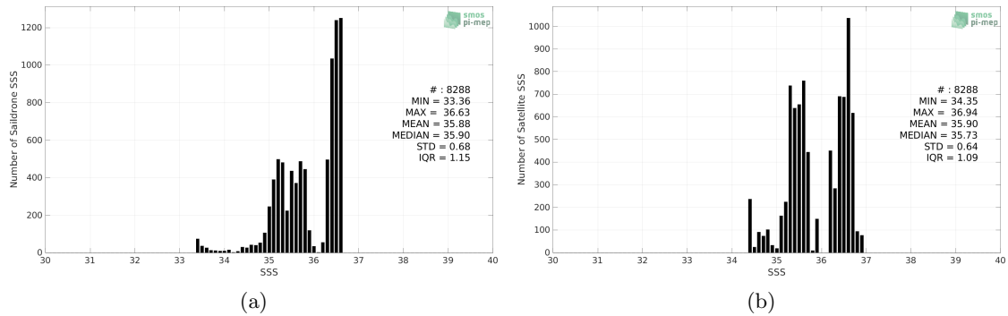
Figure 2: Histograms of SSS from Saildrone (a) and SMAP SSS L3 v5 - 8-Day running (RSS) (b) considering all match-up pairs per bins of 0.1 over the Mississippi river plume Pi-MEP region and for the full satellite product period.
