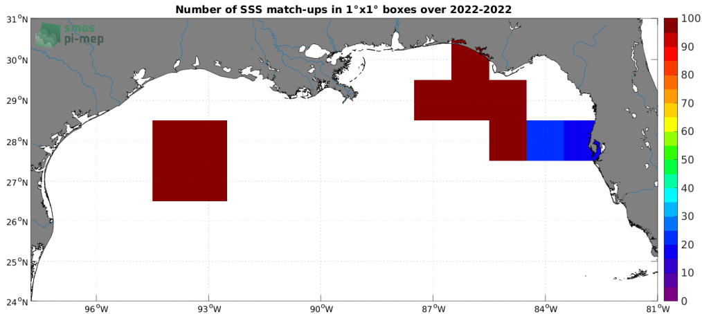
Figure 4: Number of SSS match-ups between Sairdrone SSS and the SMAP SSS L3 v5 - 8-Day running (RSS) SSS product for the Mississippi river plume Pi-MEP region over 1^\circ \times 1^\circ boxes and for the full satellite product period.
