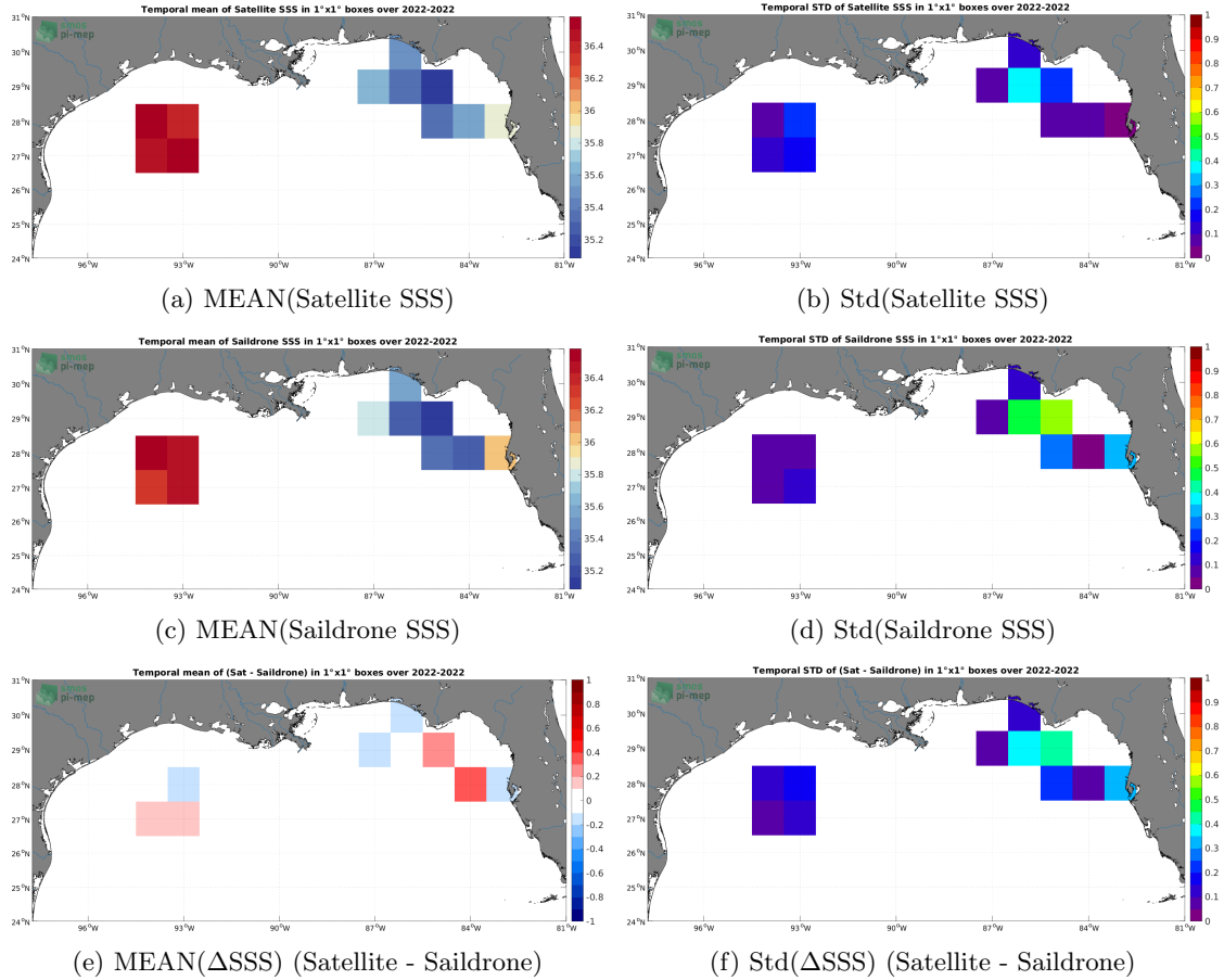
Figure 6: Temporal mean (left) and Std (right) of SSS from SMAP SSS L3 v5 - 8-Day running (RSS) (top), Saildrone (middle), and of \Delta SSS (Satellite - Saildrone). Only match-up pairs are used to generate these maps.
