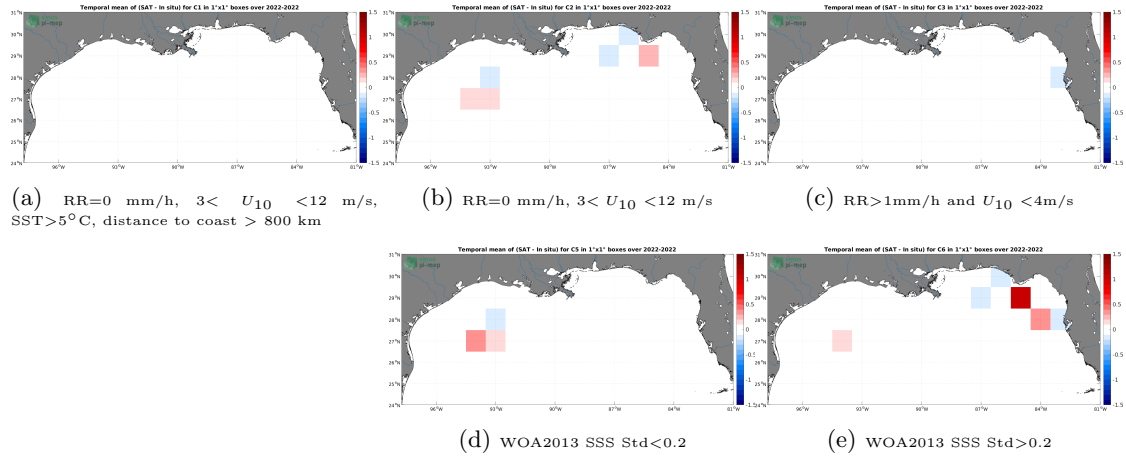
Figure 12: Temporal mean gridded over spatial boxes of size 1^{\circ}\times 1^{\circ} of \Delta\text{SSS} (SMAP SSS L3 v5 - 8-Day running (RSS) - Saildrone) for 5 different subdatasets corresponding to:RR=0 mm/h, 3 < U_{10} < 12 m/s, SST >5^{\circ}\text{C} , distance to coast > 800 km (a), RR=0 mm/h, 3 < U_{10} < 12 m/s (b), RR >1 mm/h and U_{10} < 4 m/s (c), WOA2013 SSS Std <0.2 (d), WOA2013 SSS Std >0.2 (e).
