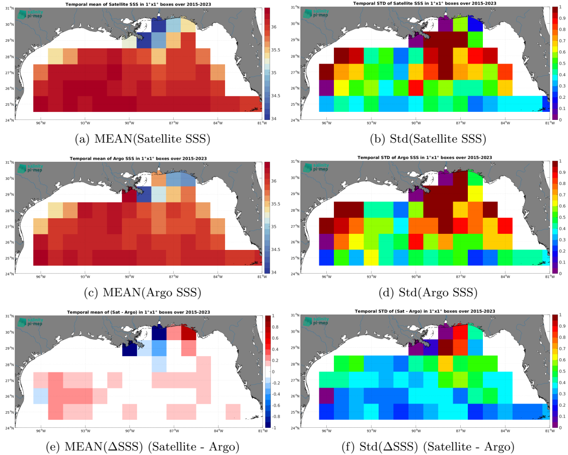
Figure 6: Temporal mean (left) and Std (right) of SSS from SMAP SSS L3 v5 - 8-Day running (RSS) (top), Argo (middle), and of \Delta\text{SSS} (Satellite - Argo). Only match-up pairs are used to generate these maps.
