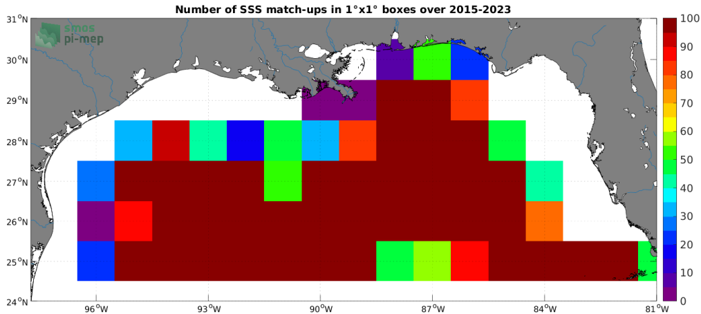
Figure 4: Number of SSS match-ups between Argo SSS and the SMAP SSS L3 v5 - 8-Day running (RSS) SSS product for the Mississippi river plume Pi-MEP region over 1^\circ \times 1^\circ boxes and for the full satellite product period.
