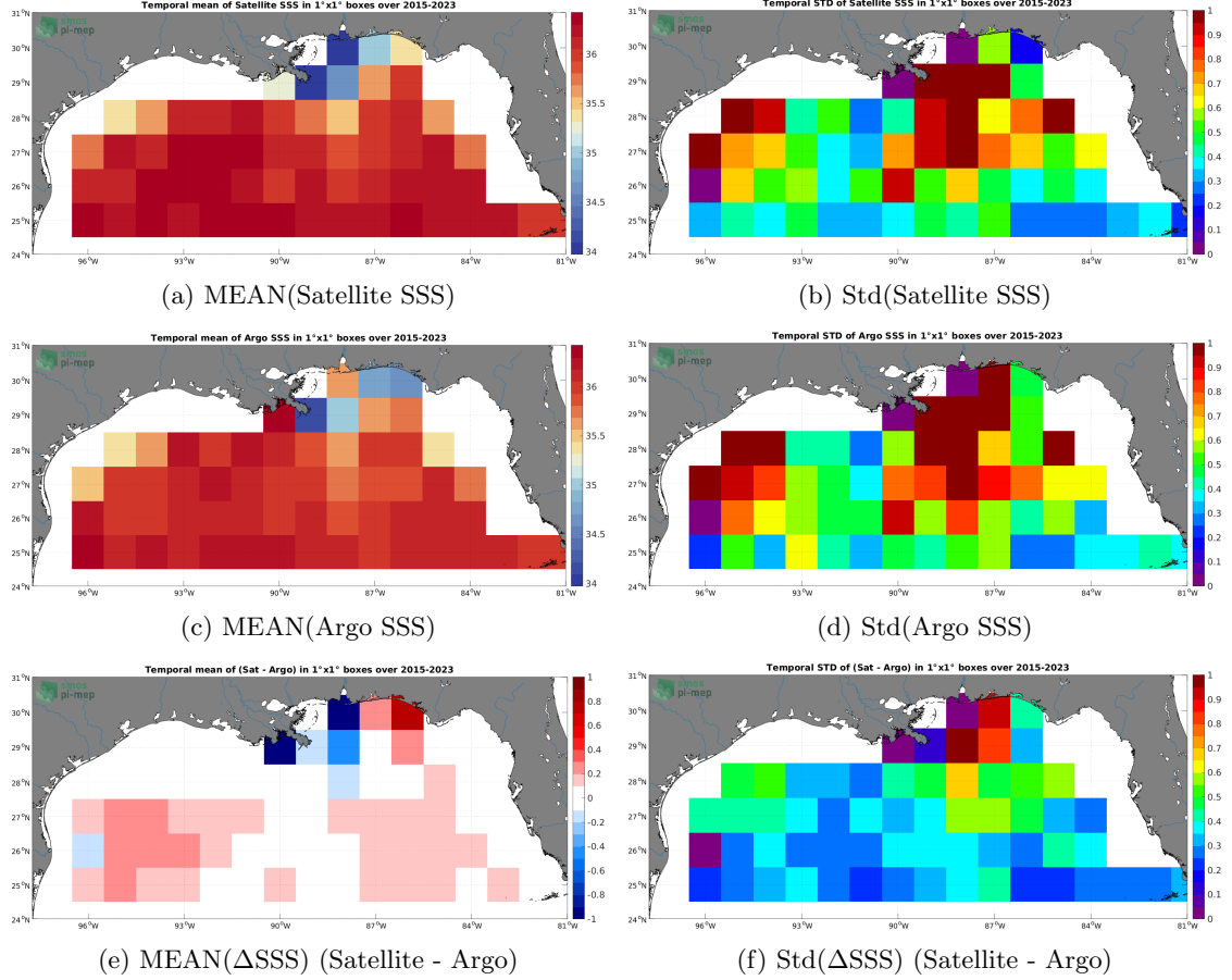
Figure 6: Temporal mean (left) and Std (right) of SSS from SMAP SSS L3 v5 - 8-Day running (RSS) (top), Argo (middle), and of \Delta\text{SSS} (Satellite - Argo). Only match-up pairs are used to generate these maps.
