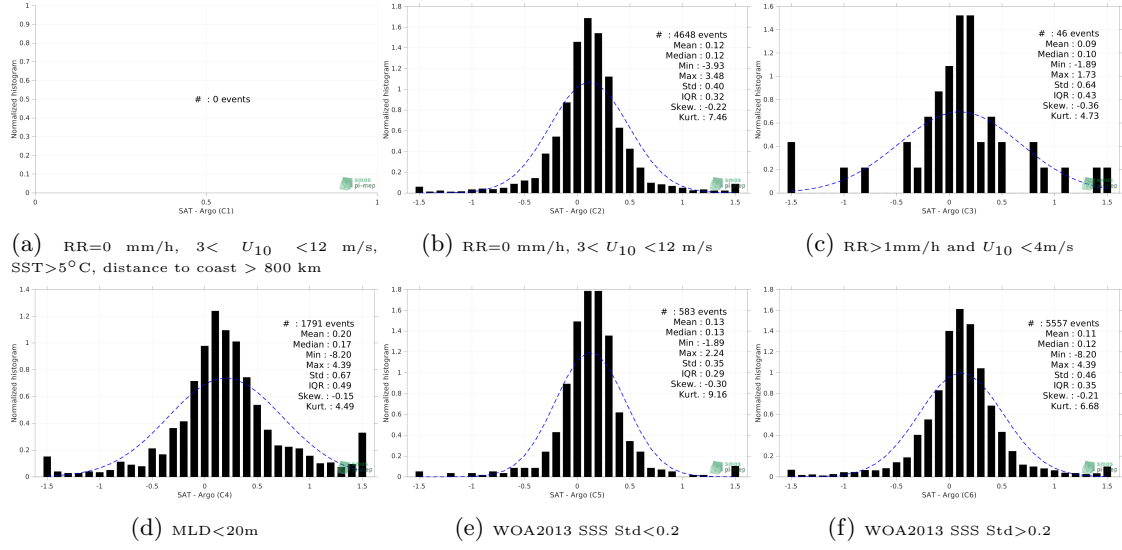
Figure 13: Normalized histogram of \Delta\text{SSS} (SMAP SSS L3 v5 - 8-Day running (RSS) - Argo) for 6 different subdatasets corresponding to: RR=0 mm/h, 3 < U_{10} < 12 m/s, SST>5°C, distance to coast > 800 km (a), RR=0 mm/h, 3 < U_{10} < 12 m/s (b), RR>1mm/h and U_{10} < 4 m/s (c), MLD<20m (d), WOA2013 SSS Std<0.2 (e), WOA2013 SSS Std>0.2 (f).
