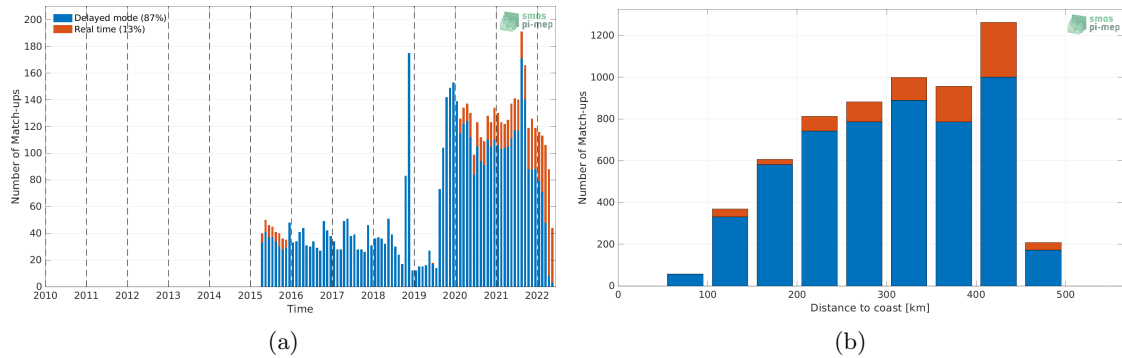
Figure 1: Number of match-ups between Argo and SMAP SSS L3 v5 - 8-Day running (RSS) SSS as a function of time (a) and as function of the distance to coast (b) over the Mississippi river plume Pi-MEP region and for the full satellite product period.
