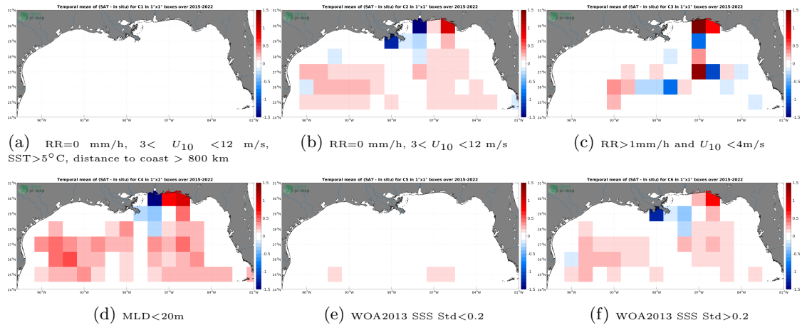
Figure 12: Temporal mean gridded over spatial boxes of size 1^{\circ}\times 1^{\circ} of \Delta\text{SSS} (SMAP SSS L3 v5 - 8-Day running (RSS) - Argo) for 6 different subdatasets corresponding to:RR=0 mm/h, 3 < U_{10} < 12 m/s, SST > 5^{\circ}\text{C} , distance to coast > 800 km (a), RR=0 mm/h, 3 < U_{10} < 12 m/s (b), RR > 1\text{mm/h} and U_{10} < 4\text{m/s} (c),MLD < 20\text{m} (d),WOA2013 SSS Std < 0.2 (e),WOA2013 SSS Std > 0.2 (f).
