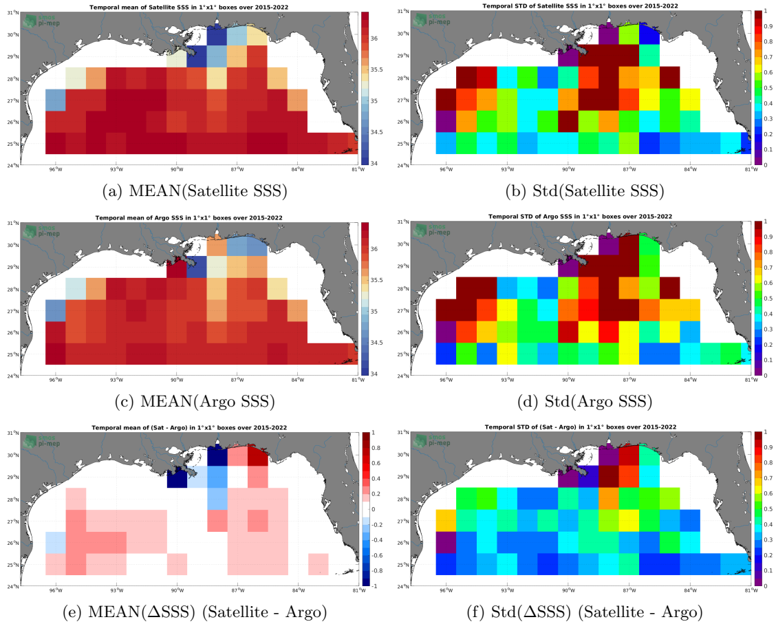
Figure 6: Temporal mean (left) and Std (right) of SSS from SMAP SSS L3 v5 - 8-Day running (RSS) (top), Argo (middle), and of \Delta SSS (Satellite - Argo). Only match-up pairs are used to generate these maps.
