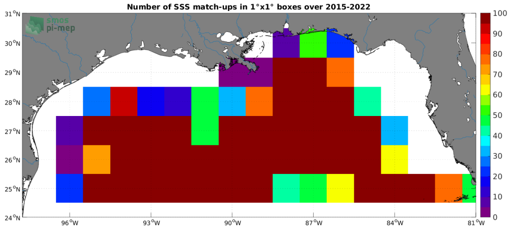
Figure 4: Number of SSS match-ups between Argo SSS and the SMAP SSS L3 v5 - 8-Day running (RSS) SSS product for the Mississippi river plume Pi-MEP region over 1^{\circ} \times 1^{\circ} boxes and for the full satellite product period.
