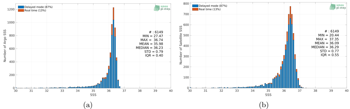
Figure 2: Histograms of SSS from Argo (a) and SMAP SSS L3 v5 - 8-Day running (RSS) (b) considering all match-up pairs per bins of 0.1 over the Mississippi river plume Pi-MEP region and for the full satellite product period.
