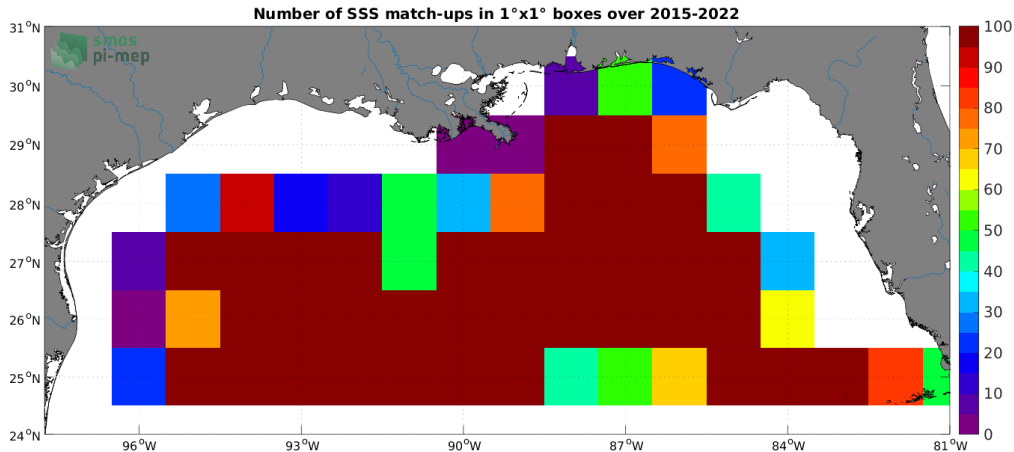
Figure 4: Number of SSS match-ups between Argo SSS and the SMAP SSS L3 v5 - Monthly (RSS) SSS product for the Mississippi river plume Pi-MEP region over 1^{\circ} \times 1^{\circ} boxes and for the full satellite product period.
