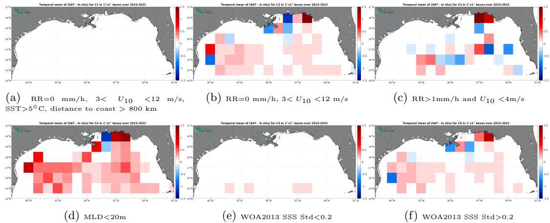
Figure 12: Temporal mean gridded over spatial boxes of size 1^{\circ}\times 1^{\circ} of \Delta\text{SSS} (SMAP SSS L3 v5 - Monthly (RSS) - Argo) for 6 different subdatasets corresponding to:RR=0 mm/h, 3 < U_{10} < 12 m/s, SST > 5^{\circ}\text{C} , distance to coast > 800 km (a), RR=0 mm/h, 3 < U_{10} < 12 m/s (b), RR > 1\text{mm/h} and U_{10} < 4\text{m/s} (c),MLD < 20\text{m} (d),WOA2013 SSS Std < 0.2 (e),WOA2013 SSS Std > 0.2 (f).
