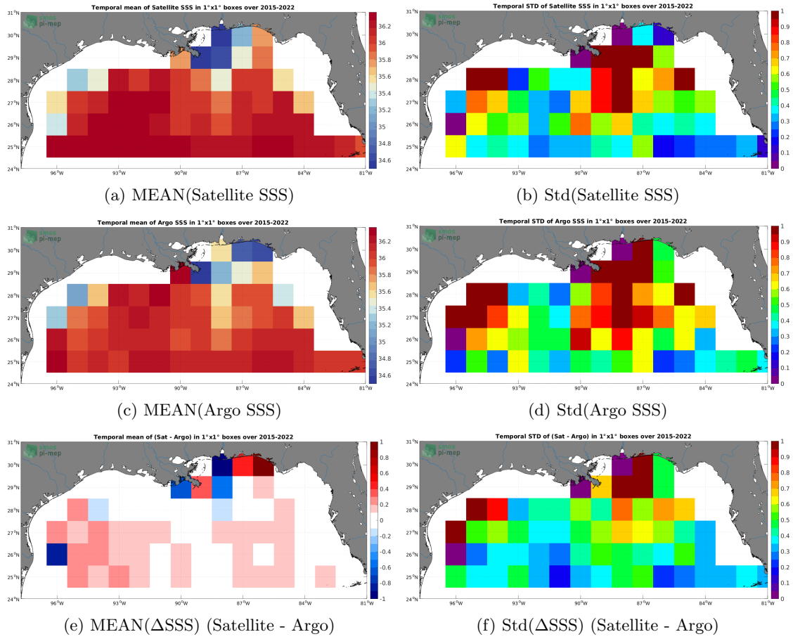
Figure 6: Temporal mean (left) and Std (right) of SSS from SMAP SSS L3 v5 - Monthly (RSS) (top), Argo (middle), and of \Delta SSS (Satellite - Argo). Only match-up pairs are used to generate these maps.
