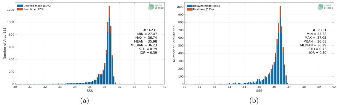
Figure 2: Histograms of SSS from Argo (a) and SMAP SSS L3 v5 - Monthly (RSS) (b) considering all match-up pairs per bins of 0.1 over the Mississippi river plume Pi-MEP region and for the full satellite product period.
