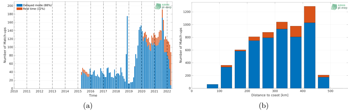
Figure 1: Number of match-ups between Argo and SMAP SSS L3 v5 - Monthly (RSS) SSS as a function of time (a) and as function of the distance to coast (b) over the Mississippi river plume Pi-MEP region and for the full satellite product period.
