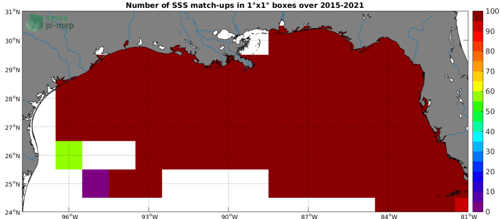
Figure 4: Number of SSS match-ups between TSG (SAMOS) SSS and the SMAP SSS L3 v4 - 8-Day running (RSS) SSS product for the Mississippi river plume Pi-MEP region over 1^\circ \times 1^\circ boxes and for the full satellite product period.
