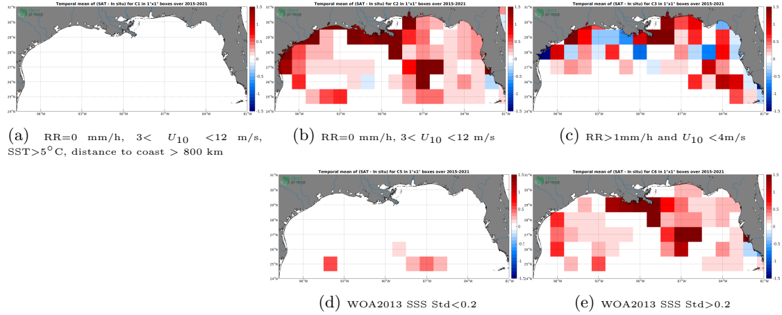
Figure 12: Temporal mean gridded over spatial boxes of size 1^{\circ}\times 1^{\circ} of \Delta\text{SSS} (SMAP SSS L3 v4 - 8-Day running (RSS) - TSG (SAMOS)) for 5 different subdatasets corresponding to: \text{RR}=0 mm/h, 3 < U_{10} < 12 m/s, \text{SST} > 5^{\circ}\text{C} , distance to coast > 800 km (a), \text{RR}=0 mm/h, 3 < U_{10} < 12 m/s (b), \text{RR} > 1 mm/h and U_{10} < 4 m/s (c), WOA2013 SSS Std < 0.2 (d), WOA2013 SSS Std > 0.2 (e).
