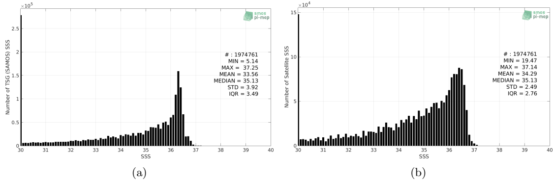
Figure 2: Histograms of SSS from TSG (SAMOS) (a) and SMAP SSS L3 v4 - 8-Day running (RSS) (b) considering all match-up pairs per bins of 0.1 over the Mississippi river plume Pi-MEP region and for the full satellite product period.
