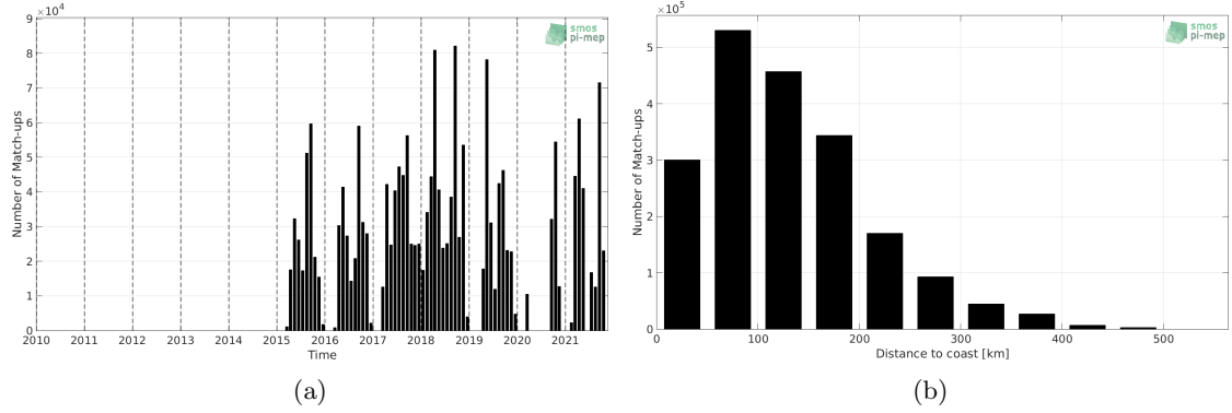
Figure 1: Number of match-ups between TSG (SAMOS) and SMAP SSS L3 v4 - 8-Day running (RSS) SSS as a function of time (a) and as function of the distance to coast (b) over the Mississippi river plume Pi-MEP region and for the full satellite product period.
