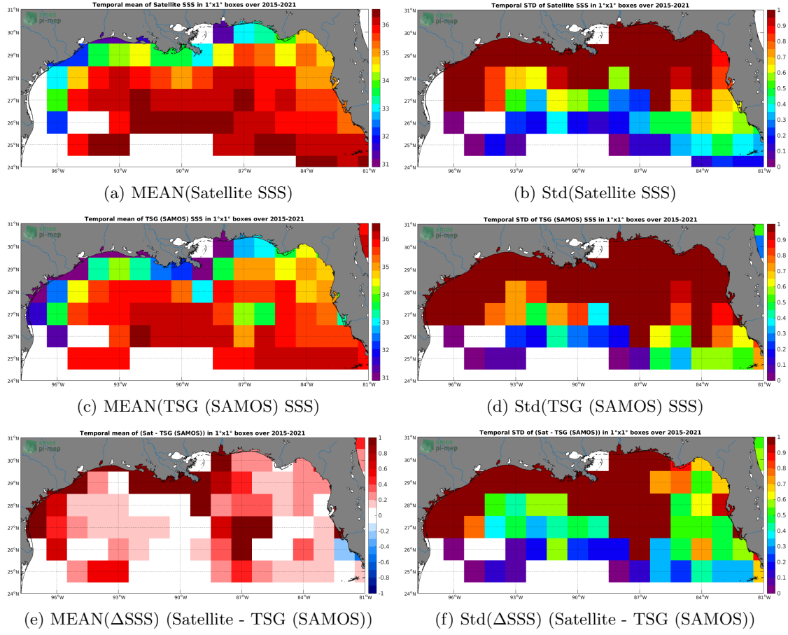
Figure 6: Temporal mean (left) and Std (right) of SSS from SMAP SSS L3 v4 - 8-Day running (RSS) (top), TSG (SAMOS) (middle), and of \Delta SSS (Satellite - TSG (SAMOS)). Only match-up pairs are used to generate these maps.
