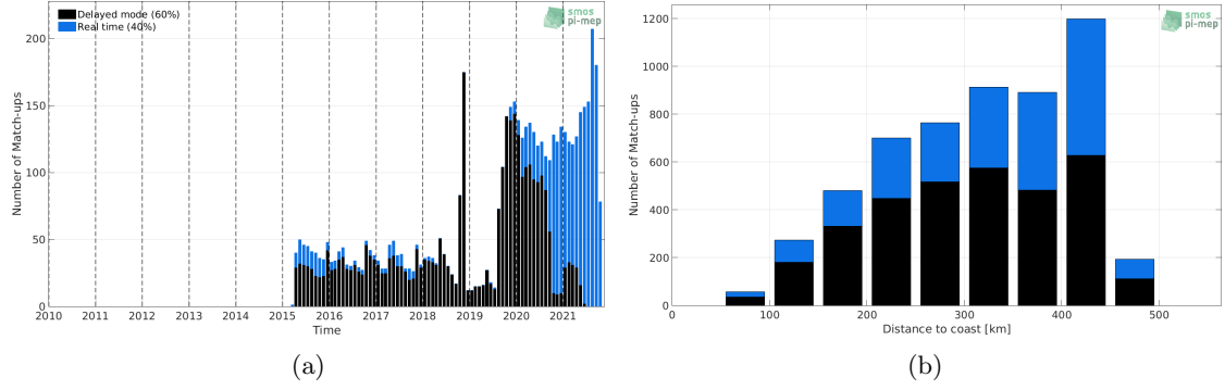
Figure 1: Number of match-ups between Argo and SMAP SSS L3 v4 - 8-Day running (RSS) SSS as a function of time (a) and as function of the distance to coast (b) over the Mississippi river plume Pi-MEP region and for the full satellite product period.
