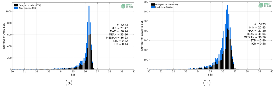
Figure 2: Histograms of SSS from Argo (a) and SMAP SSS L3 v4 - 8-Day running (RSS) (b) considering all match-up pairs per bins of 0.1 over the Mississippi river plume Pi-MEP region and for the full satellite product period.
