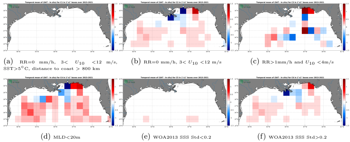
Figure 12: Temporal mean gridded over spatial boxes of size 1^{\circ} \times 1^{\circ} of \Delta\text{SSS} (SMAP SSS L3 v4 - 8-Day running (RSS) - Argo) for 6 different subdatasets corresponding to: \text{RR}=0 mm/h, 3 < U_{10} < 12 m/s, \text{SST} > 5^{\circ}\text{C} , distance to coast > 800 km (a), \text{RR}=0 mm/h, 3 < U_{10} < 12 m/s (b), \text{RR} > 1\text{mm/h} and U_{10} < 4\text{m/s} (c), \text{MLD} < 20\text{m} (d), WOA2013 SSS Std < 0.2 (e), WOA2013 SSS Std > 0.2 (f).
