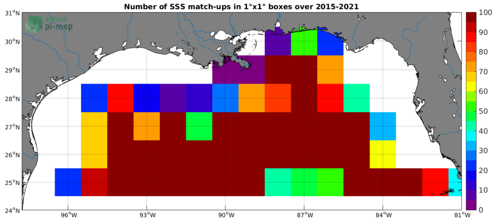
Figure 4: Number of SSS match-ups between Argo SSS and the SMAP SSS L3 v4 - 8-Day running (RSS) SSS product for the Mississippi river plume Pi-MEP region over 1^\circ \times 1^\circ boxes and for the full satellite product period.
