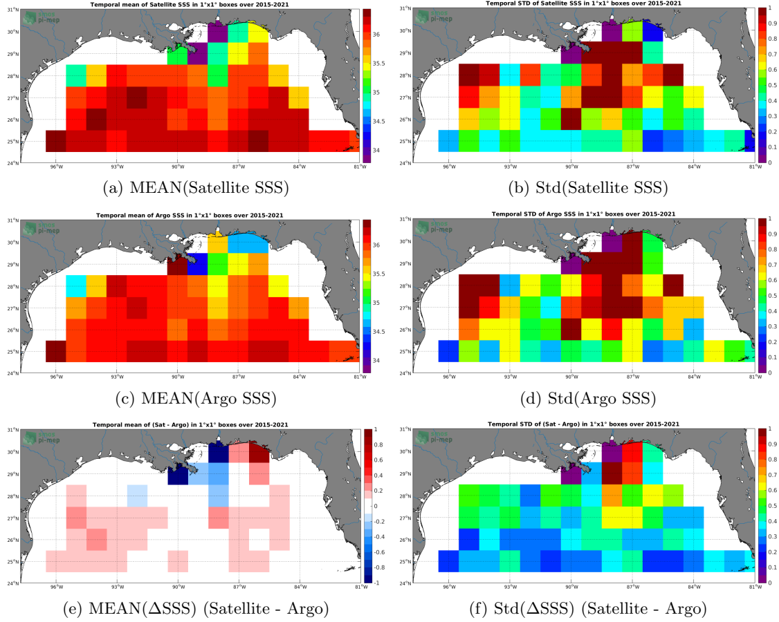
Figure 6: Temporal mean (left) and Std (right) of SSS from SMAP SSS L3 v4 - 8-Day running (RSS) (top), Argo (middle), and of \Delta SSS (Satellite - Argo). Only match-up pairs are used to generate these maps.
