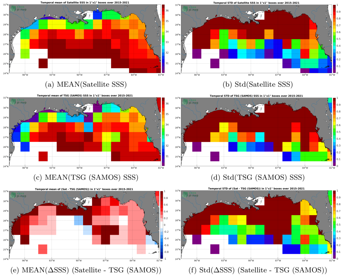
Figure 6: Temporal mean (left) and Std (right) of SSS from SMAP SSS L3 v4 - Monthly (RSS) (top), TSG (SAMOS) (middle), and of \Delta SSS (Satellite - TSG (SAMOS)). Only match-up pairs are used to generate these maps.
