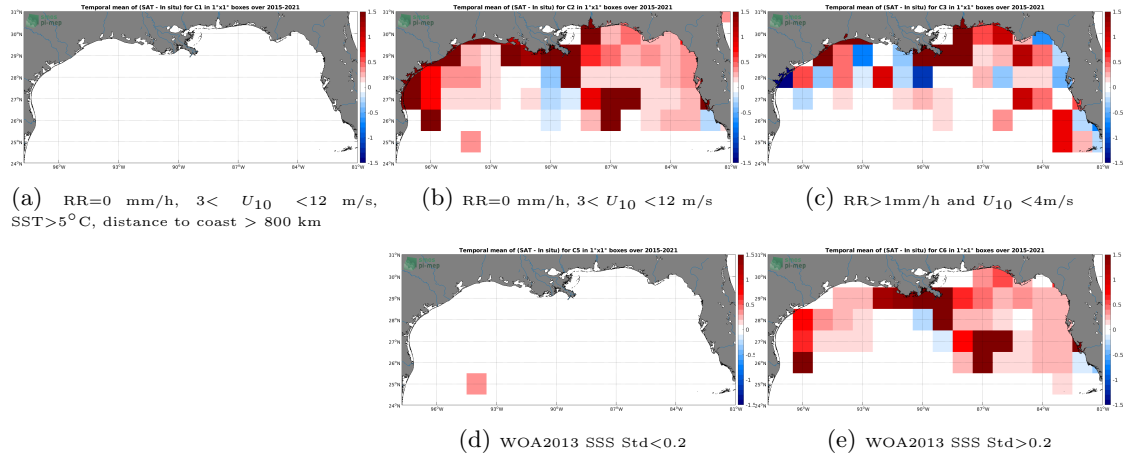
Figure 12: Temporal mean gridded over spatial boxes of size 1^{\circ}\times 1^{\circ} of \Delta\text{SSS} (SMAP SSS L3 v4 - Monthly (RSS) - TSG (SAMOS)) for 5 different subdatasets corresponding to:RR=0 mm/h, 3 < U_{10} < 12 m/s, SST >5^{\circ}\text{C} , distance to coast > 800 km (a), RR=0 mm/h, 3 < U_{10} < 12 m/s (b), RR >1 mm/h and U_{10} < 4 m/s (c), WOA2013 SSS Std <0.2 (d), WOA2013 SSS Std >0.2 (e).
