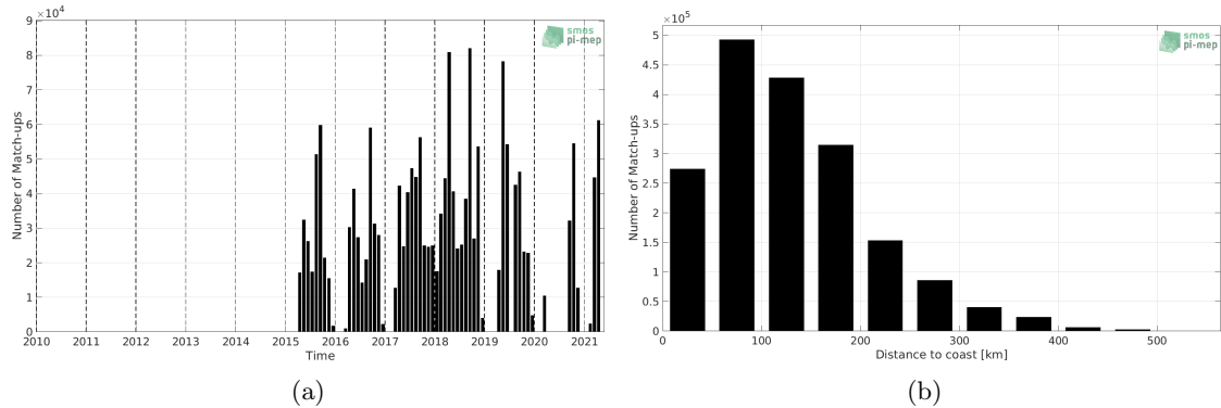
Figure 1: Number of match-ups between TSG (SAMOS) and SMAP SSS L3 v4 - Monthly (RSS) SSS as a function of time (a) and as function of the distance to coast (b) over the Mississippi river plume Pi-MEP region and for the full satellite product period.
