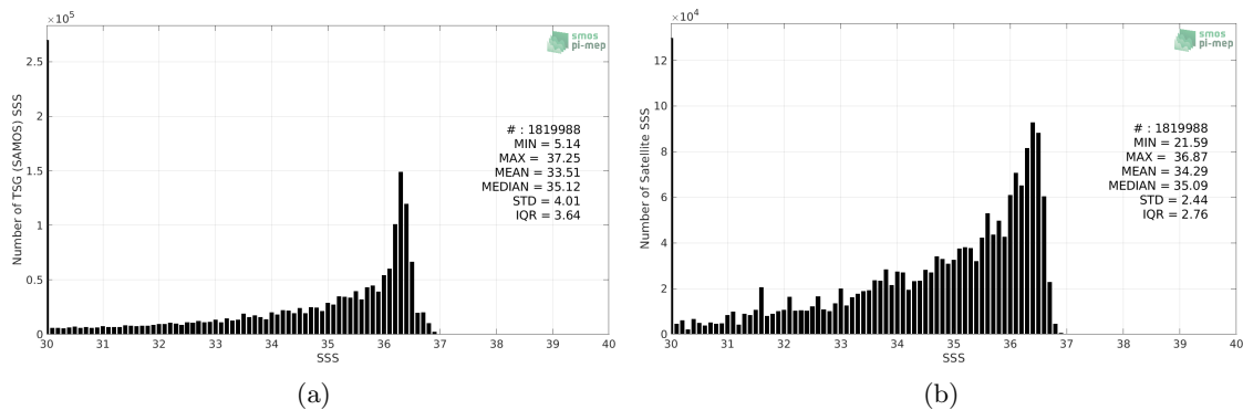
Figure 2: Histograms of SSS from TSG (SAMOS) (a) and SMAP SSS L3 v4 - Monthly (RSS) (b) considering all match-up pairs per bins of 0.1 over the Mississippi river plume Pi-MEP region and for the full satellite product period.
