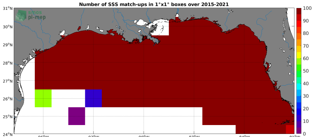
Figure 4: Number of SSS match-ups between TSG (SAMOS) SSS and the SMAP SSS L3 v4 - Monthly (RSS) SSS product for the Mississippi river plume Pi-MEP region over 1^\circ \times 1^\circ boxes and for the full satellite product period.
