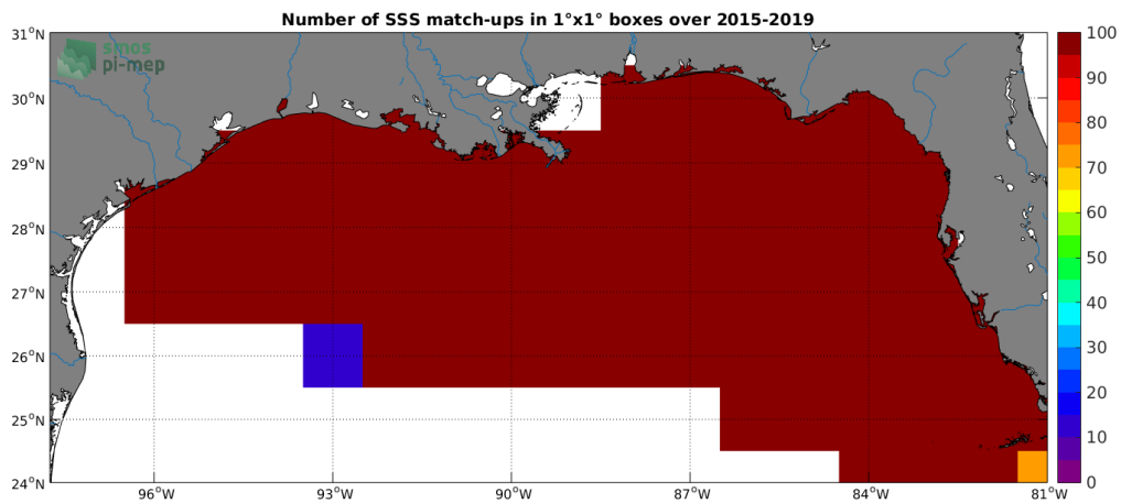
Figure 4: Number of SSS match-ups between TSG-SAMOS SSS and the SMAP-L3-RSS-V4-MONTHLY SSS product for the Mississippi river plume Pi-MEP region over 1°x1° boxes and for the full satellite product period.
