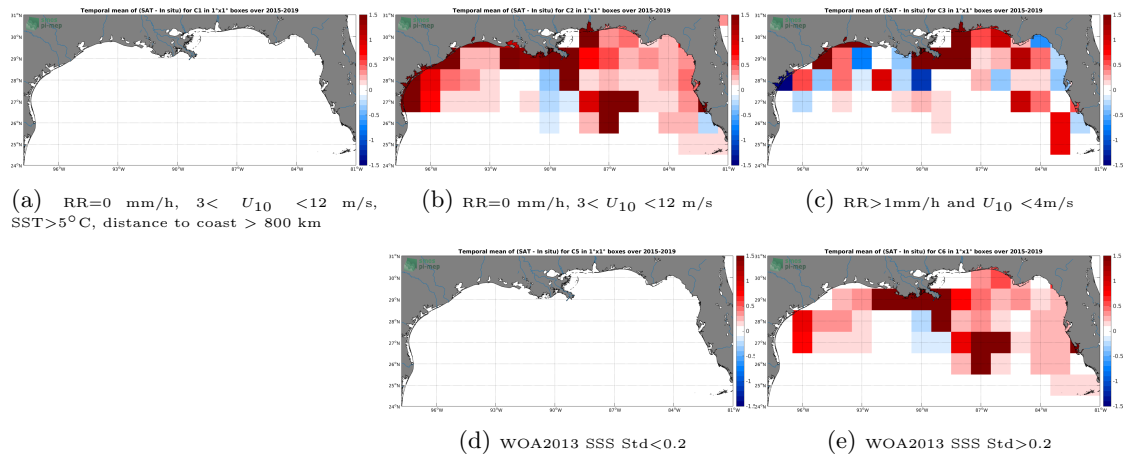
Figure 12: Temporal mean gridded over spatial boxes of size 1^{\circ}\times 1^{\circ} of \Delta\text{SSS} (SMAP-L3-RSS-V4-MONTHLY - TSG-SAMOS) for 5 different subdatasets corresponding to:RR=0 mm/h, 3 < U_{10} < 12 m/s, SST >5^{\circ}\text{C} , distance to coast > 800 km (a), RR=0 mm/h, 3 < U_{10} < 12 m/s (b), RR >1 mm/h and U_{10} < 4 m/s (c), WOA2013 SSS Std <0.2 (d), WOA2013 SSS Std >0.2 (e).
