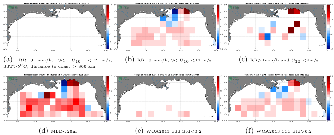
Figure 12: Temporal mean gridded over spatial boxes of size 1^{\circ}\times 1^{\circ} of \Delta\text{SSS} (SMAP-L3-RSS-V4-MONTHLY - Argo) for 6 different subdatasets corresponding to:RR=0 mm/h, 3 < U_{10} < 12 m/s, SST > 5^{\circ}\text{C} , distance to coast > 800 km (a), RR=0 mm/h, 3 < U_{10} < 12 m/s (b), RR > 1 mm/h and U_{10} < 4 m/s (c),MLD < 20\text{m} (d),WOA2013 SSS Std < 0.2 (e),WOA2013 SSS Std > 0.2 (f).
