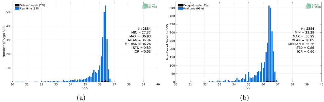
Figure 2: Histograms of SSS from Argo (a) and SMAP-L3-RSS-V4-MONTHLY (b) considering all match-up pairs per bins of 0.1 over the Mississippi river plume Pi-MEP region and for the full satellite product period.
