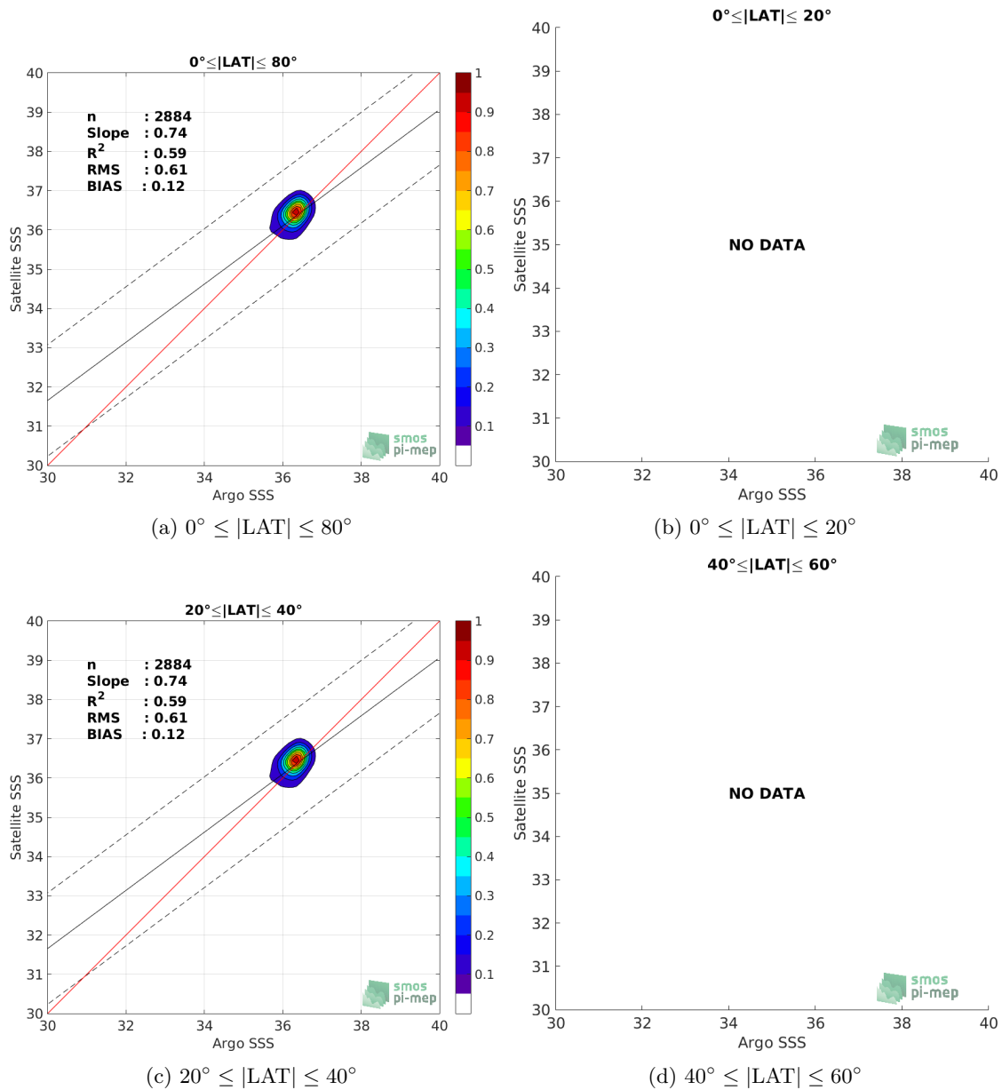
Figure 9: Contour maps of the concentration of SMAP-L3-RSS-V4-MONTHLY SSS (y-axis) versus Argo SSS (x-axis) at match-up pairs for different latitude bands. For each plot, the red line shows x=y . The black thin and dashed lines indicate a linear fit through the data cloud and the \pm 95\% confidence levels, respectively. The number match-up pairs n , the slope and R^2 coefficient of the linear fit, the root mean square (RMS) and the mean bias between satellite and in situ data are indicated for each latitude band in each plots.
