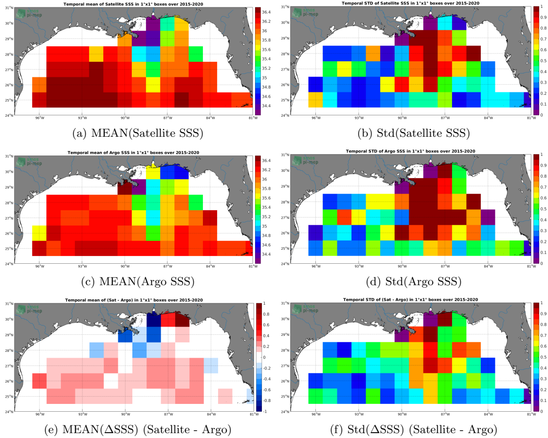
Figure 6: Temporal mean (left) and Std (right) of SSS from SMAP-L3-RSS-V4-MONTHLY (top), Argo (middle), and of \Delta SSS (Satellite - Argo). Only match-up pairs are used to generate these maps.
