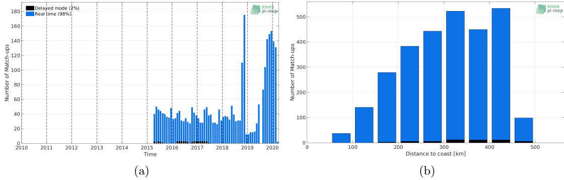
Figure 1: Number of match-ups between Argo and SMAP-L3-RSS-V4-MONTHLY SSS as a function of time (a) and as function of the distance to coast (b) over the Mississippi river plume Pi-MEP region and for the full satellite product period.
