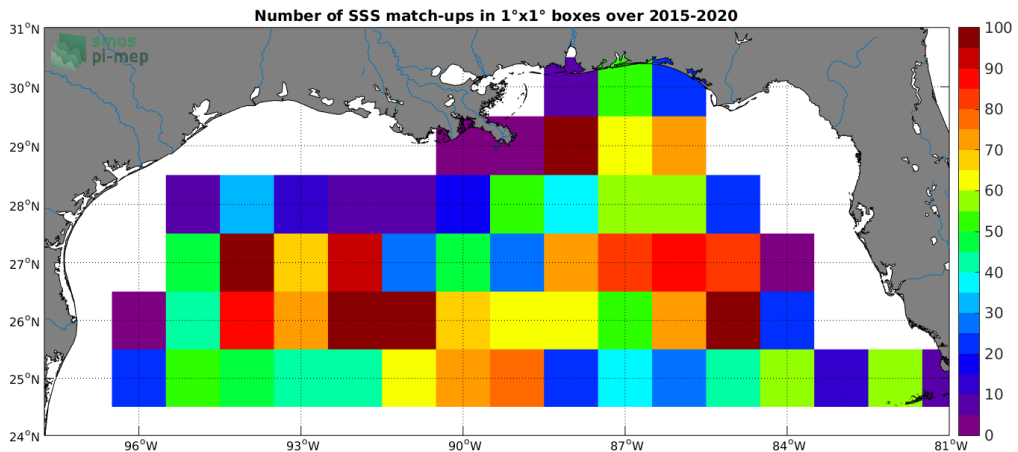
Figure 4: Number of SSS match-ups between Argo SSS and the SMAP-L3-RSS-V4-MONTHLY SSS product for the Mississippi river plume Pi-MEP region over 1^\circ \times 1^\circ boxes and for the full satellite product period.
