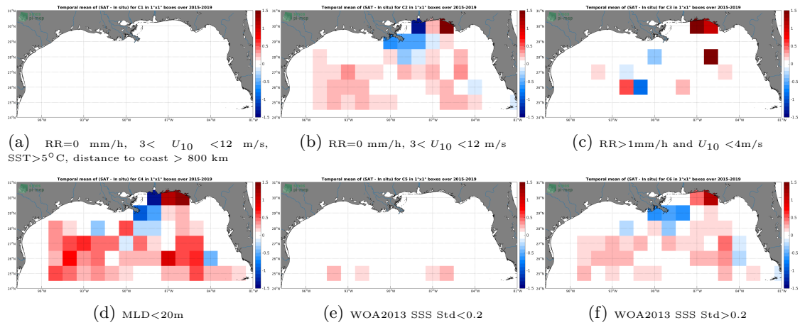
Figure 12: Temporal mean gridded over spatial boxes of size 1^\circ \times 1^\circ of \Delta SSS (SMAP-L3-RSS-V4-MONTHLY - Argo) for 6 different subdatasets corresponding to:RR=0 mm/h, 3 < U_{10} < 12 m/s, SST >5^\circ\text{C} , distance to coast > 800 km (a), RR=0 mm/h, 3 < U_{10} < 12 m/s (b), RR >1 mm/h and U_{10} < 4 m/s (c),MLD <20 m (d),WOA2013 SSS Std <0.2 (e),WOA2013 SSS Std >0.2 (f).
