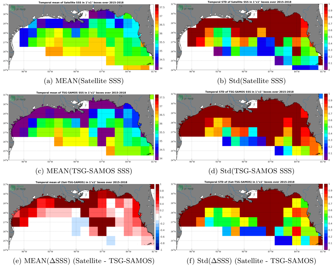
Figure 6: Temporal mean (left) and Std (right) of SSS from SMAP-L3-RSS-V3-MONTHLY-0.25DEG-40KM (top), TSG-SAMOS (middle), and of \Delta SSS (Satellite - TSG-SAMOS). Only match-up pairs are used to generate these maps.
