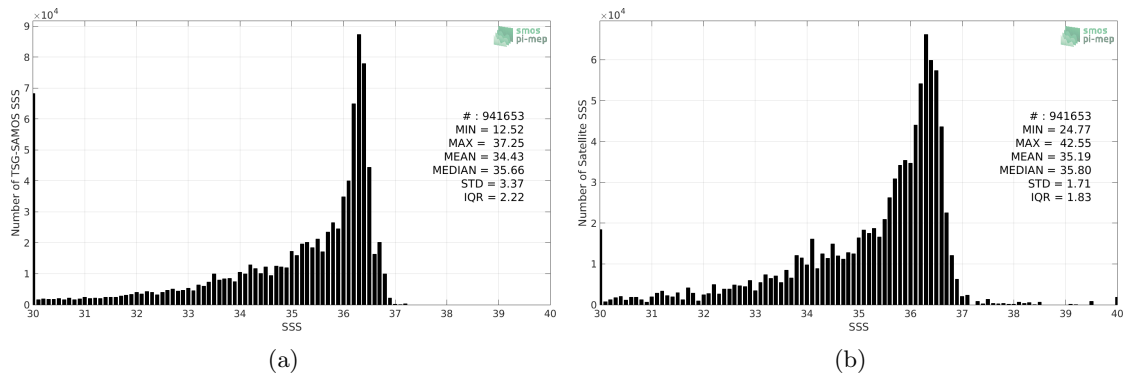
Figure 2: Histograms of SSS from TSG-SAMOS (a) and SMAP-L3-RSS-V3-MONTHLY-0.25DEG-40KM (b) considering all match-up pairs per bins of 0.1 over the Mississippi river plume Pi-MEP region and for the full satellite product period.
