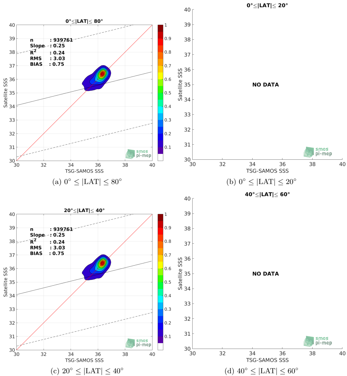
Figure 9: Contour maps of the concentration of SMAP-L3-RSS-V3-MONTHLY-0.25DEG-40KM SSS (y-axis) versus TSG-SAMOS SSS (x-axis) at match-up pairs for different latitude bands. For each plot, the red line shows x=y . The black thin and dashed lines indicate a linear fit through the data cloud and the \pm 95\% confidence levels, respectively. The number match-up pairs n , the slope and R^2 coefficient of the linear fit, the root mean square (RMS) and the mean bias between satellite and in situ data are indicated for each latitude band in each plots.
