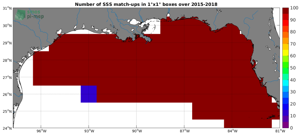
Figure 4: Number of SSS match-ups between TSG-SAMOS SSS and the SMAP-L3-RSS-V3-MONTHLY-0.25DEG-40KM SSS product for the Mississippi river plume Pi-MEP region over 1^\circ \times 1^\circ boxes and for the full satellite product period.
