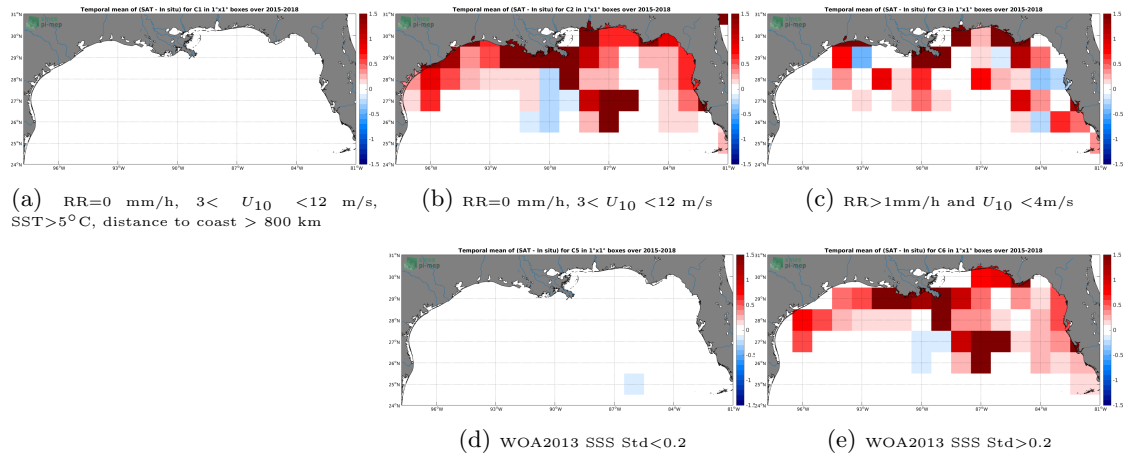
Figure 12: Temporal mean gridded over spatial boxes of size 1^\circ \times 1^\circ of \Delta SSS (SMAP-L3-RSS-V3-MONTHLY-0.25DEG-40KM - TSG-SAMOS) for 5 different subdatasets corresponding to:RR=0 mm/h, 3 < U_{10} < 12 m/s, SST >5^\circ C, distance to coast > 800 km (a), RR=0 mm/h, 3 < U_{10} < 12 m/s (b), RR >1 mm/h and U_{10} < 4 m/s (c), WOA2013 SSS Std <0.2 (d), WOA2013 SSS Std >0.2 (e).
