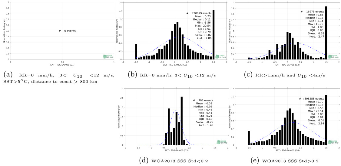
Figure 13: Normalized histogram of \Delta SSS (SMAP-L3-RSS-V3-MONTHLY-0.25DEG-40KM - TSG-SAMOS) for 5 different subdatasets corresponding to: RR=0 mm/h, 3 < U_{10} < 12 m/s, SST > 5°C, distance to coast > 800 km (a), RR=0 mm/h, 3 < U_{10} < 12 m/s (b), RR > 1mm/h and U_{10} < 4 m/s (c), WOA2013 SSS Std < 0.2 (d), WOA2013 SSS Std > 0.2 (e).
