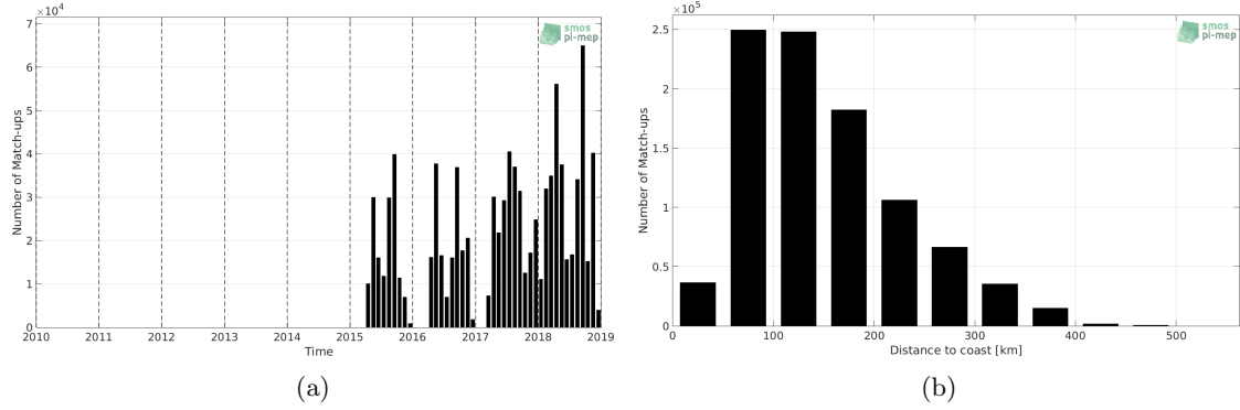
Figure 1: Number of match-ups between TSG-SAMOS and SMAP-L3-RSS-V3-MONTHLY-0.25DEG-40KM SSS as a function of time (a) and as function of the distance to coast (b) over the Mississippi river plume Pi-MEP region and for the full satellite product period.
