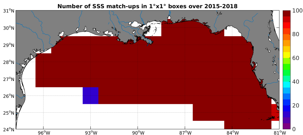
Figure 4: Number of SSS match-ups between TSG-SAMOS SSS and the SMAP-L3-RSS-V2-8DAY-RUNNING-70KM SSS product for the Mississippi river plume Pi-MEP region over 1^\circ \times 1^\circ boxes and for the full satellite product period.
