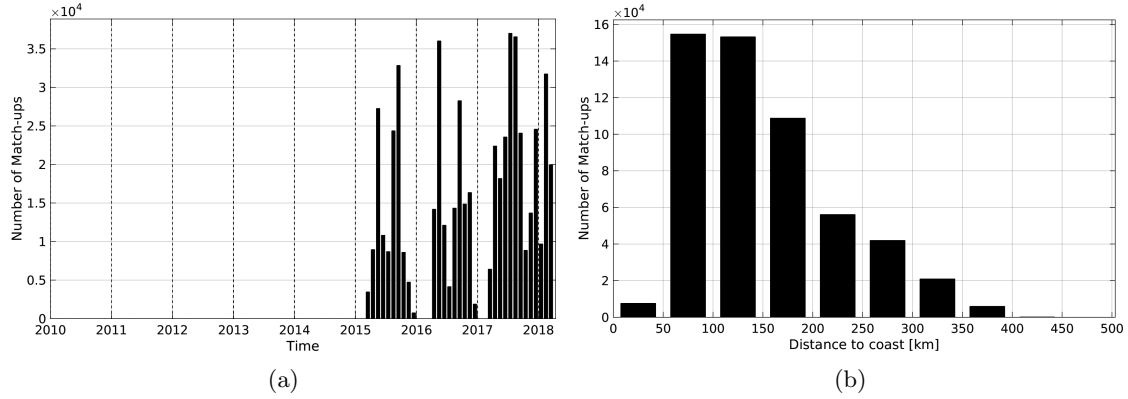
Figure 1: Number of match-ups between TSG-SAMOS and SMAP-L3-RSS-V2-8DAY-RUNNING-70KM SSS as a function of time (a) and as function of the distance to coast (b) over the Mississippi river plume Pi-MEP region and for the full satellite product period.
