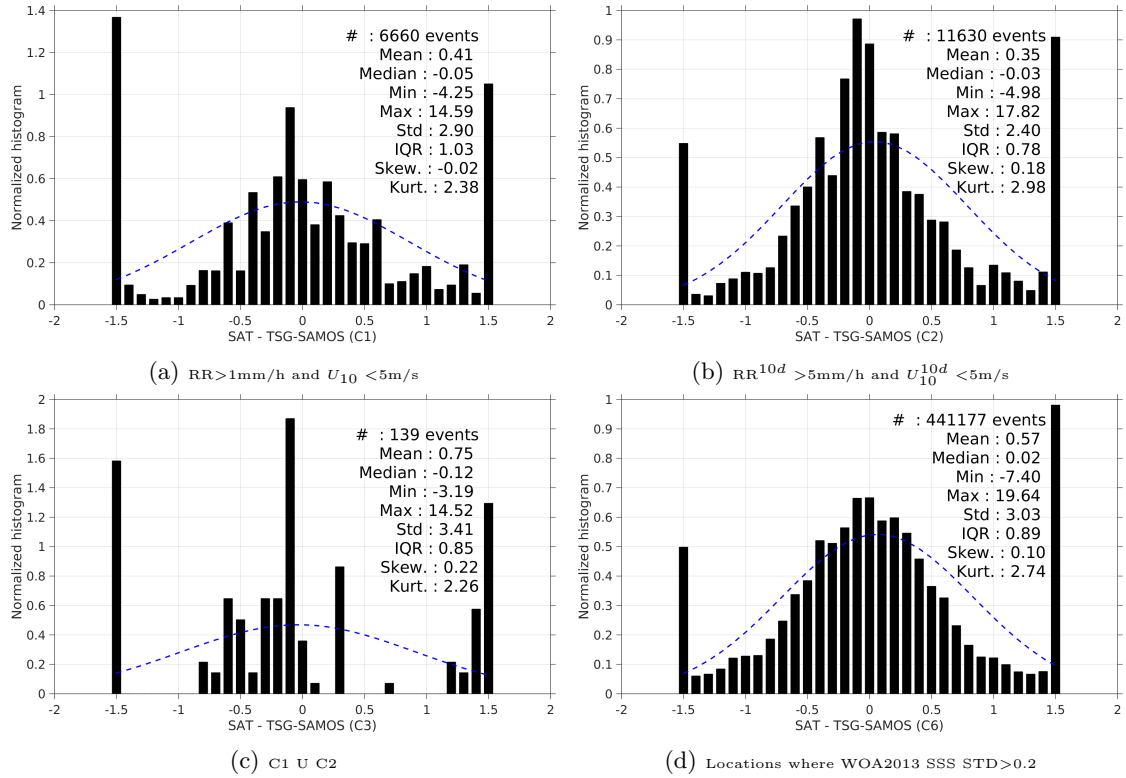
Figure 13: Normalized histogram of \Delta SSS (SMAP-L3-RSS-V2-8DAY-RUNNING-70KM - TSG-SAMOS) for 6 different subdatasets corresponding to: RR > 1mm/h and U_{10} < 5 m/s (a), RR^{10d} > 5 mm/h and U_{10}^{10d} < 5 m/s (b), C1 U C2 (c), Locations where WOA2013 SSS STD > 0.2 (d).
