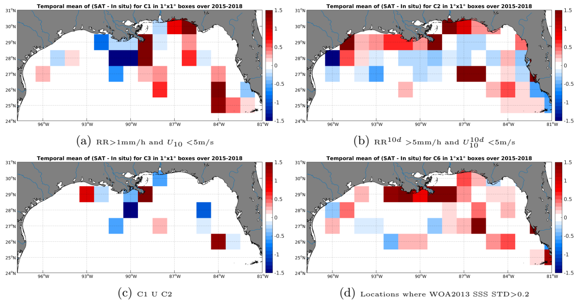
Figure 12: Temporal mean gridded over spatial boxes of size 1^\circ \times 1^\circ of \Delta SSS (SMAP-L3-RSS-V2-8DAY-RUNNING-70KM - TSG-SAMOS) for 4 different subdatasets corresponding to:RR >1 mm/h and U_{10} < 5 m/s (a), RR 10d > 5 mm/h and U_{10}^{10d} < 5 m/s (b), C1 U C2 (c),Locations where WOA2013 SSS STD >0.2 (d).
