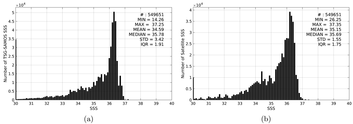
Figure 2: Histograms of SSS from TSG-SAMOS (a) and SMAP-L3-RSS-V2-8DAY-RUNNING-70KM (b) considering all match-up pairs per bins of 0.1 over the Mississippi river plume Pi-MEP region and for the full satellite product period.
