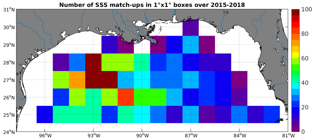
Figure 4: Number of SSS match-ups between Argo SSS and the SMAP-L3-RSS-V2-8DAY-RUNNING-70KM SSS product for the Mississippi river plume Pi-MEP region over 1^\circ \times 1^\circ boxes and for the full satellite product period.
