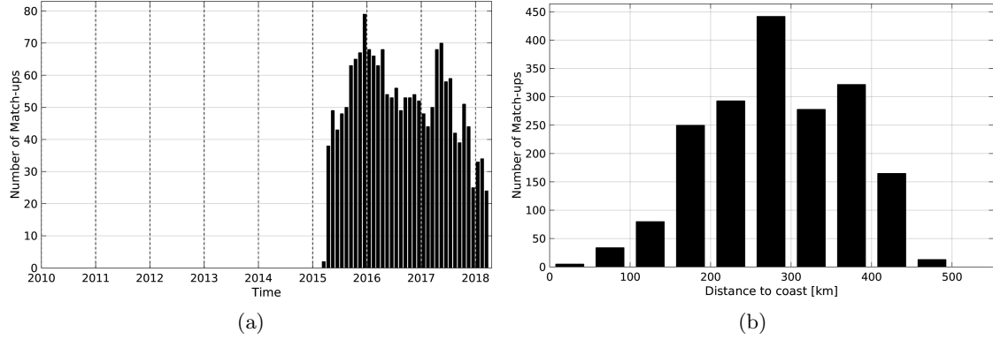
Figure 1: Number of match-ups between Argo and SMAP-L3-RSS-V2-8DAY-RUNNING-70KM SSS as a function of time (a) and as function of the distance to coast (b) over the Mississippi river plume Pi-MEP region and for the full satellite product period.
