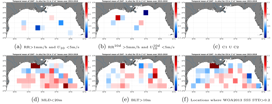
Figure 12: Temporal mean gridded over spatial boxes of size 1^\circ \times 1^\circ of \Delta SSS (SMAP-L3-RSS-V2-8DAY-RUNNING-70KM - Argo) for 6 different subdatasets corresponding to: RR > 1\text{mm/h} and U_{10} < 5\text{m/s} (a), RR^{10d} > 5\text{mm/h} and U_{10}^{10d} < 5\text{m/s} (b), C1 U C2 (c), MLD < 20\text{m} (d), BLT > 10\text{m} (e), Locations where WOA2013 SSS STD > 0.2 (f).
