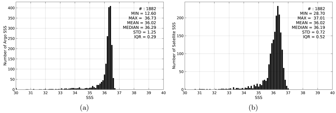
Figure 2: Histograms of SSS from Argo (a) and SMAP-L3-RSS-V2-8DAY-RUNNING-70KM (b) considering all match-up pairs per bins of 0.1 over the Mississippi river plume Pi-MEP region and for the full satellite product period.
